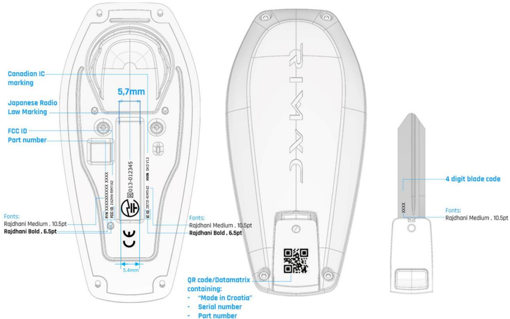
Lower housing (B surfaces below PCB)
