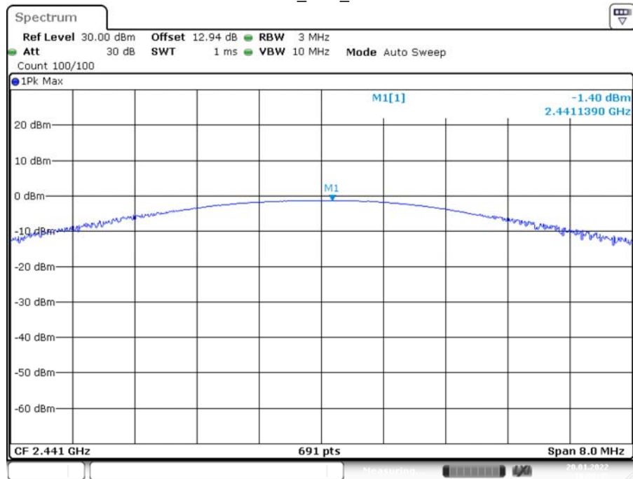
2DH1_Ant1_2441
