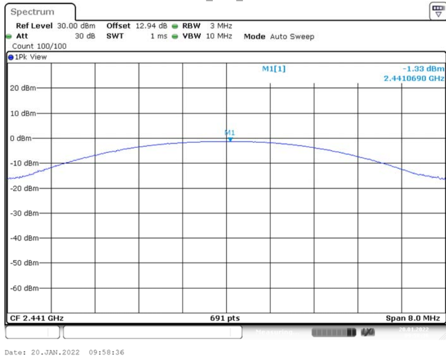
DH1_Ant1_2441
