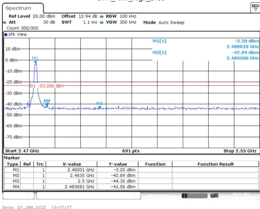
DH1_Ant1_High_2480
