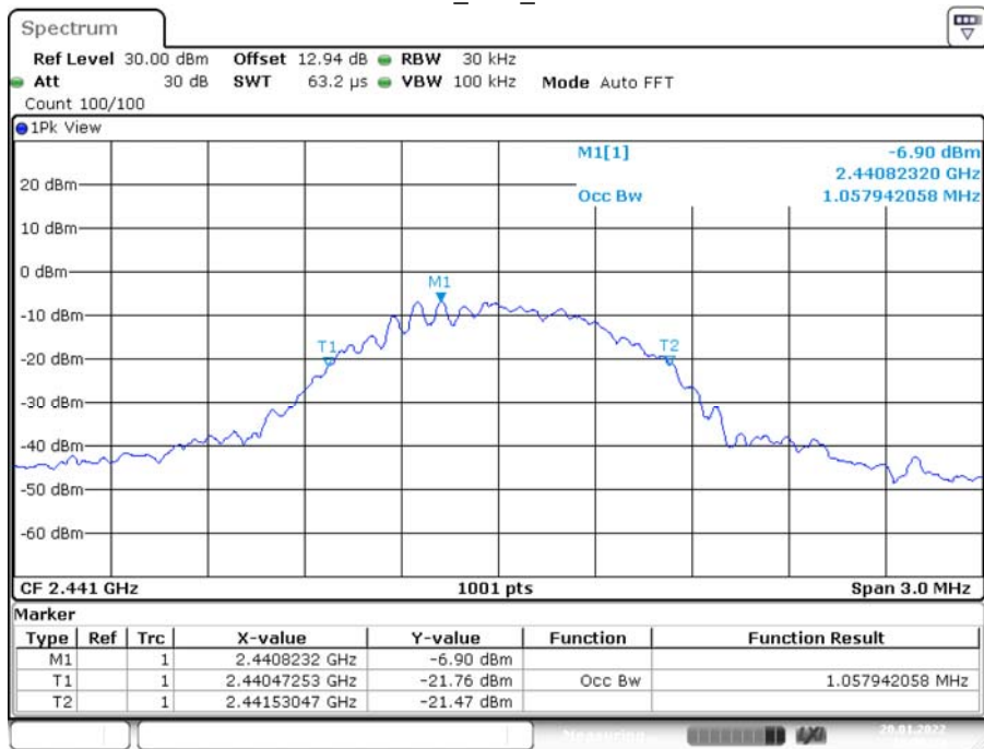
DH1_Ant1_2441
