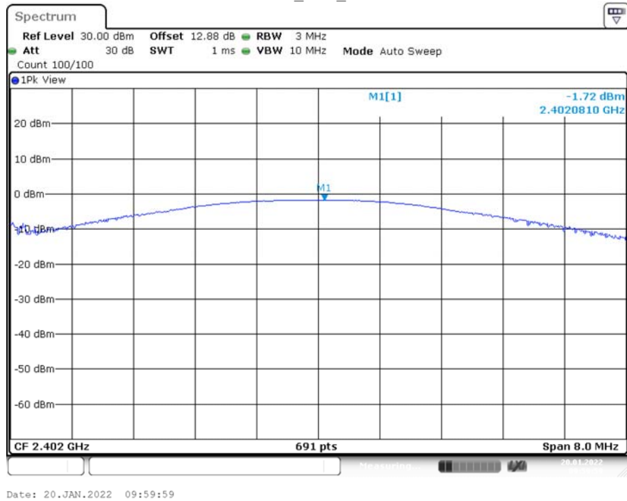
2DH1_Ant1_2402
