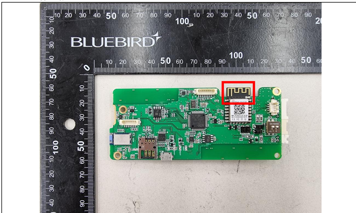
WIFI Antenna
