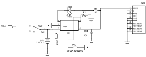
Charging Circuit
