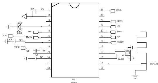
Y-2219 schematic diagram
