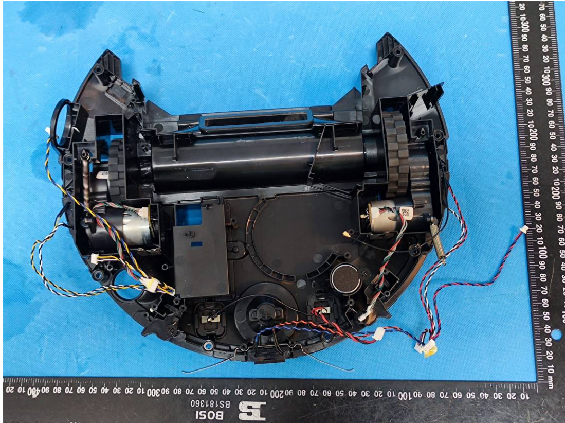
Buletooth&Wifi Antenna
