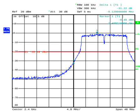
n20_2412MHz_Chain 0
