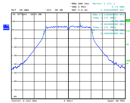
g_2412MHz_Chain 0
