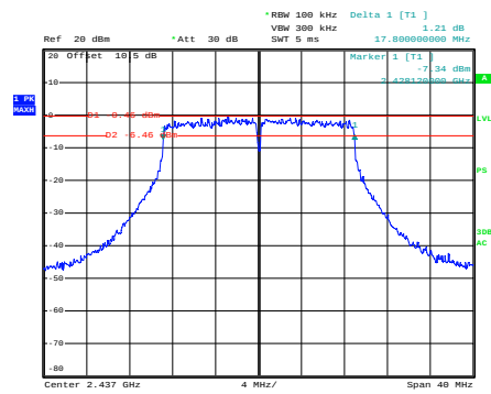
n20_2437MHz_Chain 0
