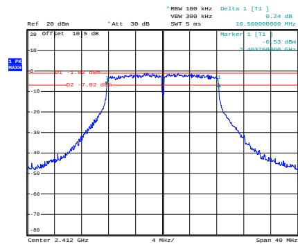
g_2412MHz_Chain 0
