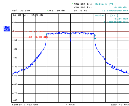
g_2462MHz_Chain 0
