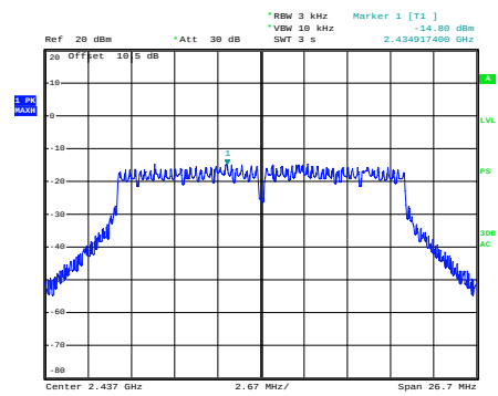
n20_2437MHz_Chain 0
