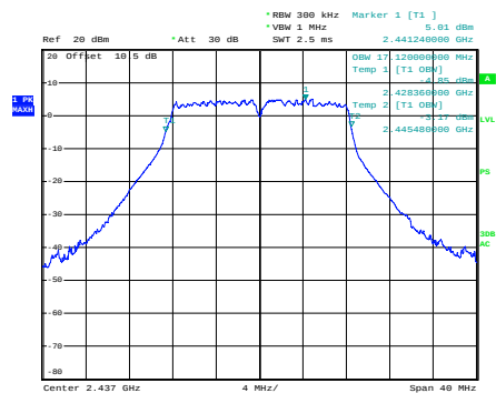
g_2437MHz_Chain 0
