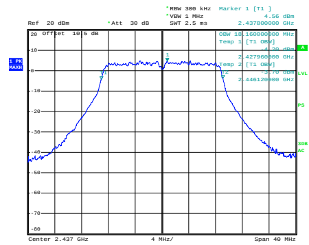
n20_2437MHz_Chain 0
