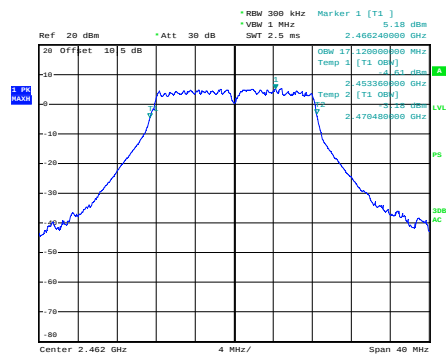
g_2462MHz_Chain 0
