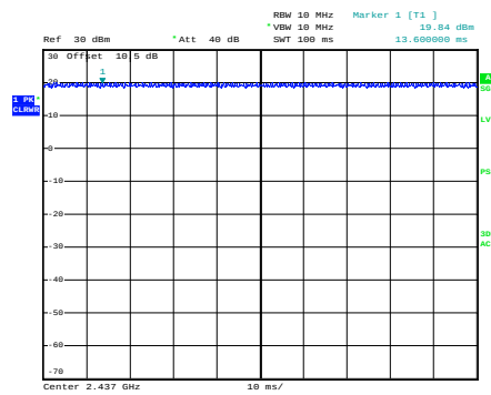
g_2437MHz_Chain 0
