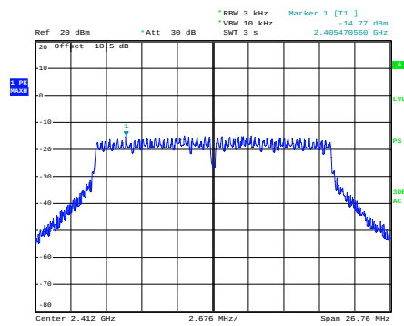
n20_2412MHz_Chain 0
