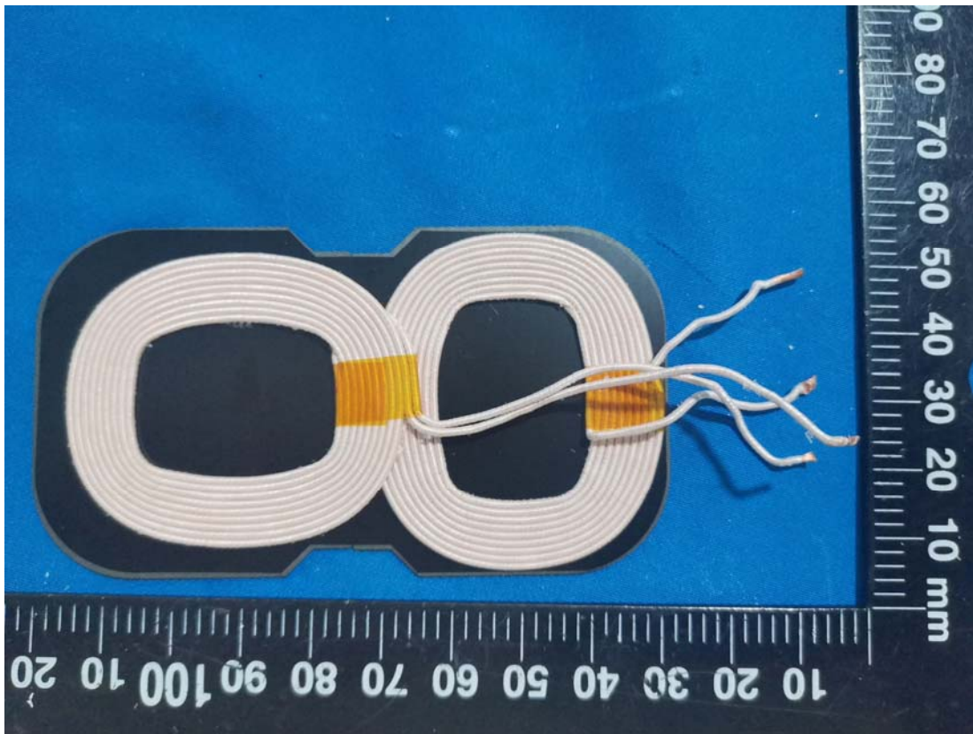
Coil Antenna
