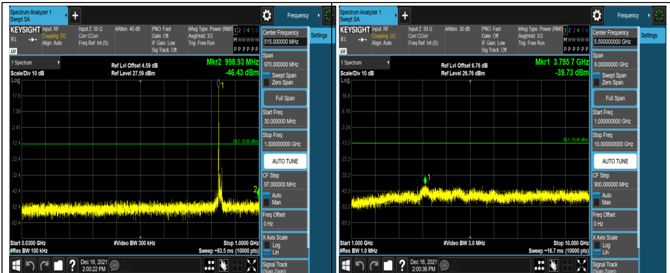
Band26-15MHz-16QAM-26865-1RB#0-Range1:30~1000MHz
