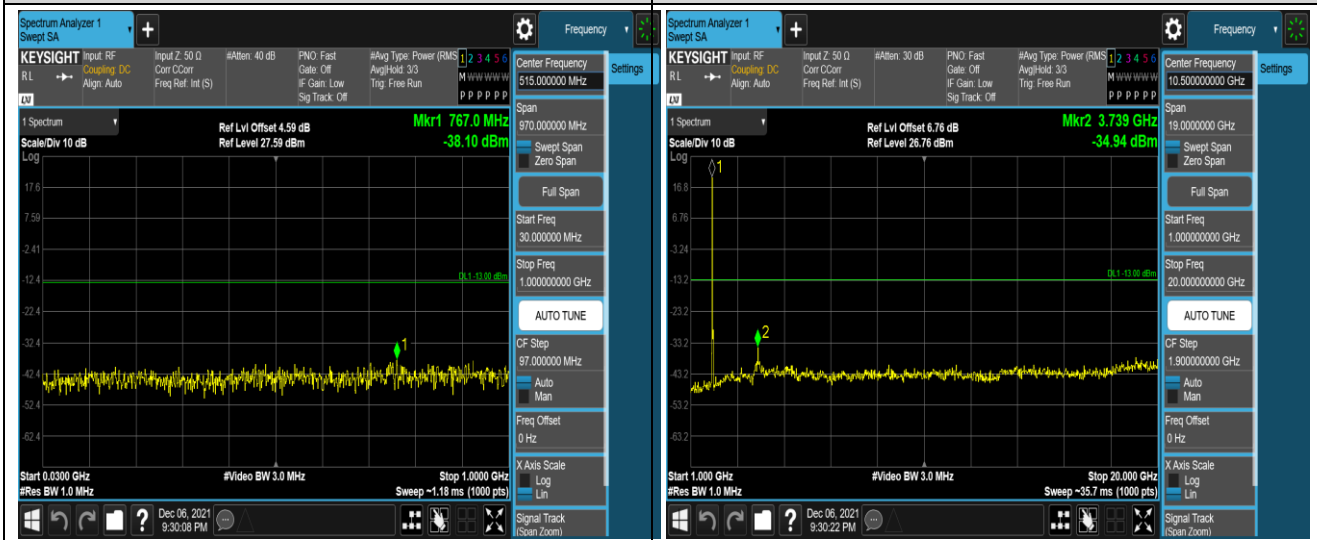
Band25-20MHz-16QAM-26365-1RB#0-Range1:30~1000MHz
