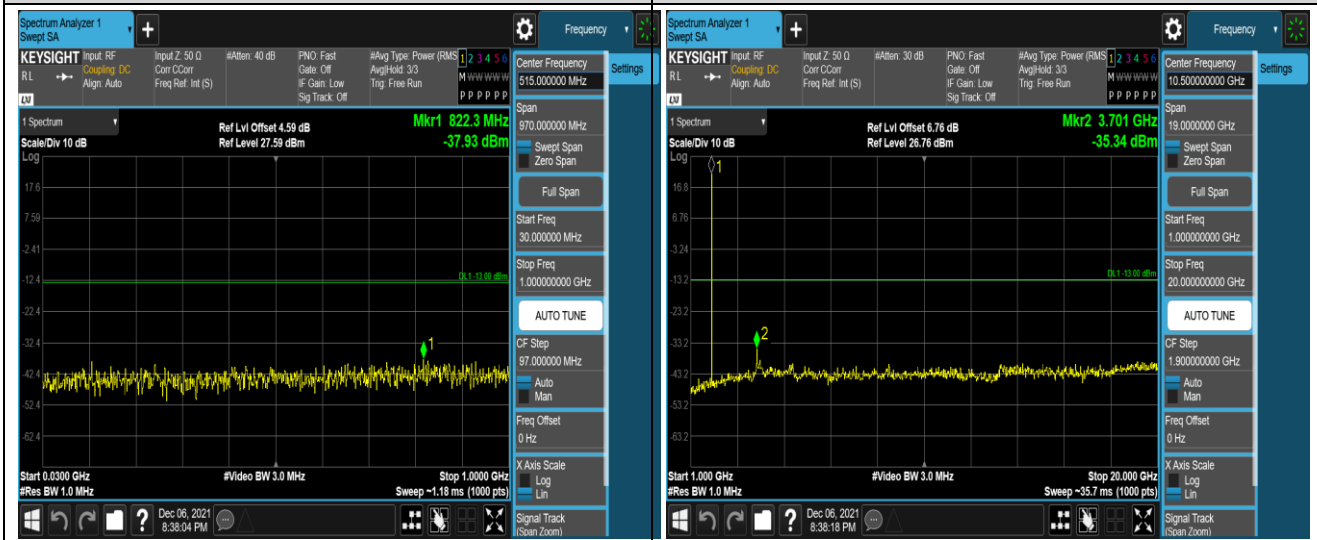
Band25-1.4MHz-QPSK-26047-1RB#0-Range1:30~1000MHz
