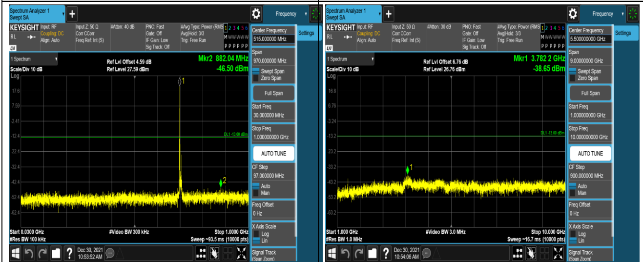
Band25-1.4MHz-QPSK-26047-1RB#0-Range1:30~1000MHz
