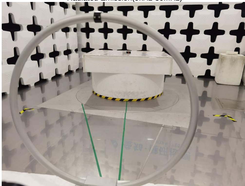
Radiated Emission(9kHz-30MHz)
