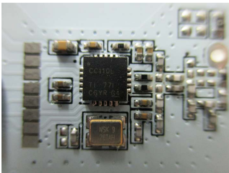
Closer view of the RF model
