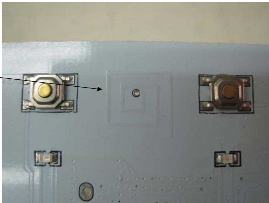
Rear closer view of the PCB antenna
