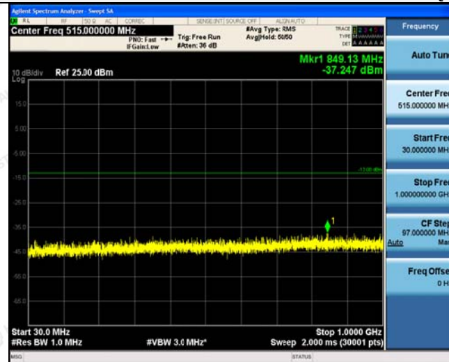
30MHz~1GHz
