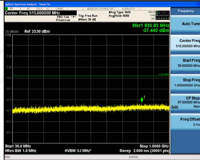
30MHz~1GHz
