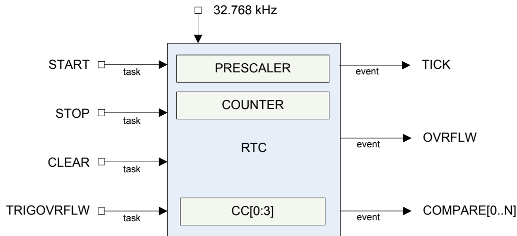
Figure 43: RTC block schematic
