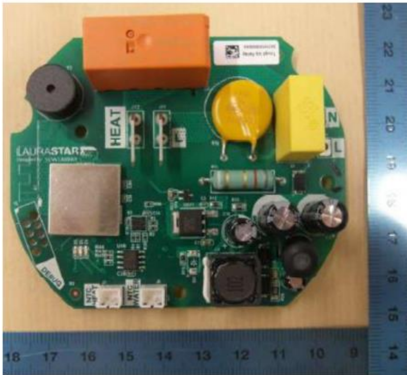
PCB top side
