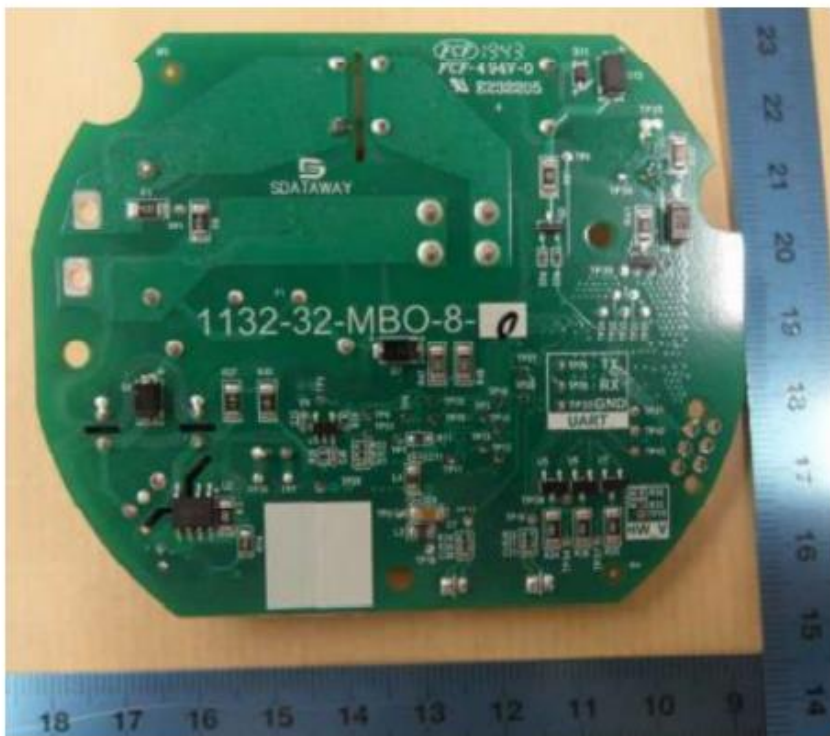
PCB bottom side
