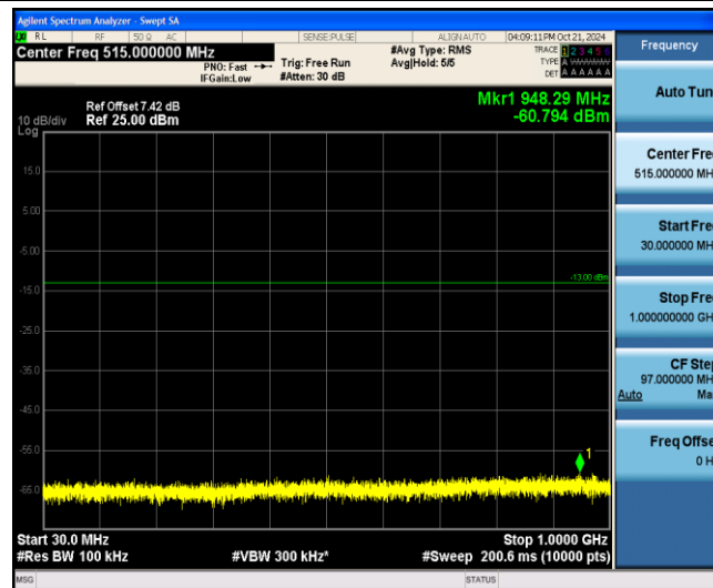
Band2-20MHz-16QAM-19100-1-0-Low-30-1000--60.79-PASS
