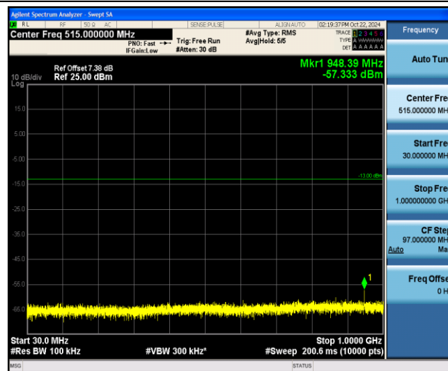
Band4-10MHz-QPSK-20175-1-0-Low-30-1000--57.33-PASS
