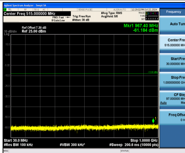
Band4-1.4MHz-16QAM-20393-1-0-Low-30-1000--61.18-PASS
