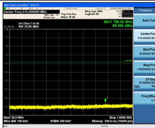
Band4-5MHz-16QAM-20175-1-0-Low-30-1000--60.06-PASS
