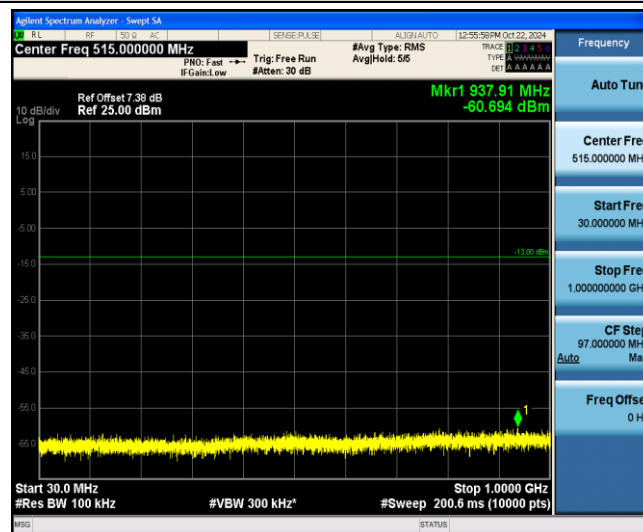
Band4-3MHz-16QAM-20175-1-0-Low-30-1000--60.69-PASS
