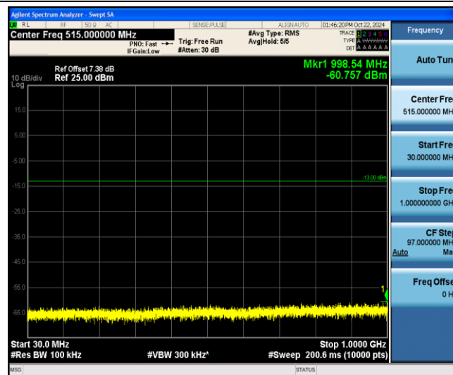
Band4-5MHz-QPSK-20175-1-0-Low-30-1000--60.76-PASS
