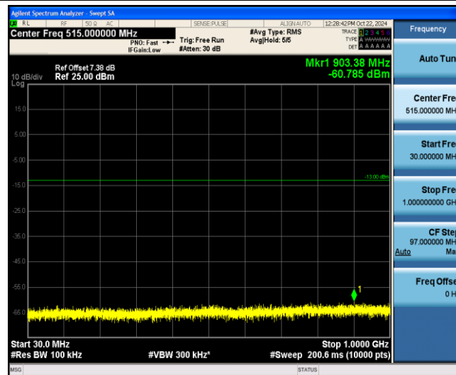
Band4-1.4MHz-QPSK-20393-1-0-Low-30-1000--60.79-PASS
