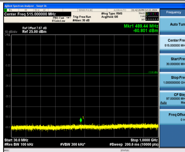
Band4-5MHz-QPSK-19975-1-0-Low-30-1000--60.8-PASS
