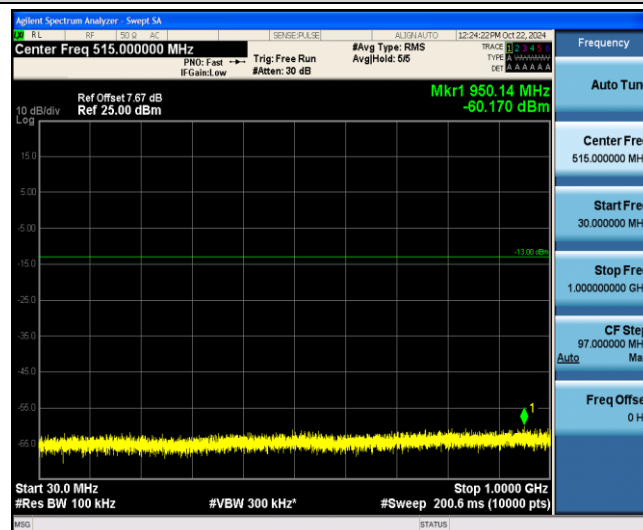
Band4-1.4MHz-16QAM-19957-1-0-Low-30-1000--60.17-PASS
