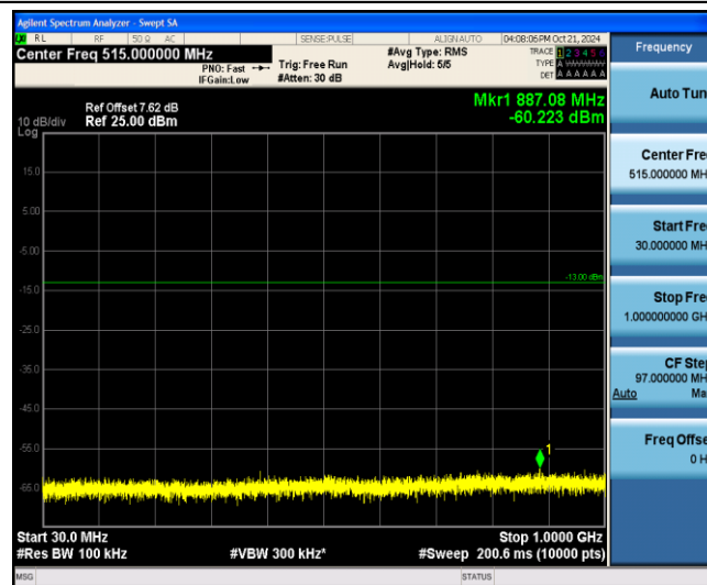
Band2-20MHz-16QAM-18900-1-0-Low-30-1000--60.22-PASS
