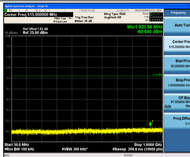
Band2-20MHz-16QAM-18700-1-0-Low-30-1000--60.64-PASS
