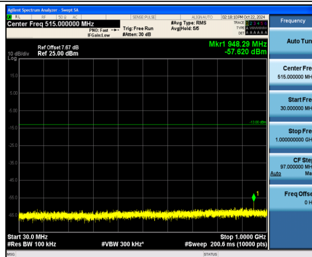
Band4-10MHz-16QAM-20000-1-0-Low-30-1000--57.62-PASS
