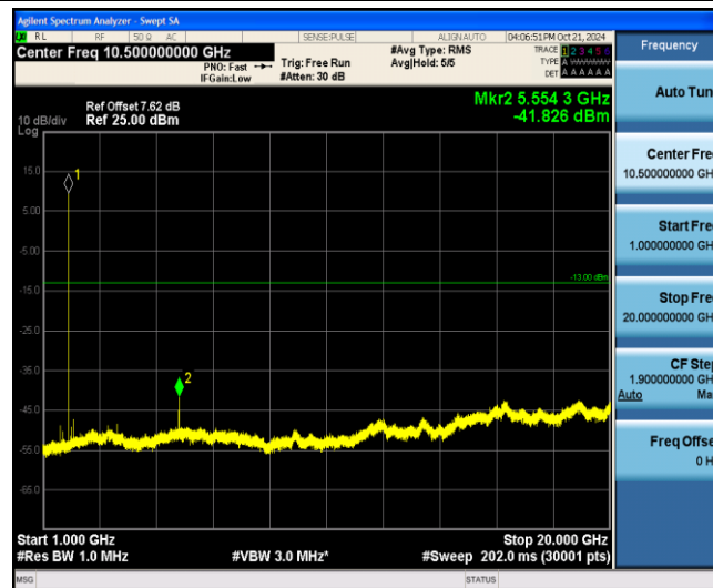
Band2-20MHz-QPSK-18700-1-0-Low-1000-20000--41.83-PASS
