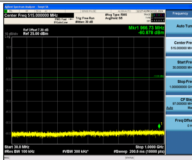
Band4-1.4MHz-16QAM-20175-1-0-Low-30-1000--60.88-PASS
