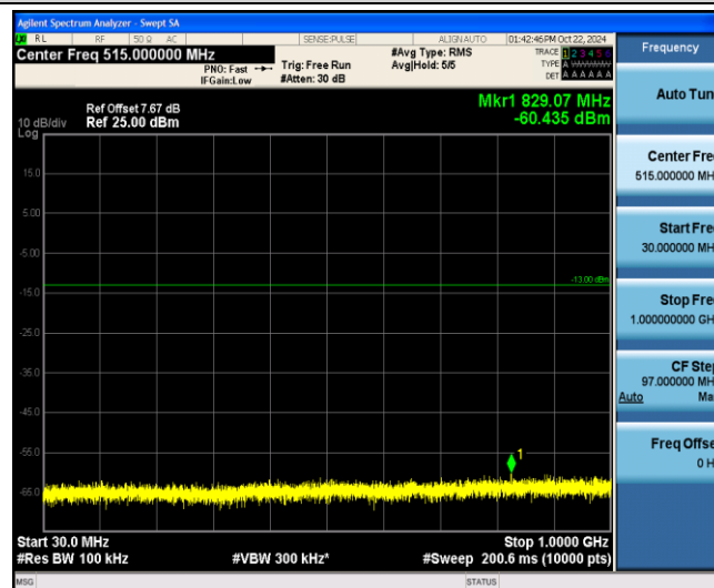
Band4-5MHz-16QAM-19975-1-0-Low-30-1000--60.44-PASS
