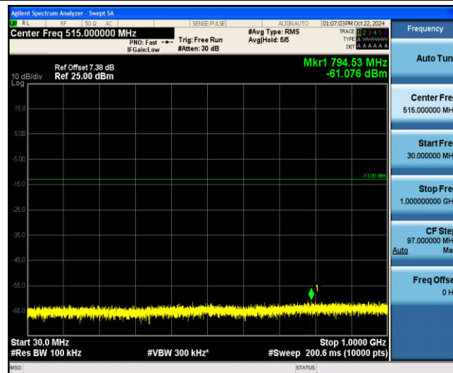
Band4-3MHz-QPSK-20385-1-0-Low-30-1000--61.08-PASS
