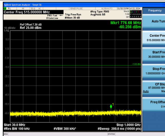
Band4-5MHz-16QAM-20375-1-0-Low-30-1000--60.26-PASS
