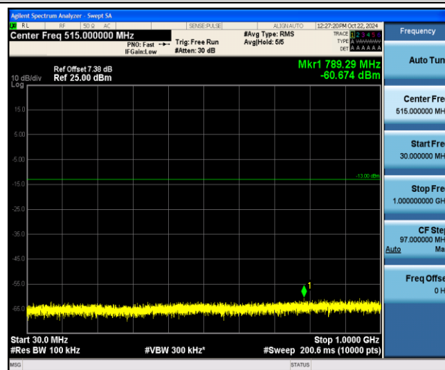
Band4-1.4MHz-QPSK-20175-1-0-Low-30-1000--60.67-PASS
