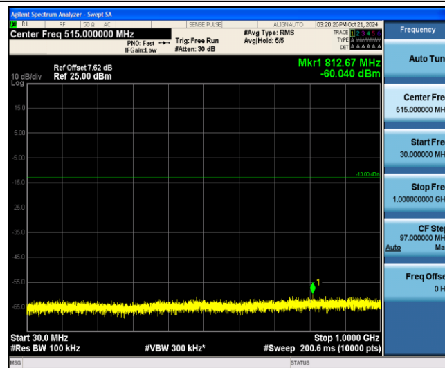
Band2-15MHz-QPSK-18900-1-0-Low-30-1000--60.04-PASS
