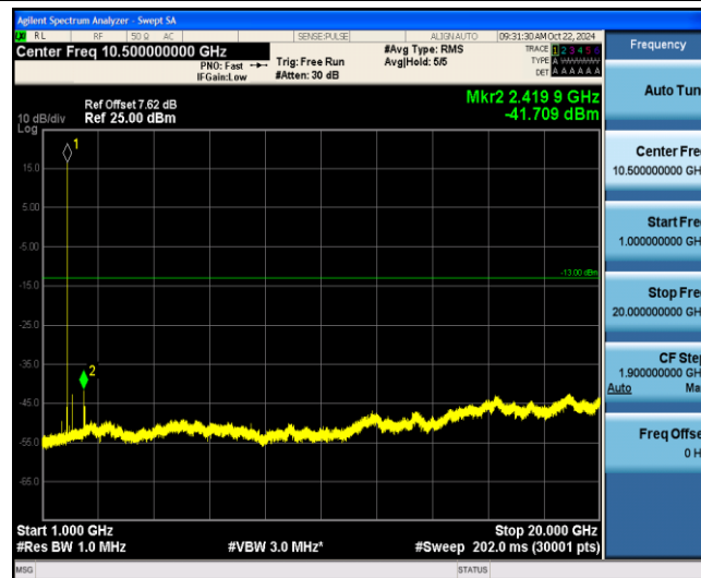
Band2-3MHz-QPSK-18615-1-0-Low-1000-20000--41.71-PASS
