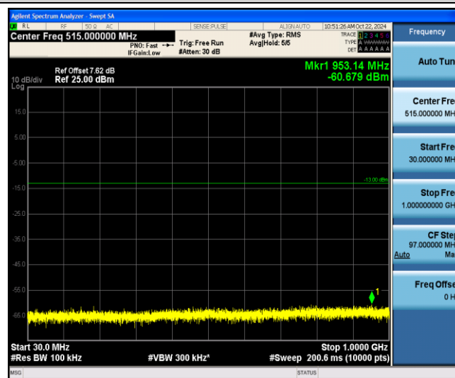
Band2-10MHz-16QAM-18900-1-0-Low-30-1000--60.68-PASS
