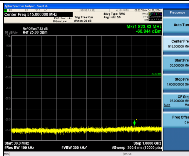
Band2-3MHz-16QAM-18900-1-0-Low-30-1000--60.84-PASS
