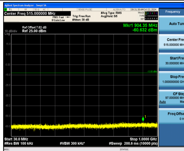
Band2-3MHz-16QAM-18615-1-0-Low-30-1000--60.63-PASS
