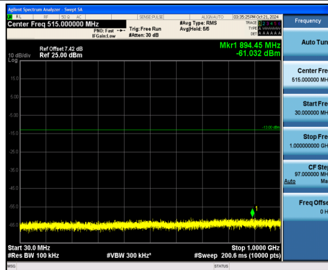
Band2-15MHz-16QAM-19125-1-0-Low-30-1000--61.03-PASS
