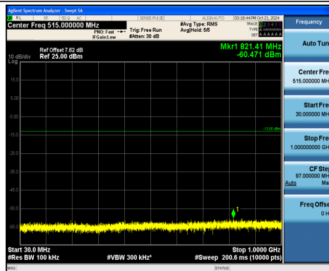
Band2-15MHz-QPSK-18675-1-0-Low-30-1000--60.47-PASS
