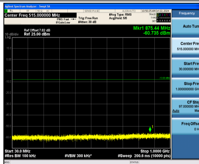
Band2-10MHz-16QAM-18650-1-0-Low-30-1000--60.74-PASS
