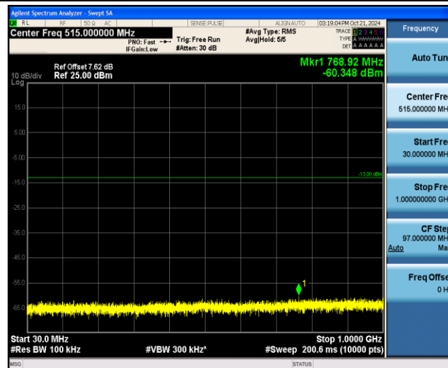
Band2-15MHz-16QAM-18675-1-0-Low-30-1000--60.35-PASS
