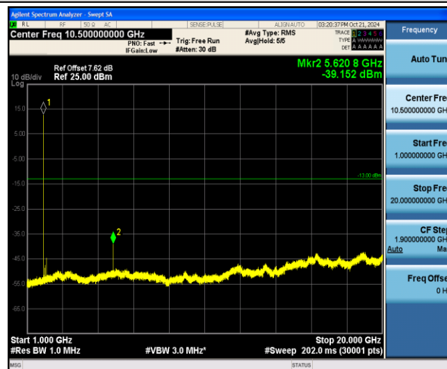
Band2-15MHz-QPSK-18900-1-0-Low-1000-20000--39.15-PASS
