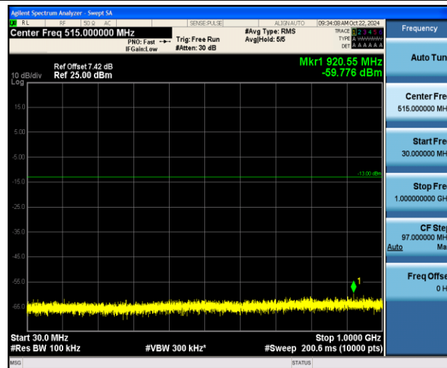
Band2-3MHz-16QAM-19185-1-0-Low-30-1000--59.78-PASS
