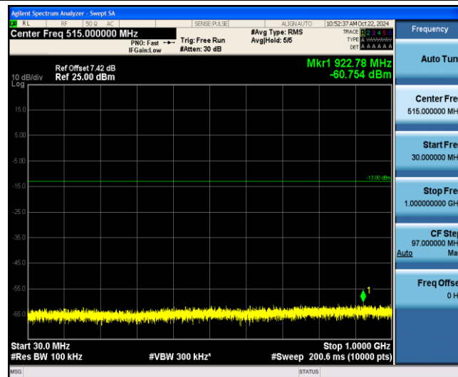
Band2-10MHz-16QAM-19150-1-0-Low-30-1000--60.75-PASS
