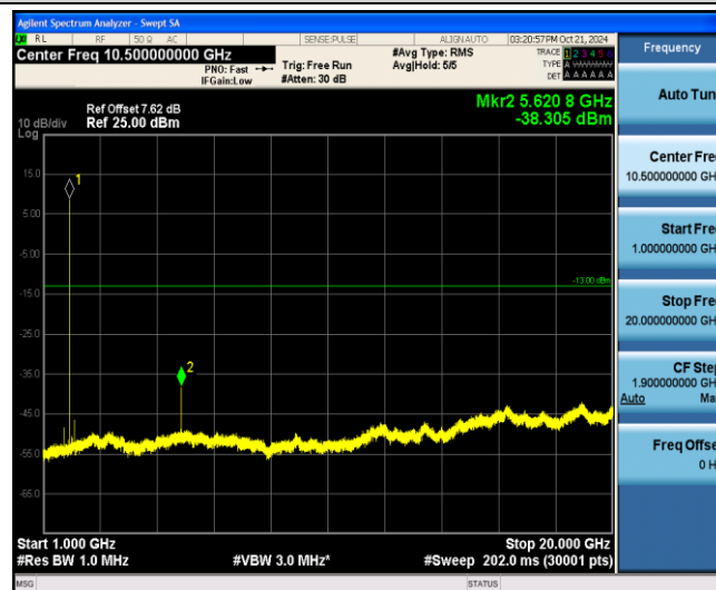
Band2-15MHz-16QAM-18900-1-0-Low-1000-20000--38.31-PASS
