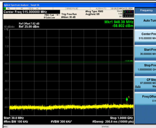
Band2-5MHz-16QAM-18625-1-0-Low-30-1000--58.8-PASS
