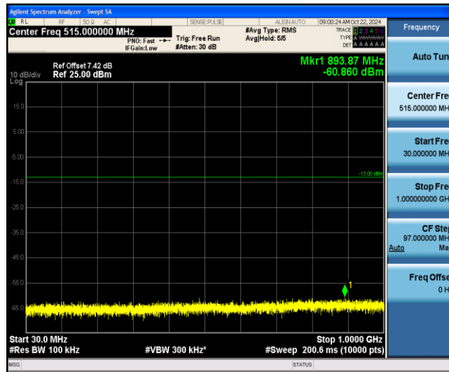
Band2-1.4MHz-16QAM-19193-1-0-Low-30-1000--60.86-PASS
