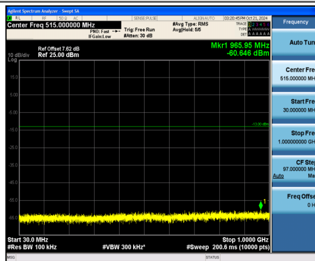
Band2-15MHz-16QAM-18900-1-0-Low-30-1000--60.65-PASS
