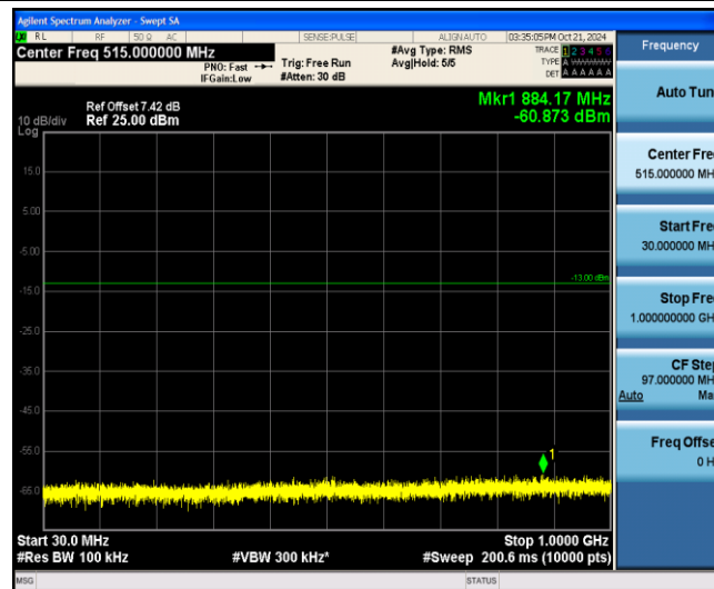
Band2-15MHz-QPSK-19125-1-0-Low-30-1000--60.87-PASS
