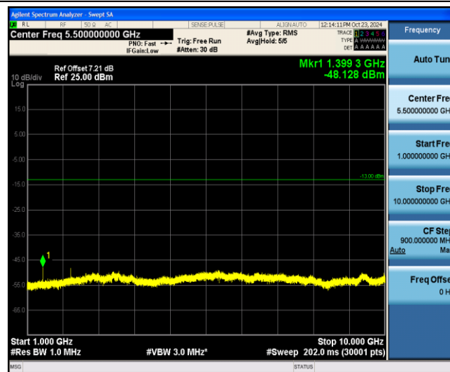
Band12-10MHz-QPSK-23060-1-0-Low-1000-10000--48.13-PASS
