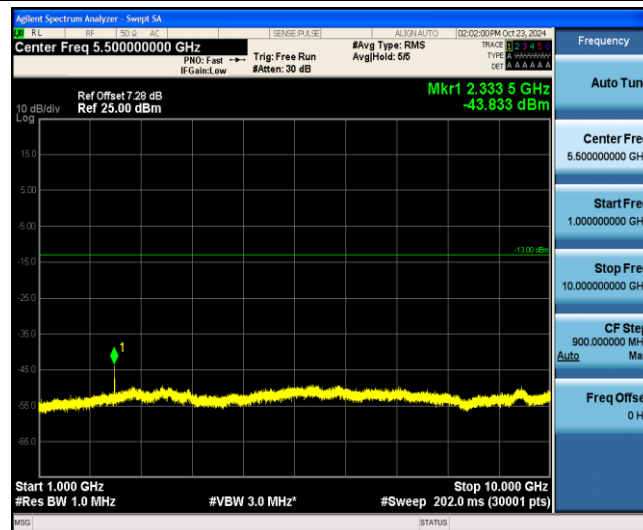
Band13-10MHz-QPSK-23230-1-0-Low-1000-10000--43.83-PASS
