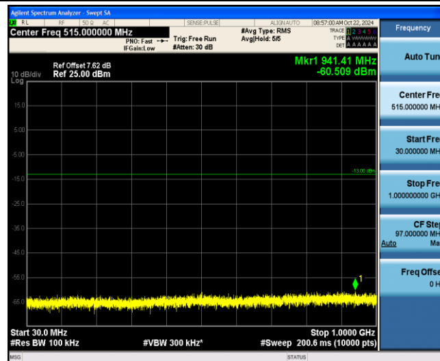
Band2-1.4MHz-16QAM-18607-1-0-Low-30-1000--60.51-PASS
