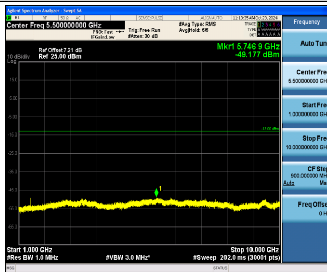
Band12-5MHz-QPSK-23035-1-0-Low-1000-10000--49.18-PASS
