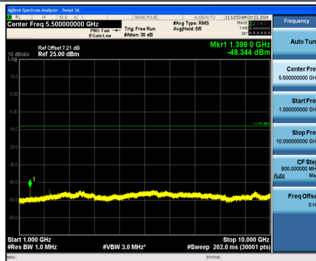
Band12-5MHz-16QAM-23035-1-0-Low-1000-10000--48.34-PASS
