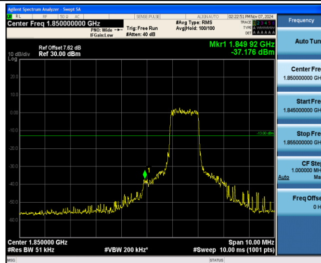
Band25-15MHz-QPSK-26115-6-0-Low--37.18-PASS
