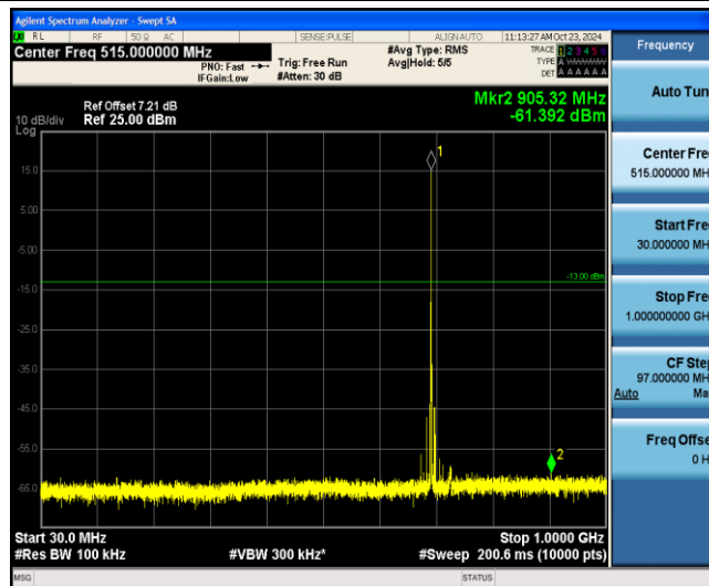
Band12-5MHz-QPSK-23035-1-0-Low-30-1000--61.39-PASS
