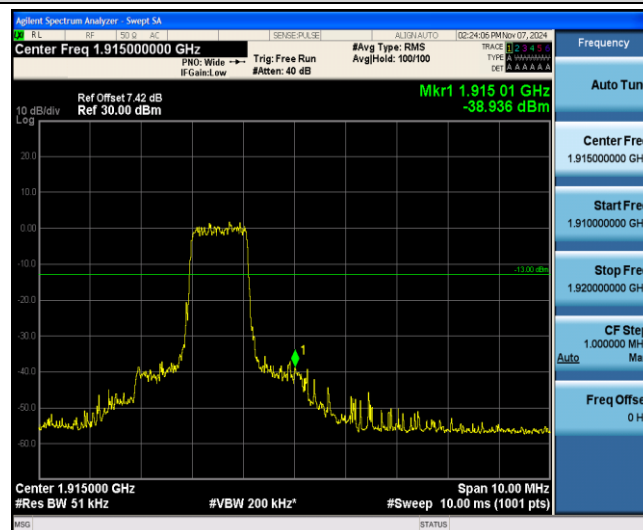
Band25-15MHz-16QAM-26615-6-0-High--38.94-PASS
