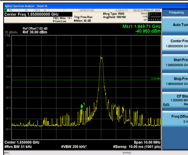
Band25-15MHz-QPSK-26115-1-0-Low--40.96-PASS
