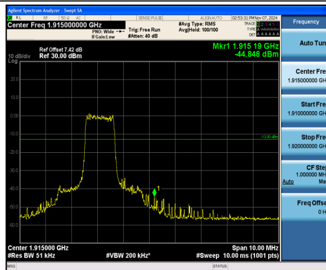
Band25-20MHz-16QAM-26590-6-0-High--44.85-PASS
