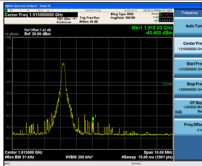
Band25-20MHz-16QAM-26590-1-5-High--45.40-PASS
