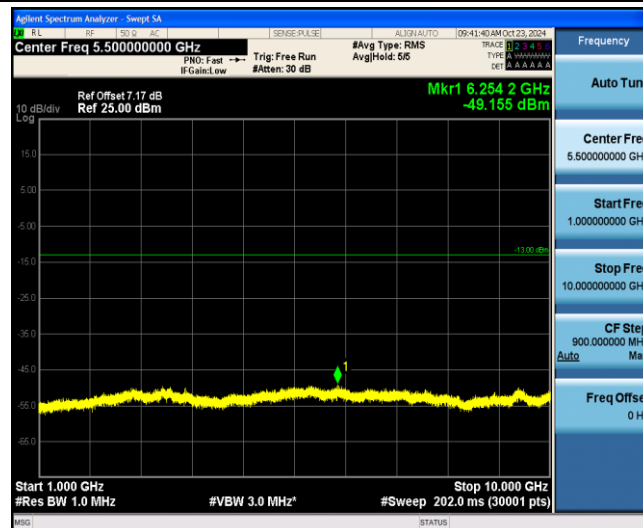
Band12-1.4MHz-QPSK-23173-1-0-Low-1000-10000--49.16-PASS
