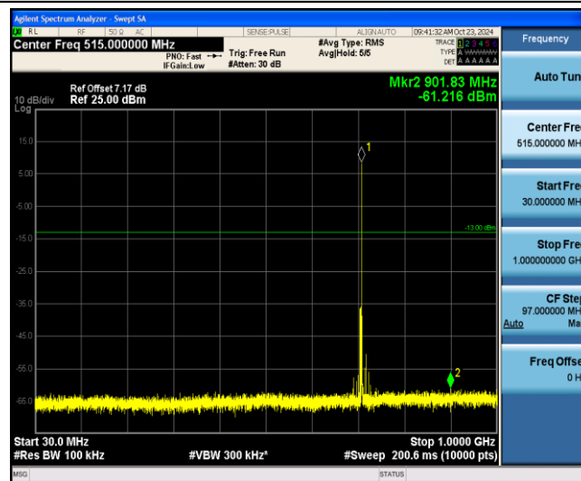
Band12-1.4MHz-QPSK-23173-1-0-Low-30-1000--61.22-PASS
