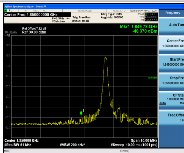
Band25-20MHz-16QAM-26140-1-0-Low--48.38-PASS
