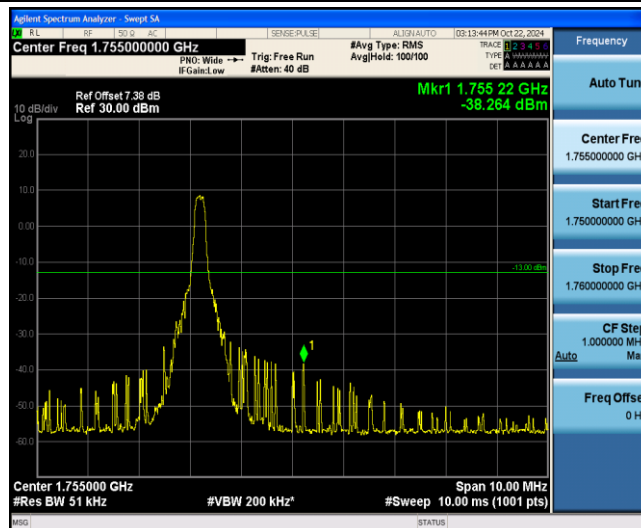
Band4-20MHz-QPSK-20300-1-5-High--38.26-PASS
