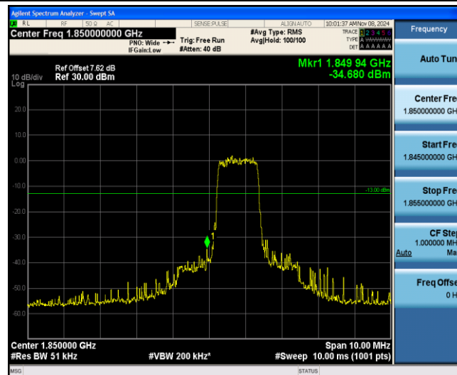
Band25-5MHz-16QAM-26065-6-0-Low--34.68-PASS
