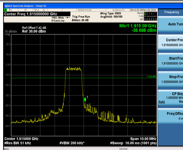
Band25-1.4MHz-QPSK-26683-6-0-High--36.70-PASS
