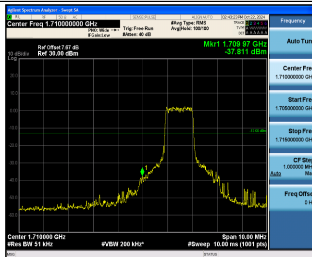
Band4-15MHz-QPSK-20025-6-0-Low--37.81-PASS
