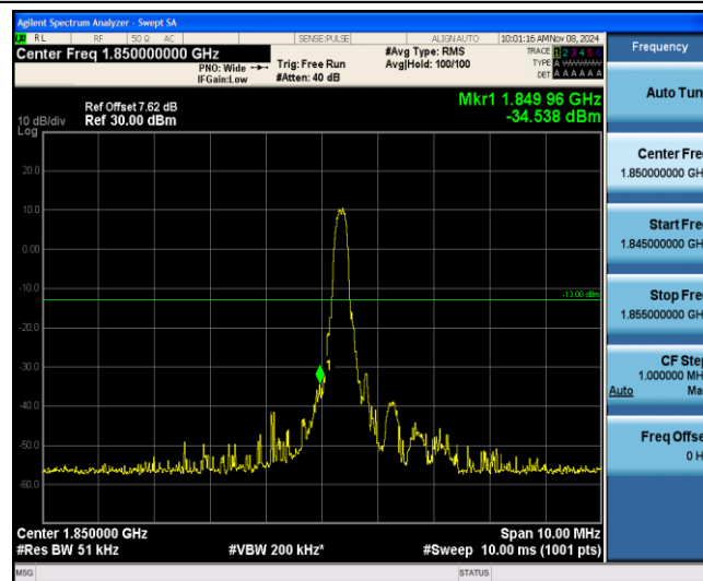
Band25-5MHz-16QAM-26065-1-0-Low--34.54-PASS
