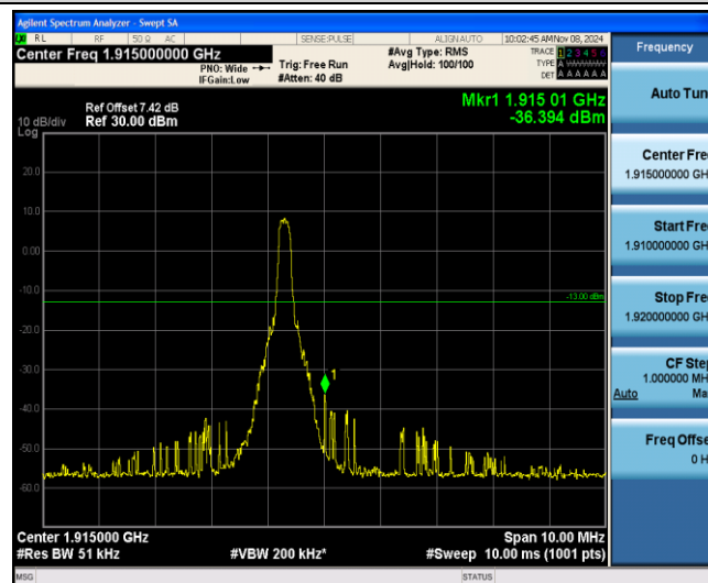
Band25-5MHz-QPSK-26665-1-5-High--36.39-PASS
