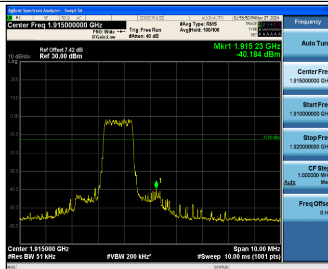
Band25-10MHz-QPSK-26640-6-0-High--40.18-PASS
