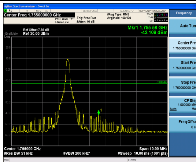
Band4-15MHz-16QAM-20325-1-5-High--42.11-PASS
