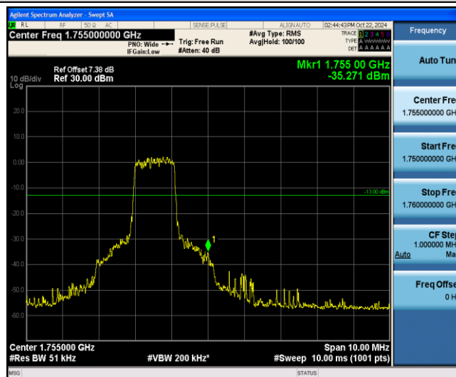
Band4-15MHz-16QAM-20325-6-0-High--35.27-PASS
