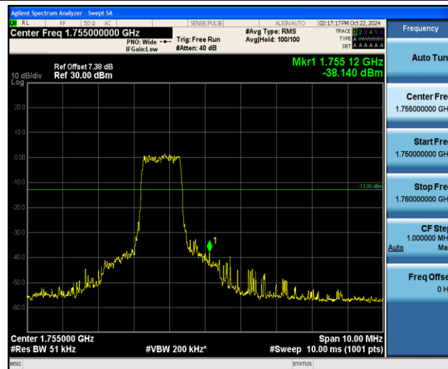
Band4-10MHz-16QAM-20350-6-0-High--38.14-PASS
