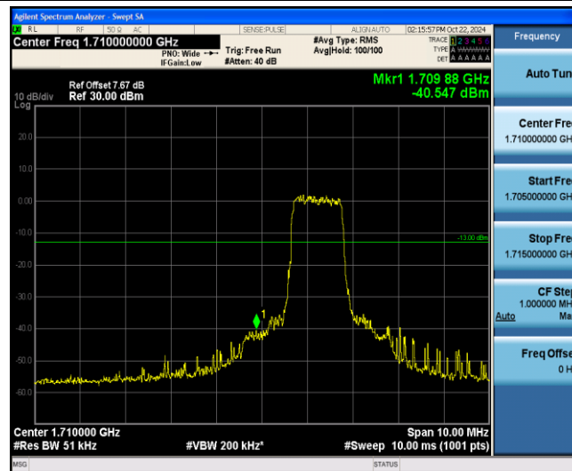
Band4-10MHz-QPSK-20000-6-0-Low--40.55-PASS
