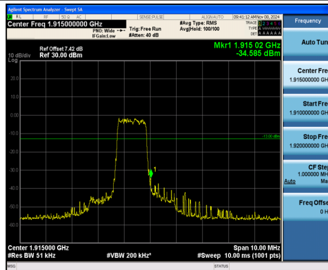
Band25-1.4MHz-16QAM-26683-6-0-High--34.58-PASS
