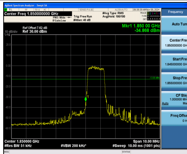
Band25-1.4MHz-QPSK-26047-6-0-Low--34.87-PASS
