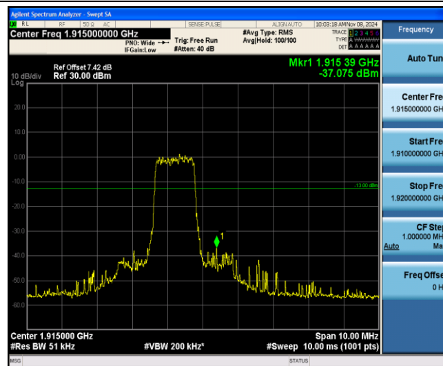
Band25-5MHz-16QAM-26665-6-0-High--37.08-PASS
