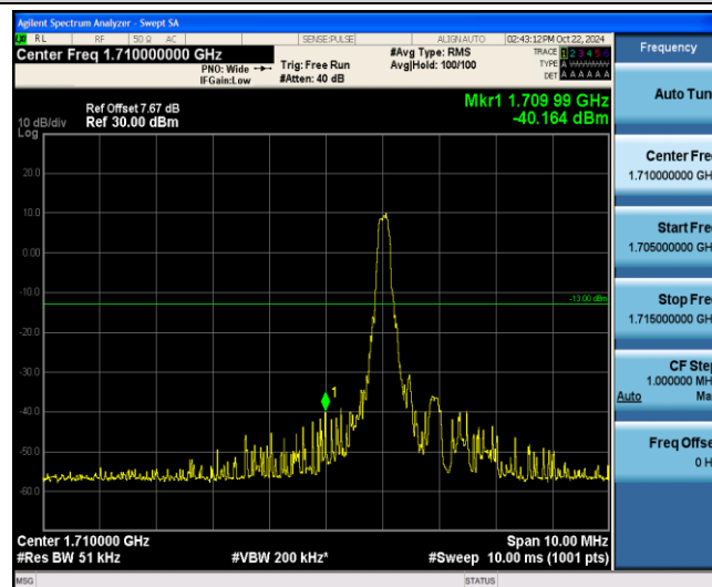
Band4-15MHz-16QAM-20025-1-0-Low--40.16-PASS
