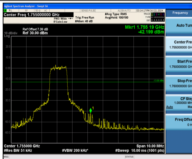
Band4-20MHz-16QAM-20300-6-0-High--42.20-PASS
