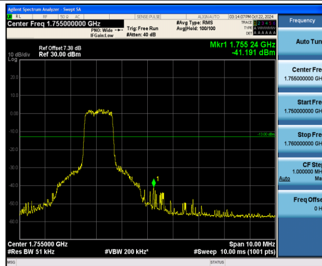
Band4-20MHz-QPSK-20300-6-0-High--41.19-PASS
