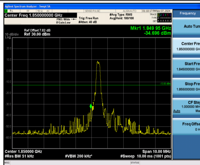
Band25-3MHz-QPSK-26055-1-0-Low--34.70-PASS
