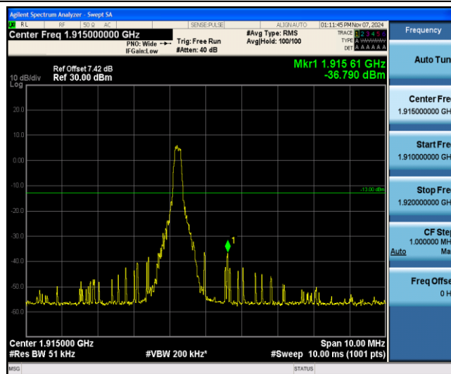
Band25-3MHz-16QAM-26675-1-5-High--36.79-PASS
