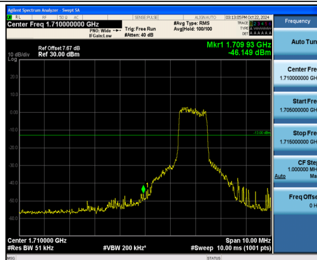
Band4-20MHz-16QAM-20050-6-0-Low--46.15-PASS
