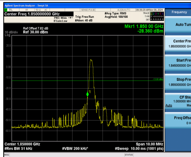
Band25-1.4MHz-16QAM-26047-1-0-Low--28.36-PASS
