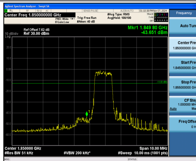
Band25-3MHz-QPSK-26055-6-0-Low--43.65-PASS
