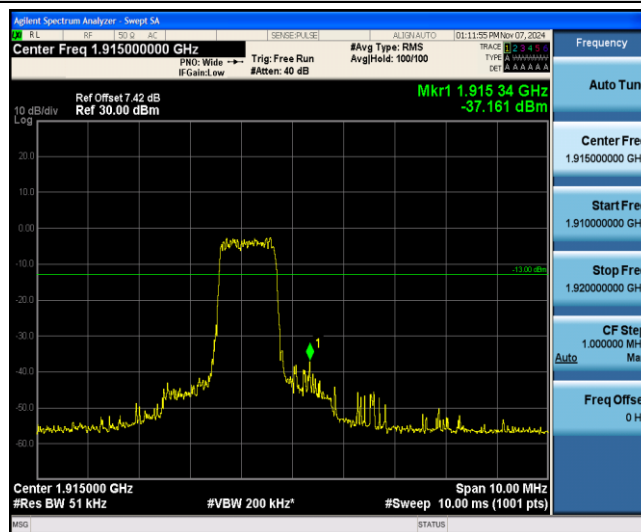
Band25-3MHz-QPSK-26675-6-0-High--37.16-PASS
