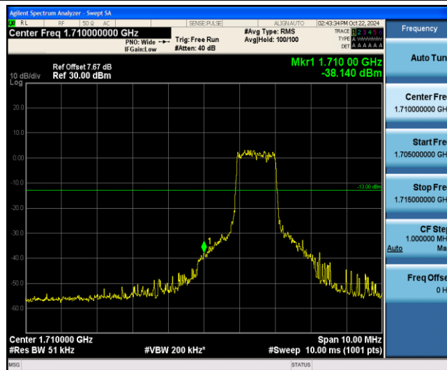
Band4-15MHz-16QAM-20025-6-0-Low--38.14-PASS
