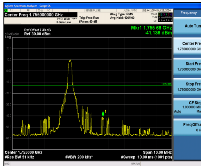
Band4-15MHz-QPSK-20325-1-5-High--41.14-PASS
