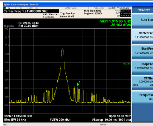
Band25-1.4MHz-16QAM-26683-1-5-High--38.16-PASS
