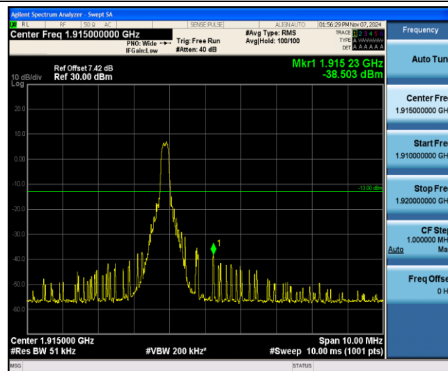
Band25-10MHz-QPSK-26640-1-5-High--38.50-PASS
