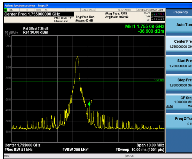
Band4-5MHz-16QAM-20375-1-5-High--36.90-PASS
