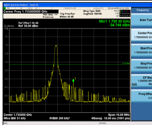
Band4-10MHz-QPSK-20350-1-5-High--34.75-PASS
