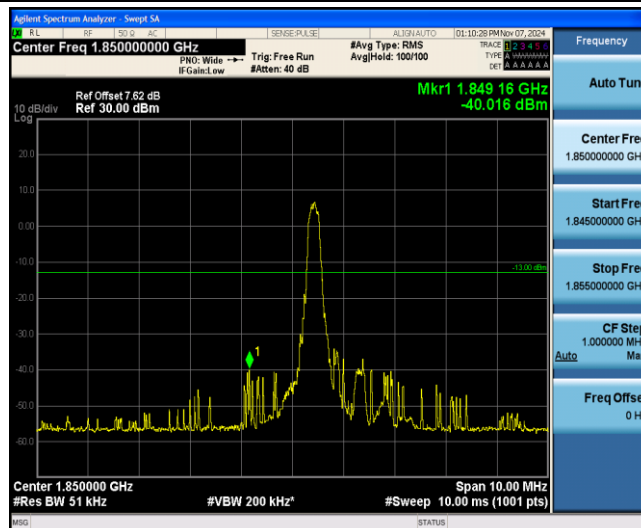
Band25-3MHz-16QAM-26055-1-0-Low--40.02-PASS
