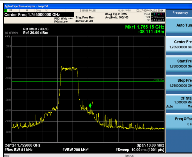
Band4-10MHz-QPSK-20350-6-0-High--38.11-PASS
