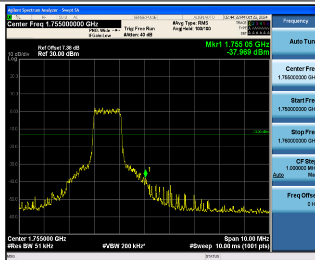
Band4-15MHz-QPSK-20325-6-0-High--37.97-PASS
