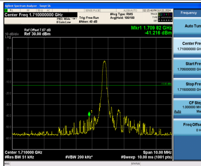
Band4-10MHz-16QAM-20000-1-0-Low--41.22-PASS
