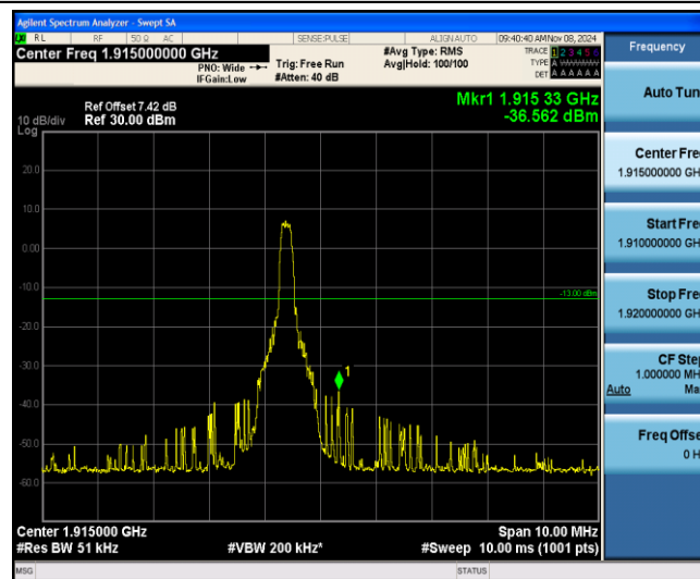
Band25-1.4MHz-QPSK-26683-1-5-High--36.56-PASS
