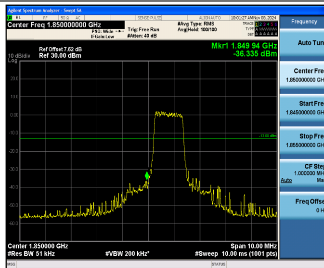
Band25-5MHz-QPSK-26065-6-0-Low--36.33-PASS
