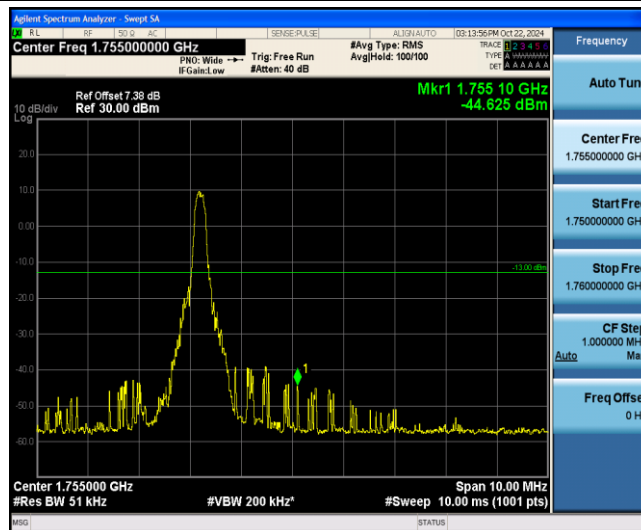
Band4-20MHz-16QAM-20300-1-5-High--44.62-PASS
