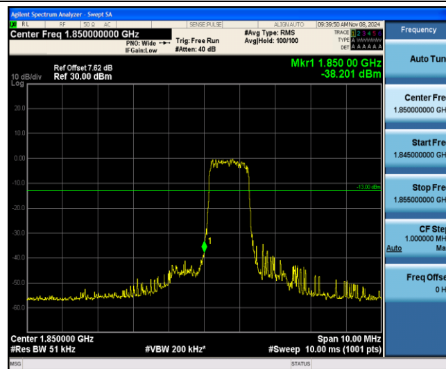
Band25-1.4MHz-16QAM-26047-6-0-Low--38.20-PASS
