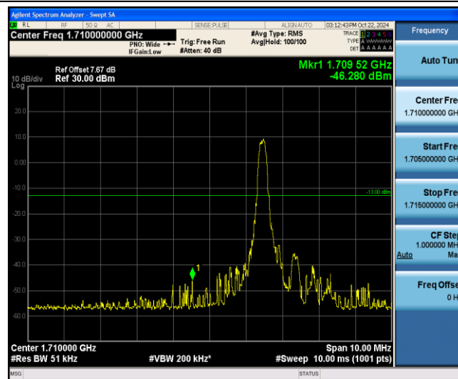
Band4-20MHz-16QAM-20050-1-0-Low--46.28-PASS
