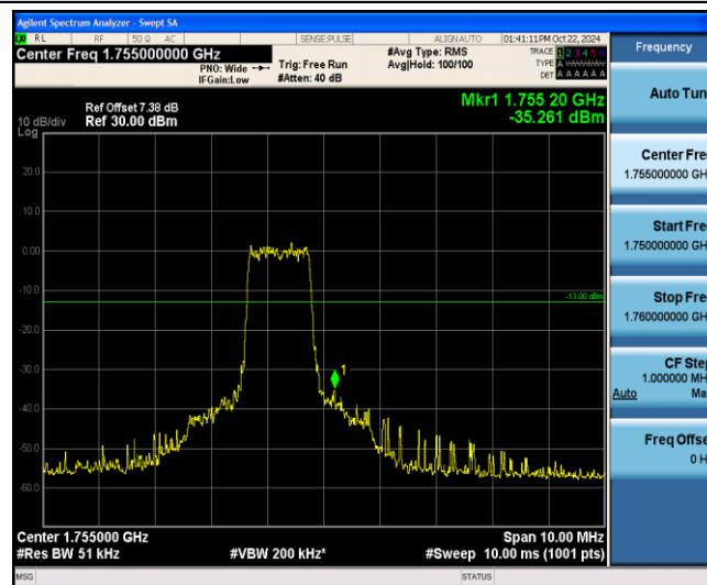
Band4-5MHz-16QAM-20375-6-0-High--35.26-PASS
