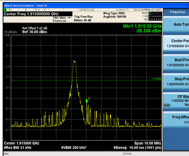
Band25-3MHz-QPSK-26675-1-5-High--35.34-PASS
