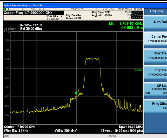
Band4-10MHz-16QAM-20000-6-0-Low--38.98-PASS
