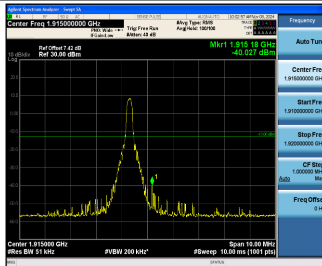
Band25-5MHz-16QAM-26665-1-5-High--40.03-PASS
