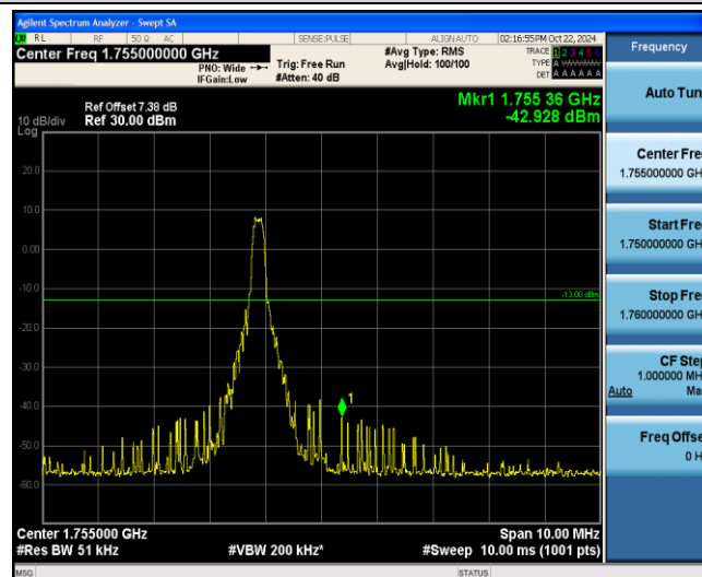
Band4-10MHz-16QAM-20350-1-5-High--42.93-PASS
