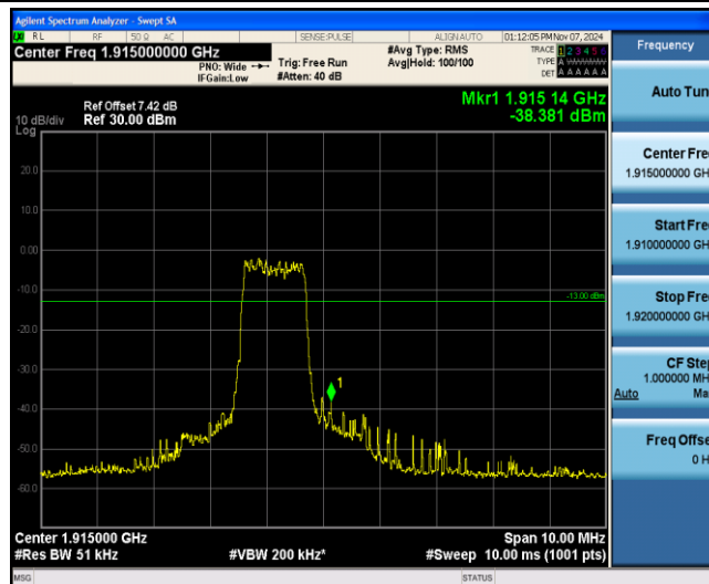
Band25-3MHz-16QAM-26675-6-0-High--38.38-PASS
