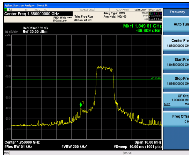
Band25-10MHz-QPSK-26090-6-0-Low--39.61-PASS
