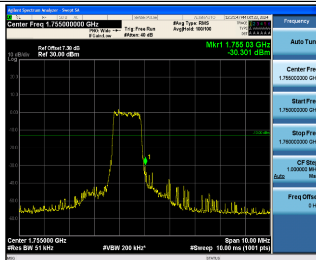
Band4-1.4MHz-QPSK-20393-6-0-High--30.30-PASS
