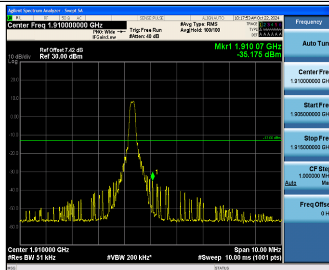
Band2-5MHz-QPSK-19175-1-5-High--35.17-PASS
