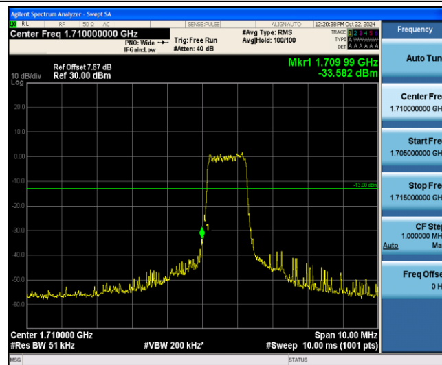
Band4-1.4MHz-16QAM-19957-6-0-Low--33.58-PASS
