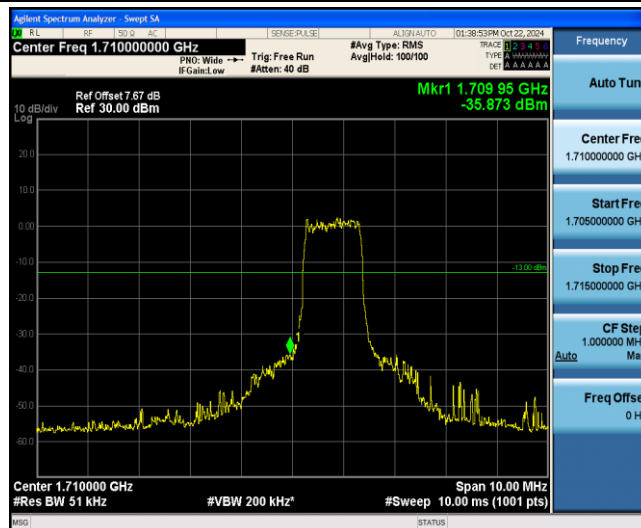
Band4-5MHz-16QAM-19975-6-0-Low--35.87-PASS
