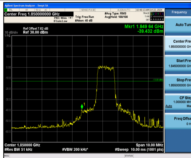
Band2-10MHz-QPSK-18650-6-0-Low--39.43-PASS
