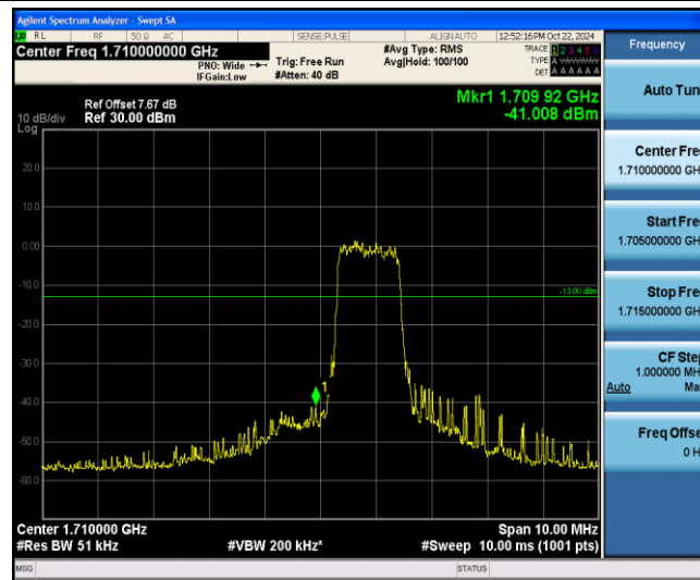
Band4-3MHz-16QAM-19965-6-0-Low--41.01-PASS
