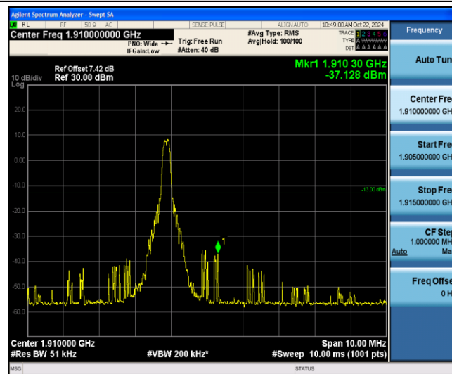
Band2-10MHz-QPSK-19150-1-5-High--37.13-PASS
