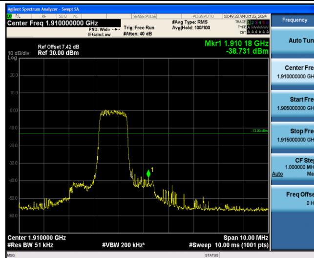
Band2-10MHz-QPSK-19150-6-0-High--38.73-PASS
