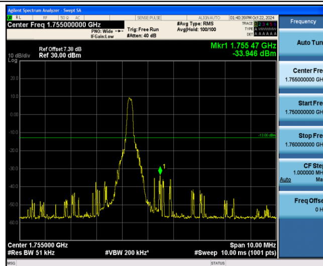
Band4-5MHz-QPSK-20375-1-5-High--33.95-PASS
