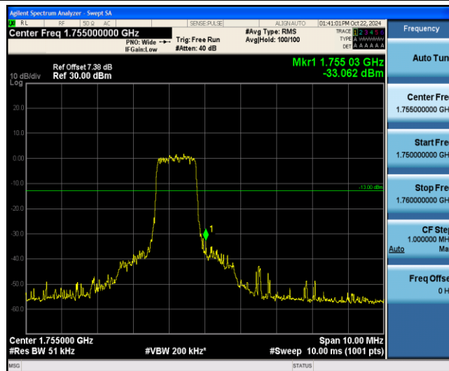
Band4-5MHz-QPSK-20375-6-0-High--33.06-PASS
