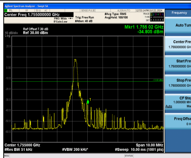
Band4-3MHz-16QAM-20385-1-5-High--34.81-PASS
