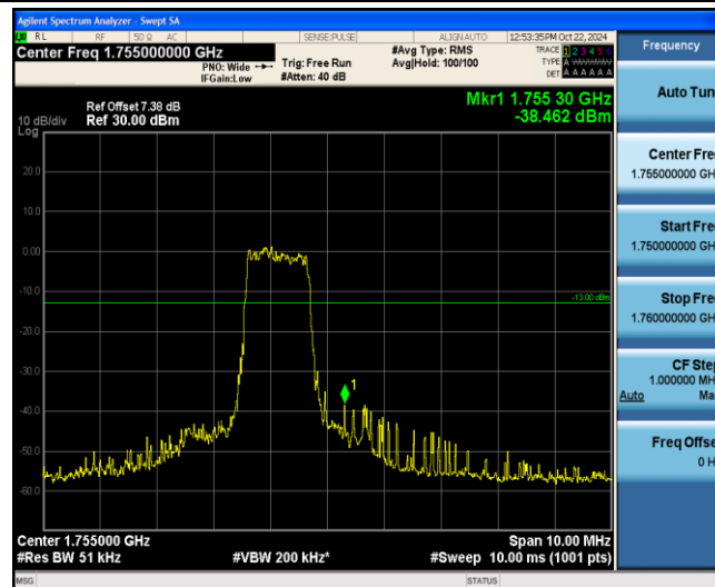
Band4-3MHz-16QAM-20385-6-0-High--38.46-PASS
