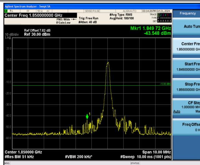
Band2-15MHz-16QAM-18675-1-0-Low--43.55-PASS
