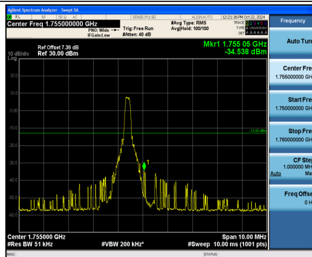
Band4-1.4MHz-16QAM-20393-1-5-High--34.54-PASS
