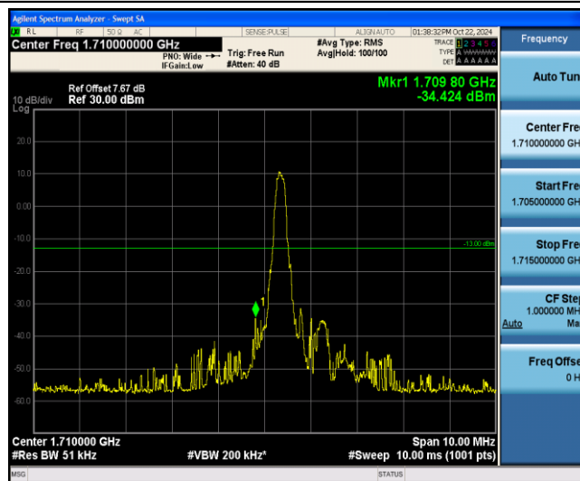
Band4-5MHz-16QAM-19975-1-0-Low--34.42-PASS
