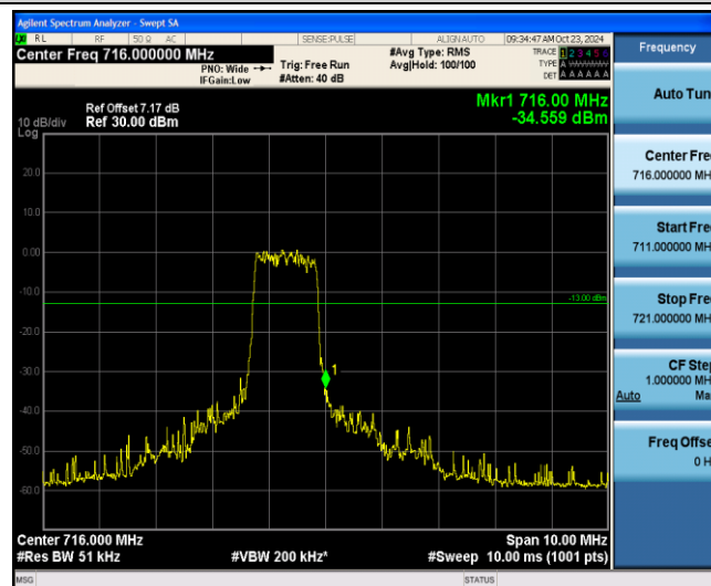
Band12-1.4MHz-QPSK-23173-6-0-High--34.56-PASS
