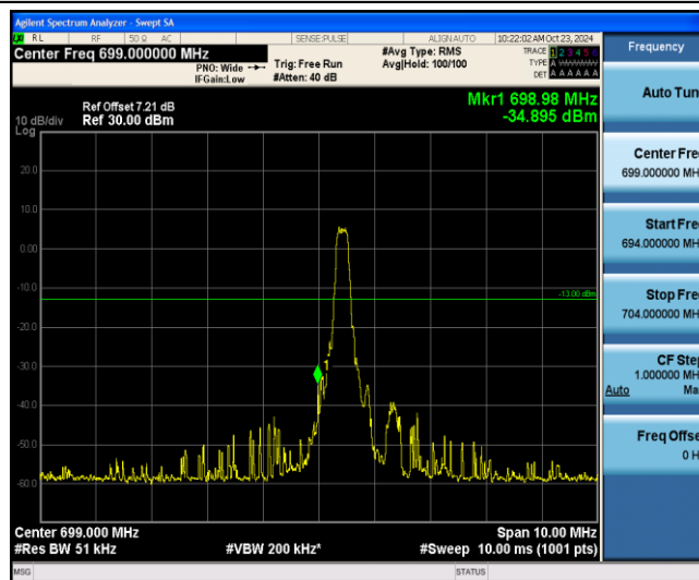
Band12-3MHz-QPSK-23025-1-0-Low--34.90-PASS
