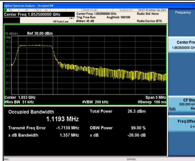
Band25-5MHz-QPSK-26065-6-0-Low-1.1193-1.357-PASS
