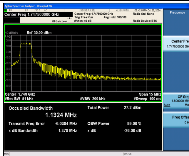
Band4-15MHz-QPSK-20325-6-0-Low-1.1324-1.378-PASS
