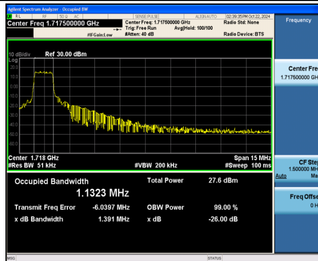
Band4-15MHz-16QAM-20025-6-0-Low-1.1323-1.391-PASS
