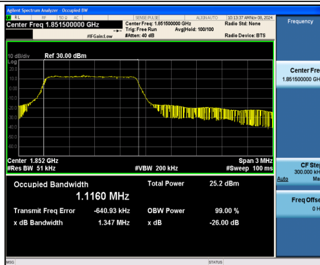
Band25-3MHz-16QAM-26055-6-0-Low-1.1160-1.347-PASS
