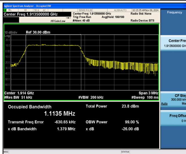
Band25-3MHz-QPSK-26675-6-0-Low-1.1135-1.379-PASS
