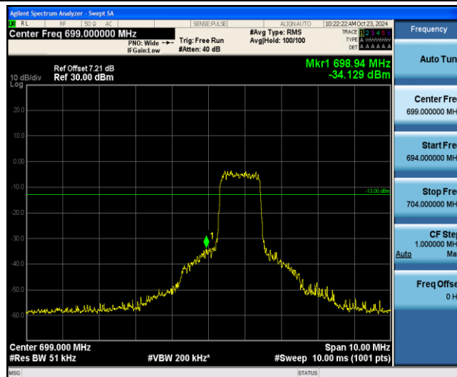
Band12-3MHz-QPSK-23025-6-0-Low--34.13-PASS
