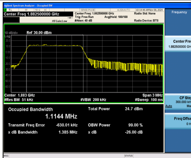
Band25-3MHz-16QAM-26365-6-0-Low-1.1144-1.385-PASS
