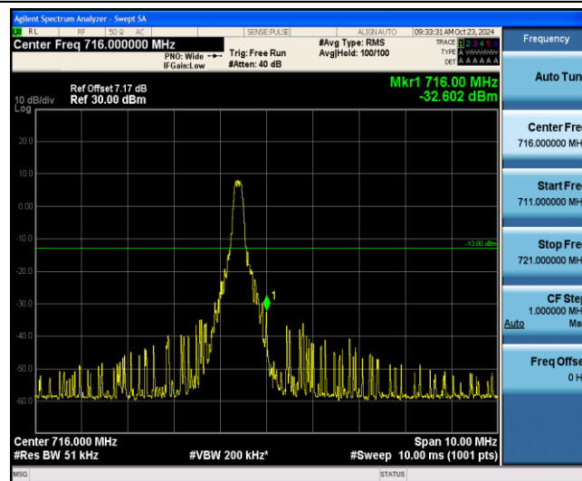
Band12-1.4MHz-QPSK-23173-1-5-High--32.60-PASS
