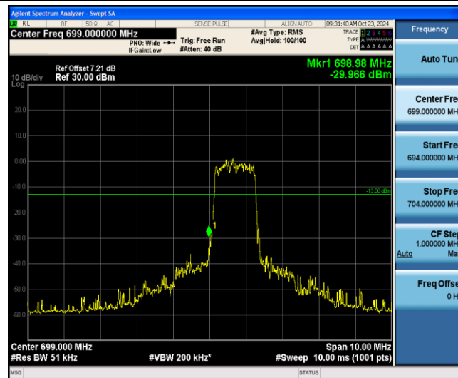
Band12-1.4MHz-QPSK-23017-6-0-Low--29.97-PASS
