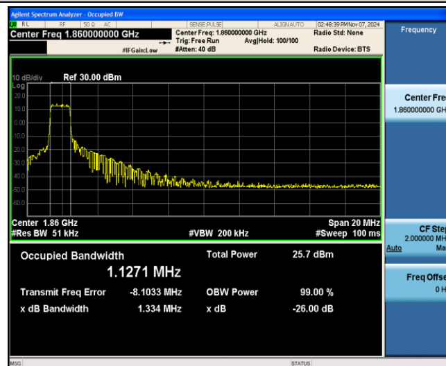
Band25-20MHz-QPSK-26140-6-0-Low-1.1271-1.334-PASS
