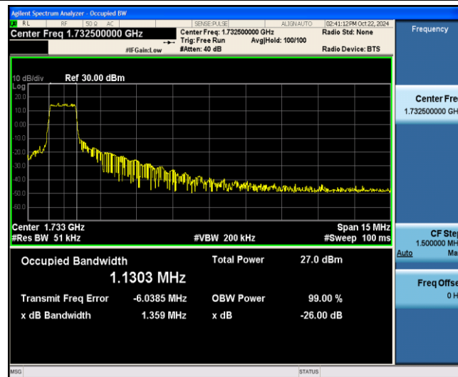
Band4-15MHz-QPSK-20175-6-0-Low-1.1303-1.359-PASS
