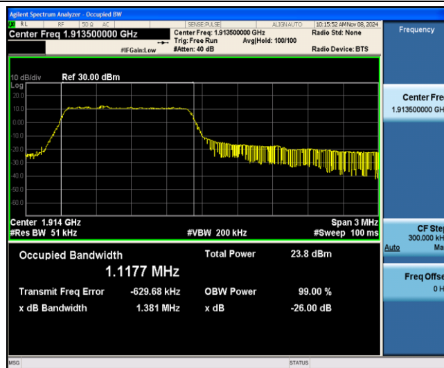
Band25-3MHz-16QAM-26675-6-0-Low-1.1177-1.381-PASS
