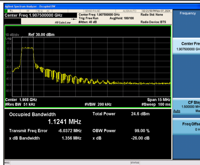
Band25-15MHz-16QAM-26615-6-0-Low-1.1241-1.356-PASS
