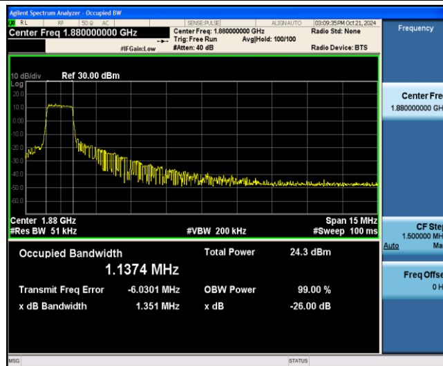
Band2-15MHz-QPSK-18900-6-0-Low-1.1374-1.351-PASS
