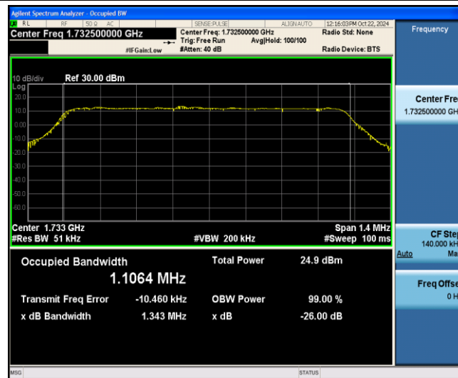
Band4-1.4MHz-QPSK-20175-6-0-Low-1.1064-1.343-PASS
