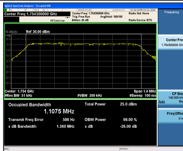
Band4-1.4MHz-QPSK-20393-6-0-Low-1.1075-1.360-PASS
