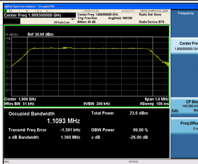
Band2-1.4MHz-16QAM-19193-6-0-Low-1.1093-1.360-PASS
