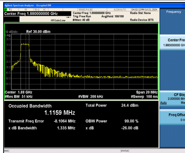
Band2-20MHz-16QAM-18900-6-0-Low-1.1159-1.335-PASS
