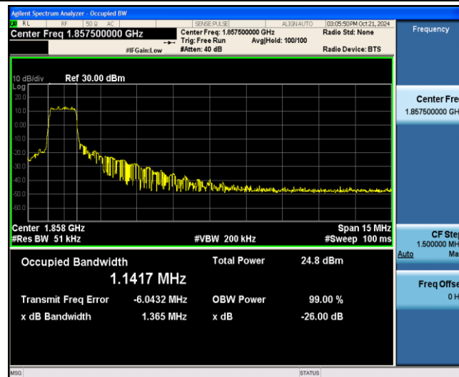
Band2-15MHz-QPSK-18675-6-0-Low-1.1417-1.365-PASS
