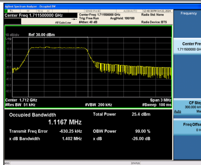
Band4-3MHz-16QAM-19965-6-0-Low-1.1167-1.402-PASS
