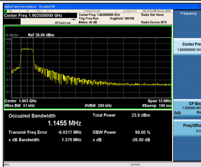
Band2-15MHz-QPSK-19125-6-0-Low-1.1455-1.370-PASS
