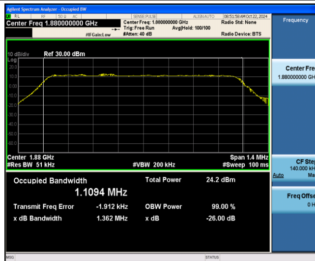
Band2-1.4MHz-16QAM-18900-6-0-Low-1.1094-1.362-PASS
