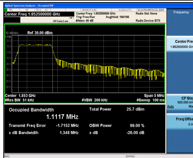
Band2-5MHz-16QAM-18625-6-0-Low-1.1117-1.348-PASS
