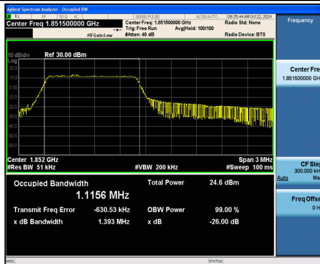
Band2-3MHz-16QAM-18615-6-0-Low-1.1156-1.393-PASS
