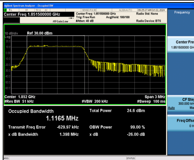
Band2-3MHz-QPSK-18615-6-0-Low-1.1165-1.398-PASS
