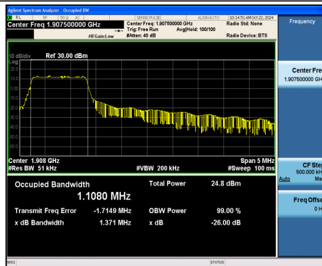
Band2-5MHz-QPSK-19175-6-0-Low-1.1080-1.371-PASS
