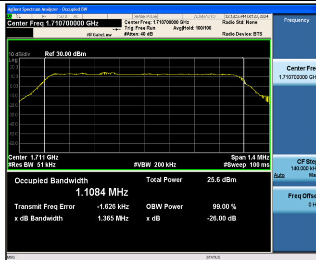
Band4-1.4MHz-16QAM-19957-6-0-Low-1.1084-1.365-PASS
