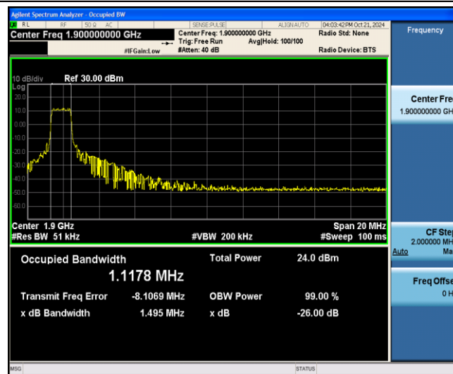
Band2-20MHz-16QAM-19100-6-0-Low-1.1178-1.495-PASS
