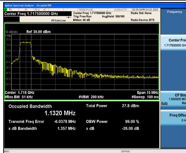
Band4-15MHz-QPSK-20025-6-0-Low-1.1320-1.357-PASS
