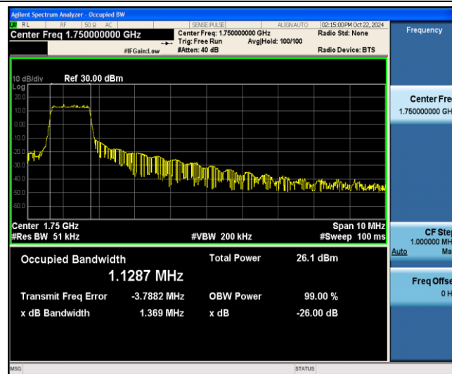
Band4-10MHz-16QAM-20350-6-0-Low-1.1287-1.369-PASS
