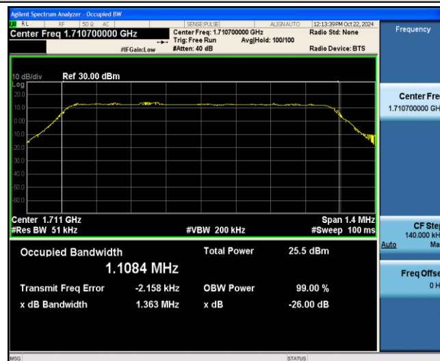
Band4-1.4MHz-QPSK-19957-6-0-Low-1.1084-1.363-PASS
