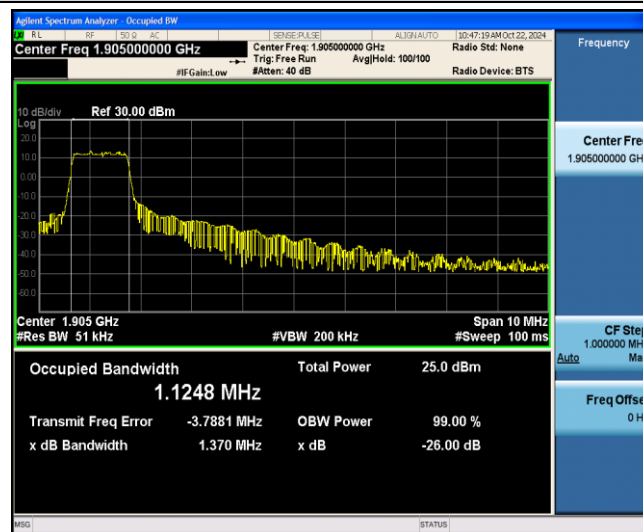
Band2-10MHz-16QAM-19150-6-0-Low-1.1248-1.370-PASS
