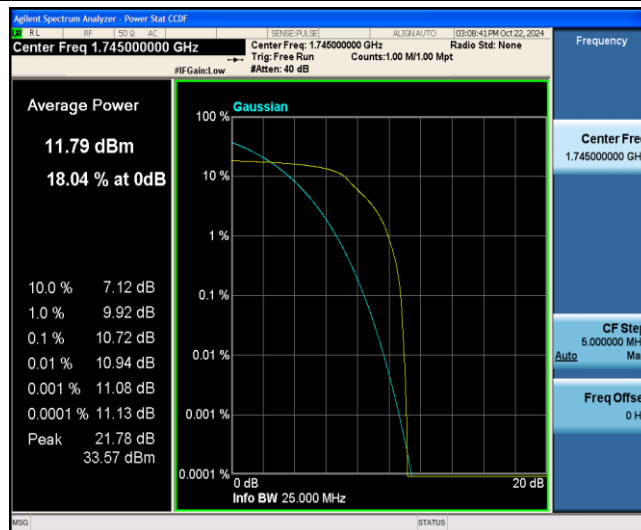
Band4-20MHz-16QAM-20300-6-0-Low-10.72-&lt;=13-PASS
