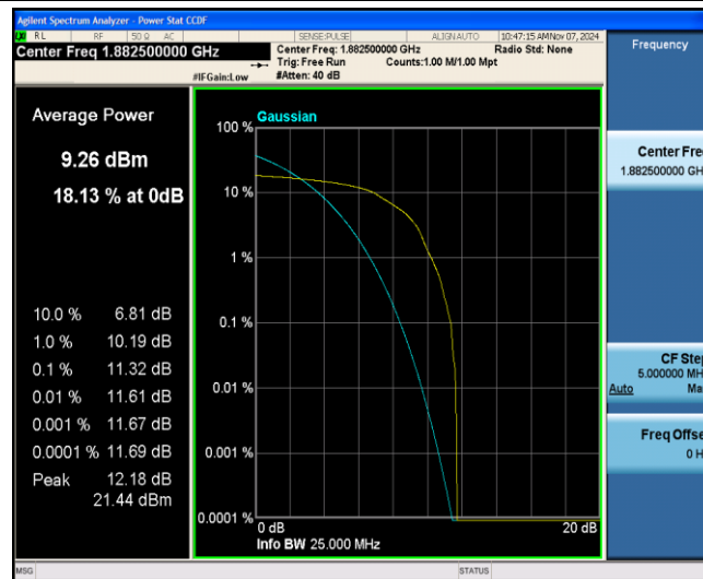
Band25-1.4MHz-16QAM-26365-1-0-Low-11.32-13-PASS
