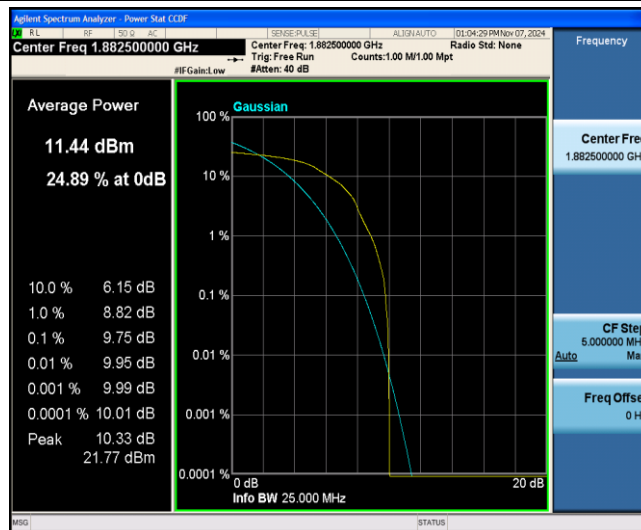
Band25-3MHz-16QAM-26365-1-0-Low-9.75-13-PASS
