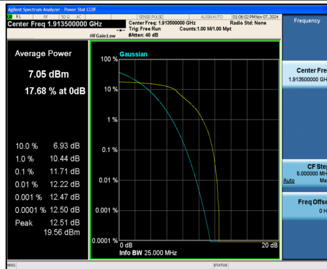
Band25-3MHz-16QAM-26675-6-0-Low-11.71-&lt;=13-PASS
