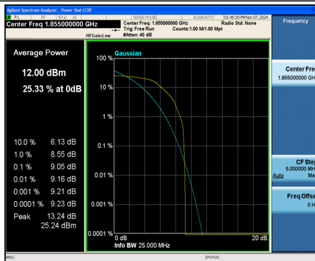
Band25-10MHz-QPSK-26090-1-0-Low-9.05-&lt;=13-PASS
