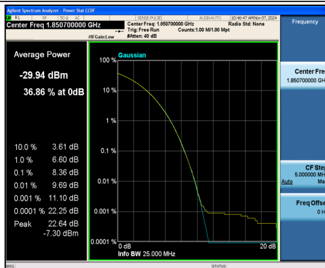
Band25-1.4MHz-QPSK-26047-6-0-Low-8.36-&lt;=13-PASS
