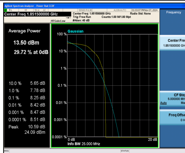
Band25-3MHz-QPSK-26055-1-0-Low-8.25-&lt;=13-PASS
