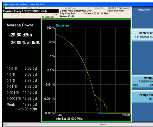
Band25-5MHz-QPSK-26665-6-0-Low-8.37-&lt;=13-PASS
