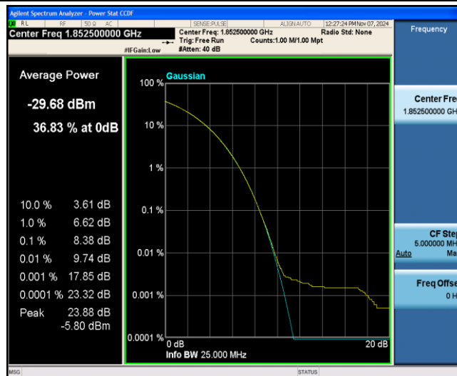
Band25-5MHz-16QAM-26065-6-0-Low-8.38-&lt;=13-PASS
