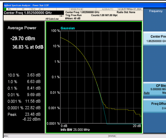
Band25-5MHz-QPSK-26065-1-0-Low-8.41-&lt;=13-PASS
