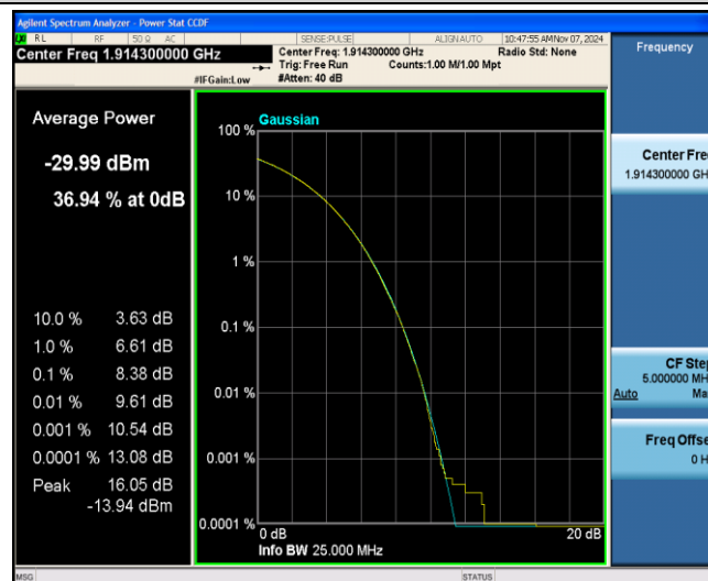
Band25-1.4MHz-16QAM-26683-1-0-Low-8.38-13-PASS
