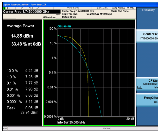
Band4-20MHz-QPSK-20300-6-0-Low-7.77-=&lt;=13-PASS
