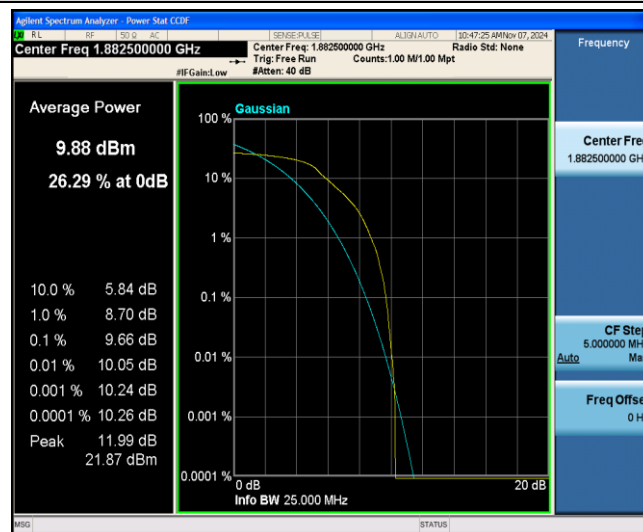
Band25-1.4MHz-QPSK-26365-6-0-Low-9.66-&lt;=13-PASS
