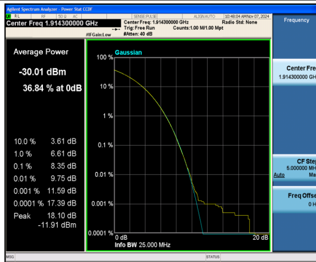
Band25-1.4MHz-QPSK-26683-6-0-Low-8.35-≤13-PASS
