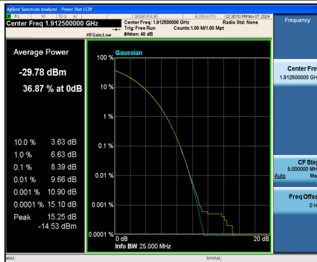
Band25-5MHz-16QAM-26665-6-0-Low-8.39-&lt;=13-PASS
