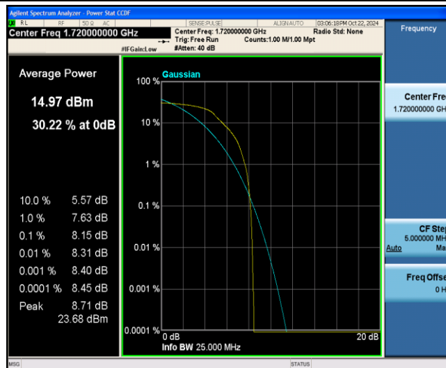
Band4-20MHz-16QAM-20050-6-0-Low-8.15-=&lt;=13-PASS
