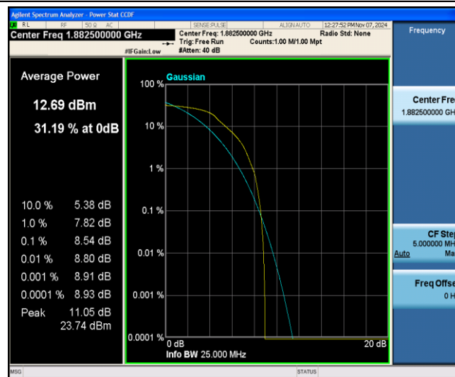
Band25-5MHz-QPSK-26365-6-0-Low-8.54-&lt;=13-PASS
