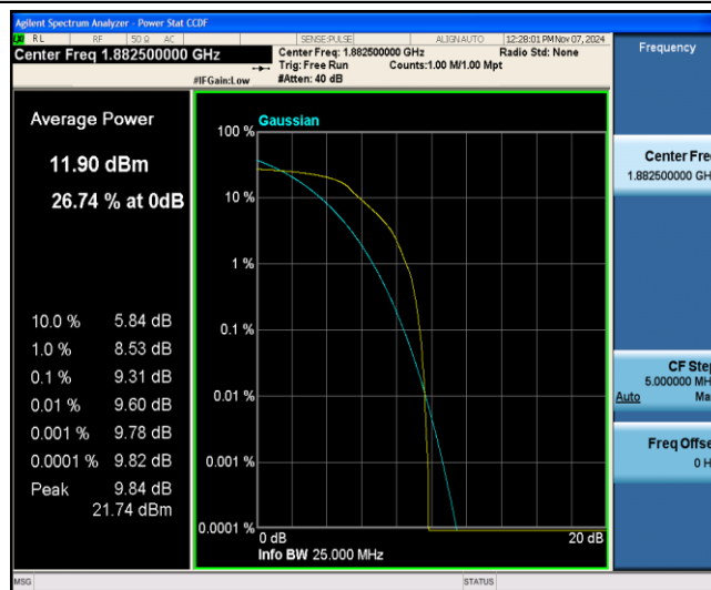
Band25-5MHz-16QAM-26365-6-0-Low-9.31-&lt;=13-PASS
