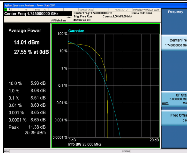
Band4-20MHz-QPSK-20300-1-0-Low-8.51-&lt;=13-PASS
