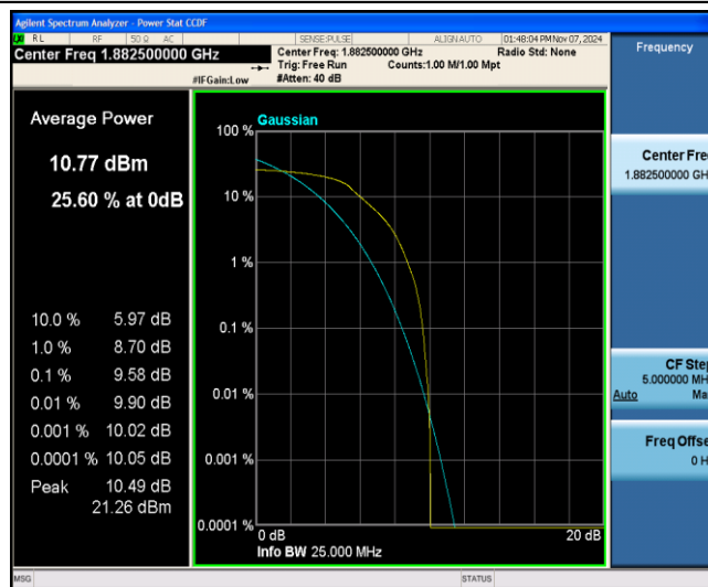
Band25-10MHz-16QAM-26365-6-0-Low-9.58-&lt;=13-PASS
