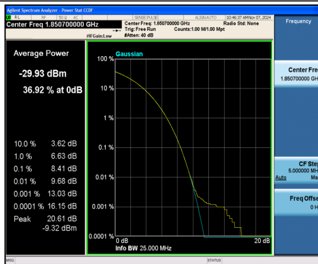
Band25-1.4MHz-16QAM-26047-1-0-Low-8.41-≤13-PASS
