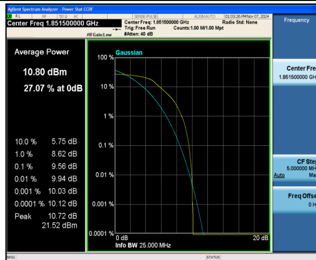
Band25-3MHz-QPSK-26055-6-0-Low-9.56-&lt;=13-PASS
