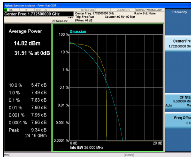
Band4-20MHz-QPSK-20175-1-0-Low-7.83-&lt;=13-PASS
