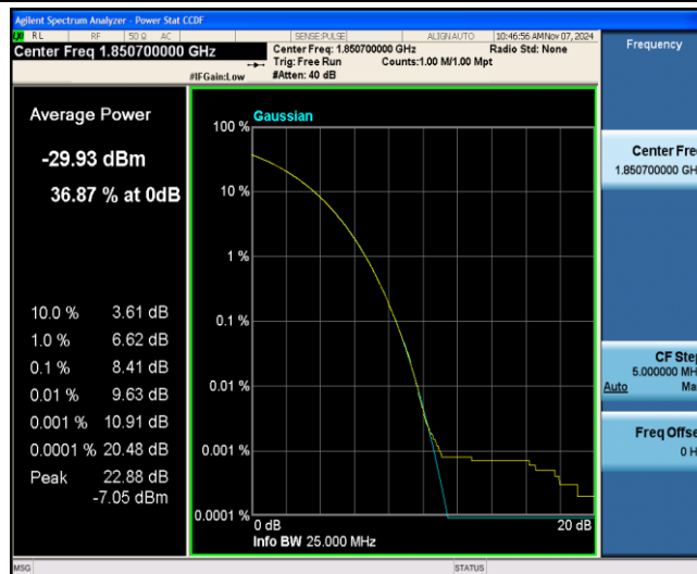
Band25-1.4MHz-16QAM-26047-6-0-Low-8.41-≤13-PASS
