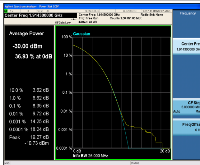
Band25-1.4MHz-QPSK-26683-1-0-Low-8.35-&lt;=13-PASS
