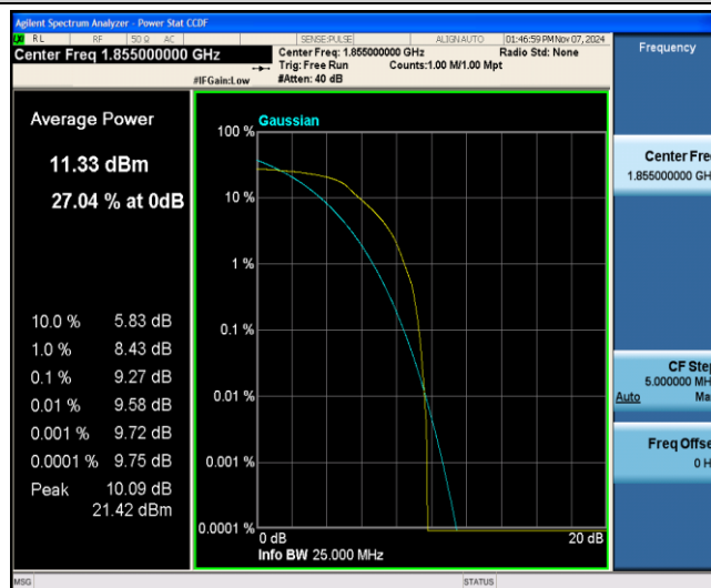
Band25-10MHz-16QAM-26090-6-0-Low-9.27-&lt;=13-PASS
