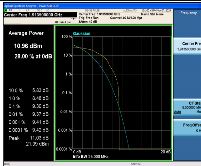
Band25-3MHz-16QAM-26675-1-0-Low-9.30-13-PASS
