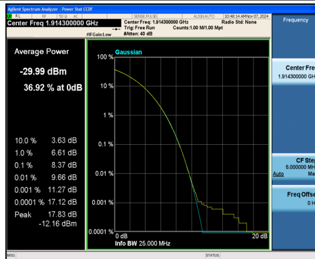
Band25-1.4MHz-16QAM-26683-6-0-Low-8.37-&lt;=13-PASS
