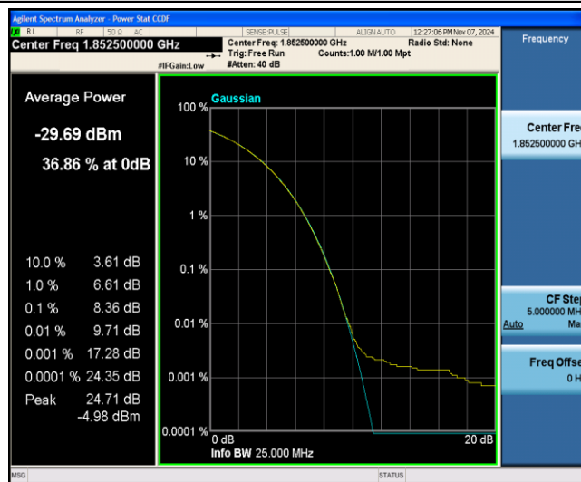
Band25-5MHz-16QAM-26065-1-0-Low-8.36-&lt;=13-PASS
