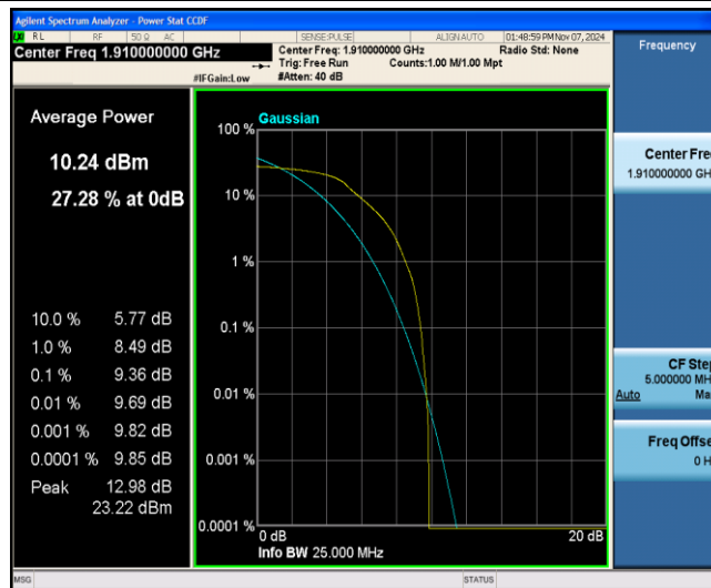
Band25-10MHz-QPSK-26640-6-0-Low-9.36-&lt;=13-PASS
