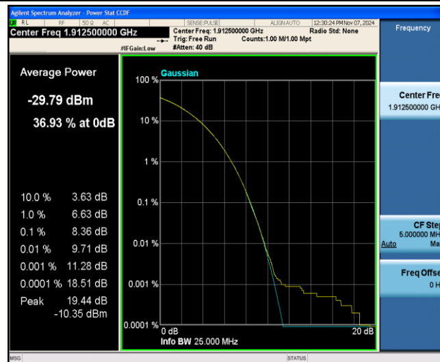
Band25-5MHz-QPSK-26665-1-0-Low-8.36-&lt;=13-PASS
