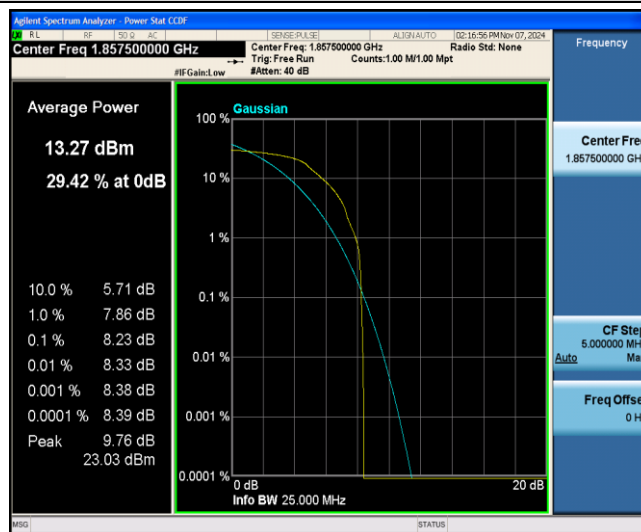
Band25-15MHz-QPSK-26115-1-0-Low-8.23-&lt;=13-PASS
