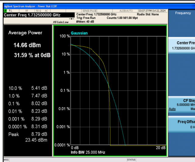
Band4-20MHz-16QAM-20175-6-0-Low-8.02-=&lt;=13-PASS
