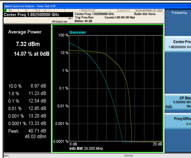
Band25-3MHz-16QAM-26365-6-0-Low-12.54-13-PASS
