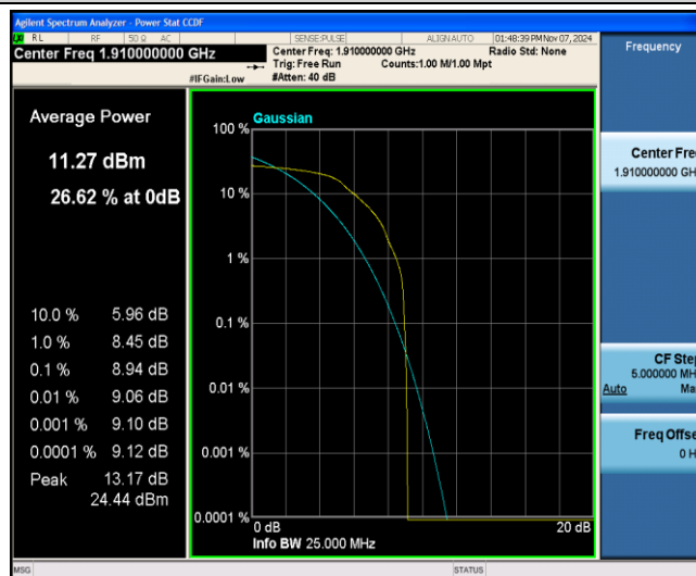
Band25-10MHz-QPSK-26640-1-0-Low-8.94-&lt;=13-PASS
