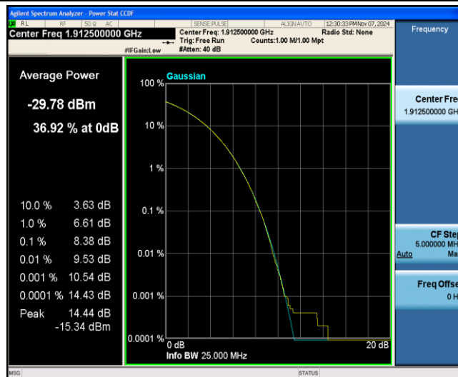
Band25-5MHz-16QAM-26665-1-0-Low-8.38-&lt;=13-PASS
