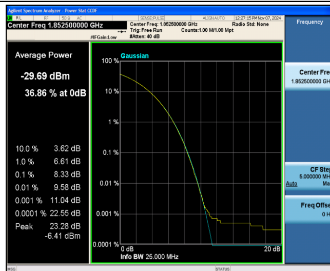
Band25-5MHz-QPSK-26065-6-0-Low-8.33-&lt;=13-PASS
