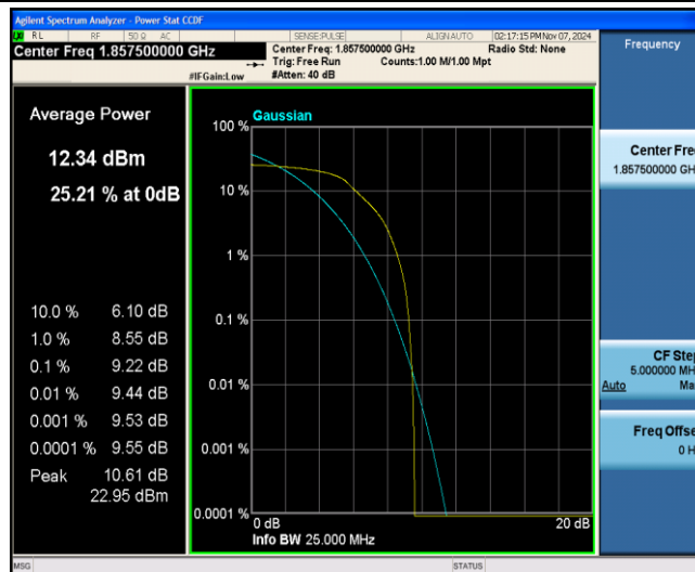
Band25-15MHz-QPSK-26115-6-0-Low-9.22-&lt;=13-PASS
