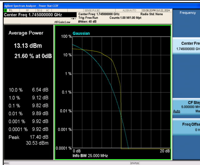
Band4-20MHz-16QAM-20300-1-0-Low-9.82-=&lt;=13-PASS
