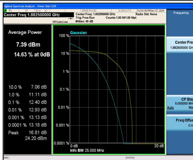
Band25-3MHz-QPSK-26365-6-0-Low-12.40-&lt;=13-PASS
