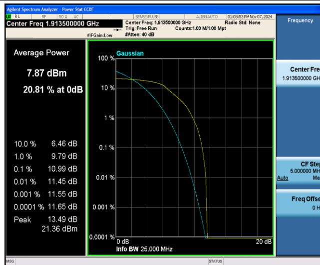
Band25-3MHz-QPSK-26675-6-0-Low-10.99-&lt;=13-PASS
