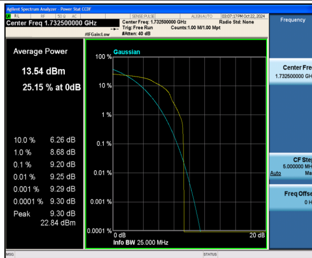
Band4-20MHz-16QAM-20175-1-0-Low-9.20-=&lt;=13-PASS
