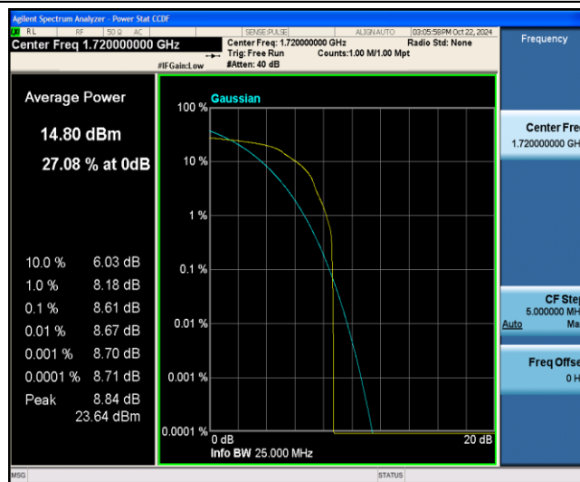
Band4-20MHz-16QAM-20050-1-0-Low-8.61-=&lt;=13-PASS
