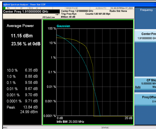
Band25-10MHz-16QAM-26640-1-0-Low-9.58-&lt;=13-PASS
