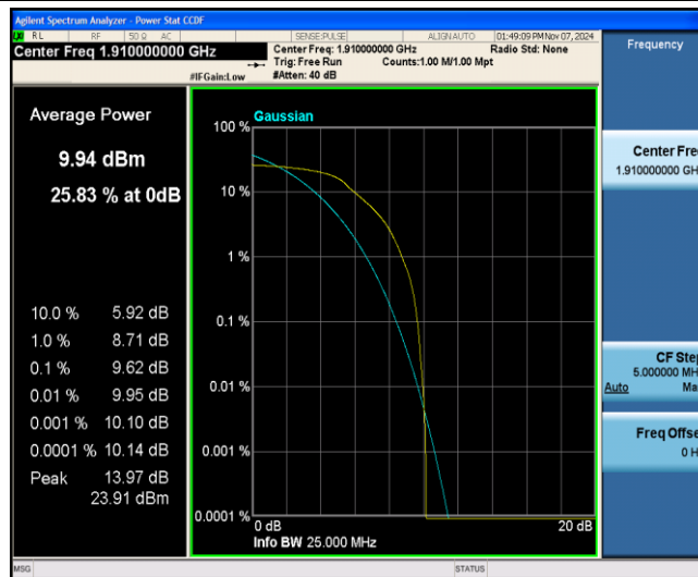
Band25-10MHz-16QAM-26640-6-0-Low-9.62-&lt;=13-PASS
