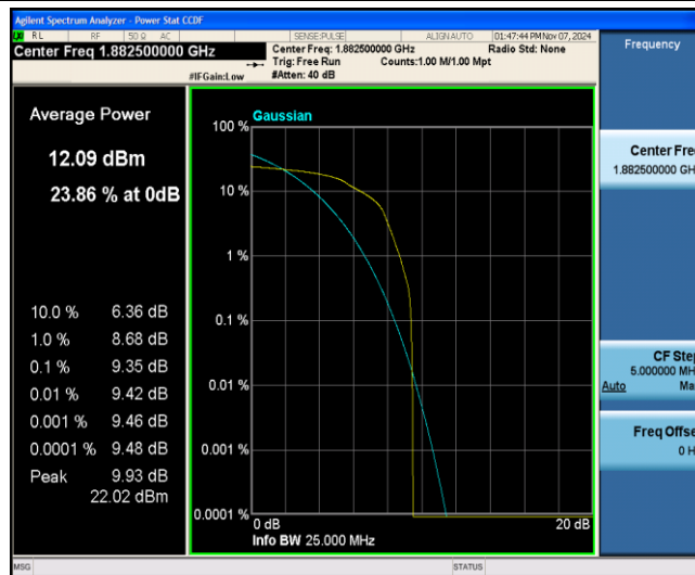
Band25-10MHz-16QAM-26365-1-0-Low-9.35-&lt;=13-PASS
