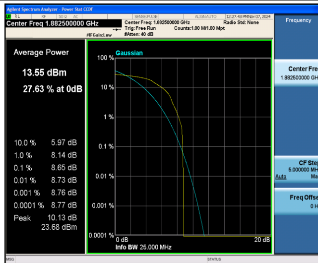
Band25-5MHz-16QAM-26365-1-0-Low-8.65-&lt;=13-PASS
