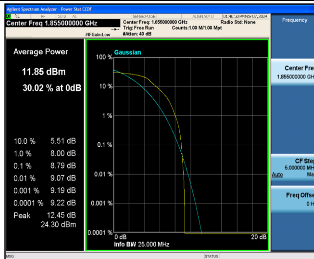
Band25-10MHz-QPSK-26090-6-0-Low-8.79-&lt;=13-PASS
