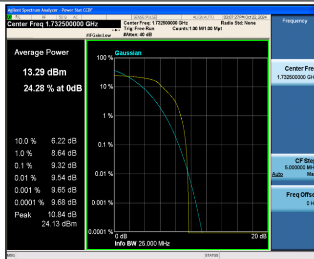
Band4-20MHz-QPSK-20175-6-0-Low-9.32-&lt;=13-PASS
