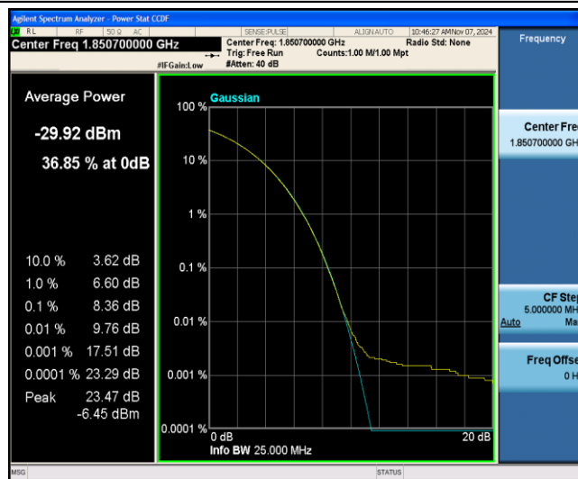
Band25-1.4MHz-QPSK-26047-1-0-Low-8.36-&lt;=13-PASS
