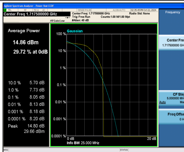
Band4-15MHz-QPSK-20025-1-0-Low-8.05-&lt;=13-PASS
