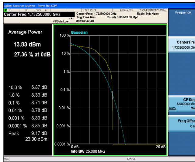
Band4-5MHz-QPSK-20175-1-0-Low-8.71-&lt;=13-PASS
