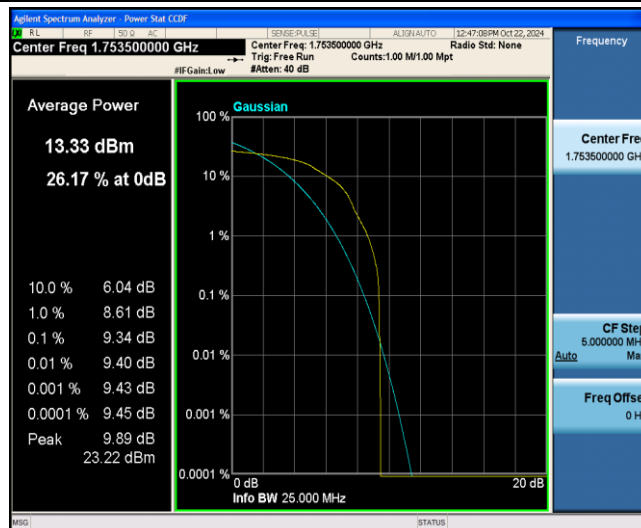
Band4-3MHz-16QAM-20385-1-0-Low-9.34-&lt;=13-PASS
