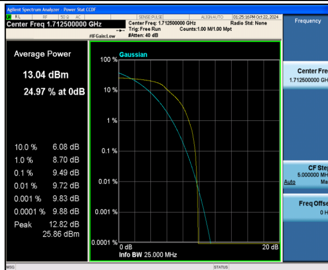
Band4-5MHz-QPSK-19975-6-0-Low-9.49-13-PASS
