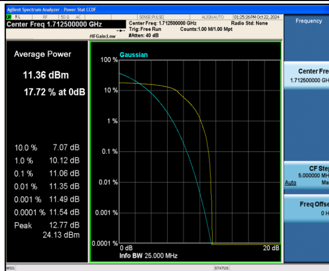
Band4-5MHz-16QAM-19975-6-0-Low-11.06-&lt;=13-PASS
