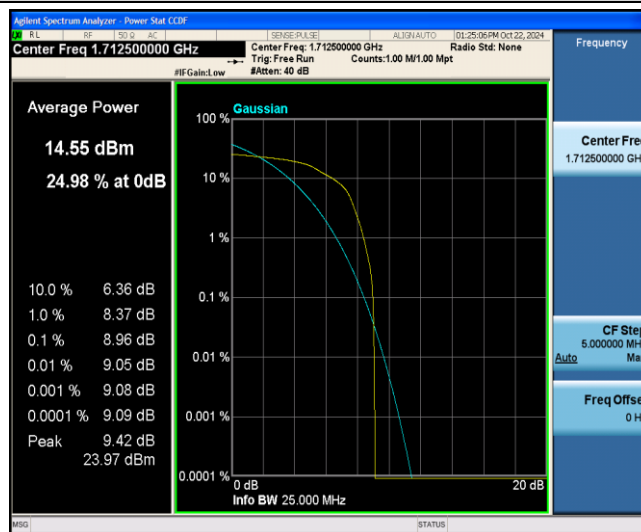
Band4-5MHz-16QAM-19975-1-0-Low-8.96-&lt;=13-PASS
