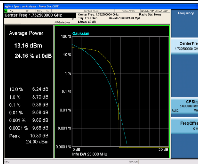
Band4-15MHz-16QAM-20175-6-0-Low-9.36-=&lt;=13-PASS
