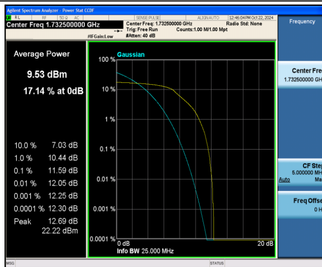
Band4-3MHz-QPSK-20175-6-0-Low-11.59-&lt;=13-PASS
