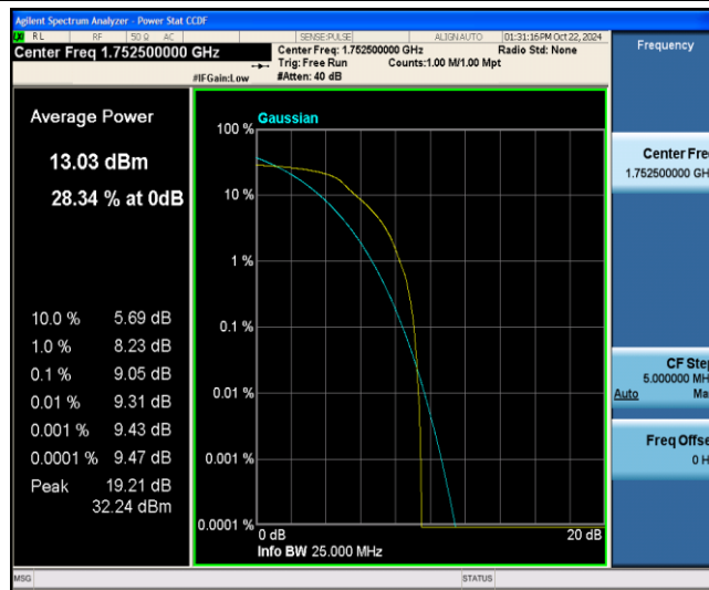
Band4-5MHz-16QAM-20375-6-0-Low-9.05-&lt;=13-PASS
