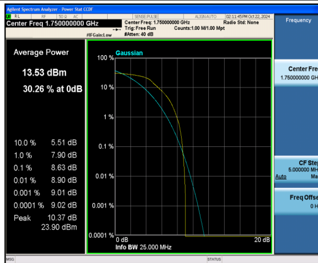
Band4-10MHz-16QAM-20350-6-0-Low-8.63-&lt;=13-PASS
