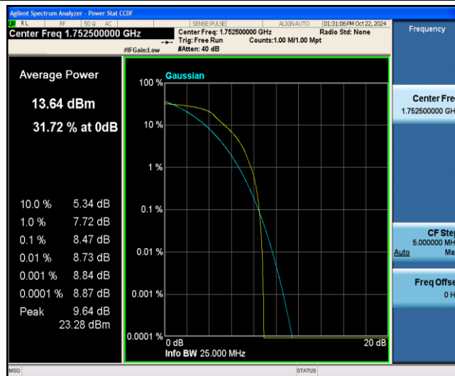
Band4-5MHz-QPSK-20375-6-0-Low-8.47-&lt;=13-PASS
