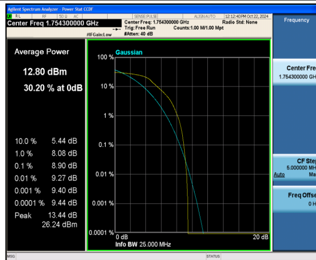
Band4-1.4MHz-16QAM-20393-6-0-Low-8.90-&lt;=13-PASS
