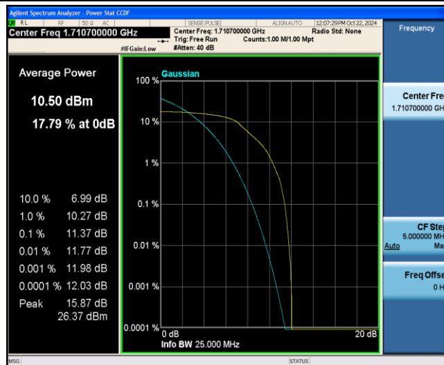
Band4-1.4MHz-16QAM-19957-6-0-Low-11.37-&lt;=13-PASS
