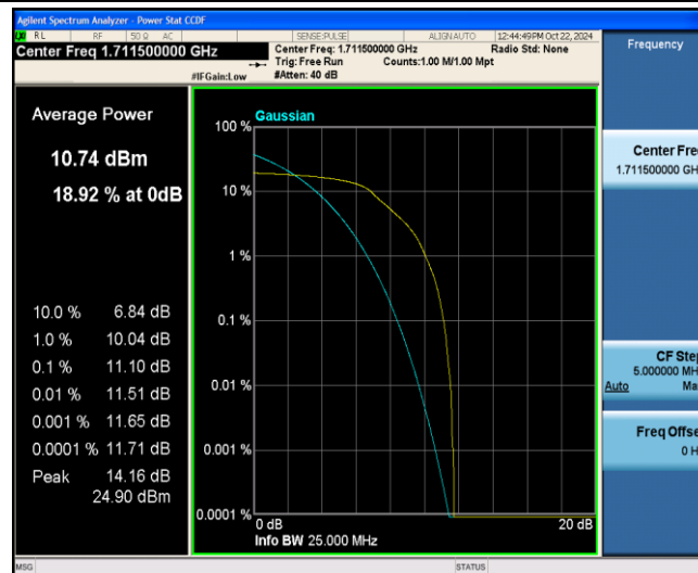
Band4-3MHz-QPSK-19965-6-0-Low-11.10-&lt;=13-PASS
