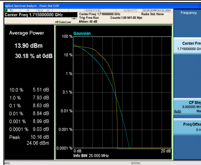
Band4-10MHz-16QAM-20000-6-0-Low-8.63-&lt;=13-PASS
