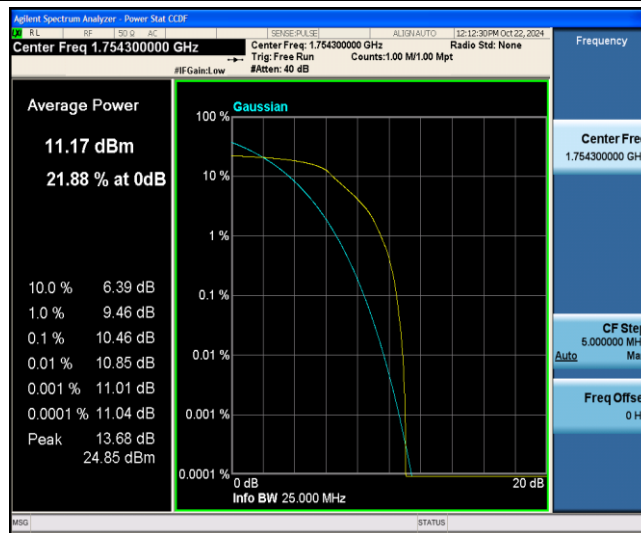
Band4-1.4MHz-QPSK-20393-6-0-Low-10.46-&lt;=13-PASS
