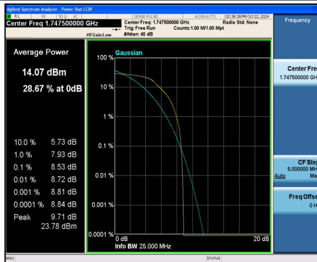
Band4-15MHz-16QAM-20325-6-0-Low-8.53-&lt;=13-PASS
