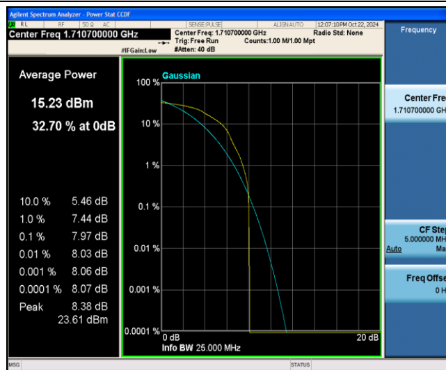
Band4-1.4MHz-16QAM-19957-1-0-Low-7.97-&lt;=13-PASS
