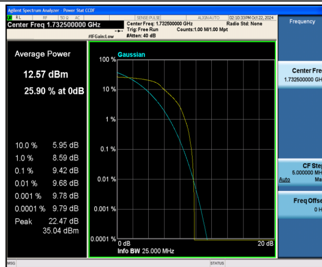
Band4-10MHz-16QAM-20175-6-0-Low-9.42-=&lt;=13-PASS
