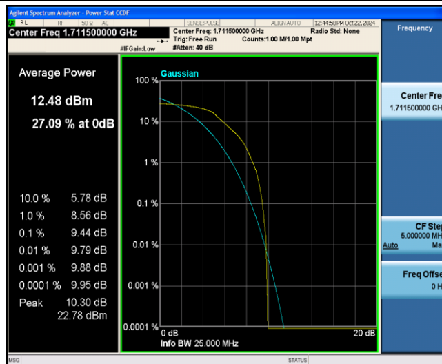
Band4-3MHz-16QAM-19965-6-0-Low-9.44-&lt;=13-PASS
