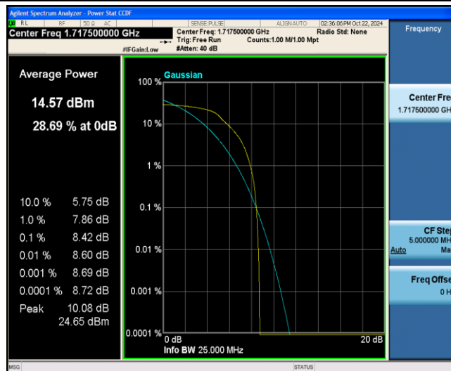
Band4-15MHz-QPSK-20025-6-0-Low-8.42-&lt;=13-PASS
