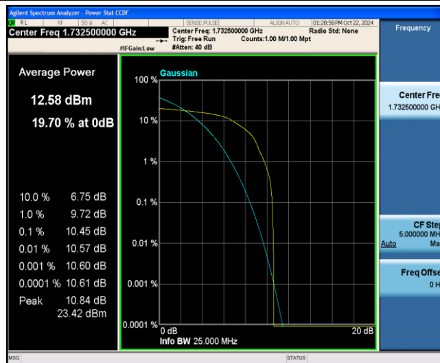
Band4-5MHz-16QAM-20175-1-0-Low-10.45-&lt;=13-PASS
