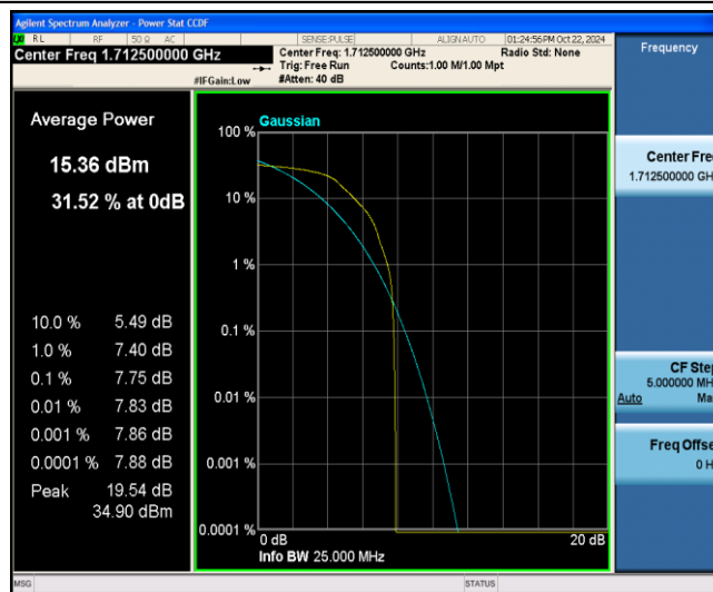
Band4-5MHz-QPSK-19975-1-0-Low-7.75-13-PASS
