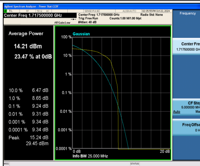
Band4-15MHz-16QAM-20025-1-0-Low-9.24-&lt;=13-PASS
