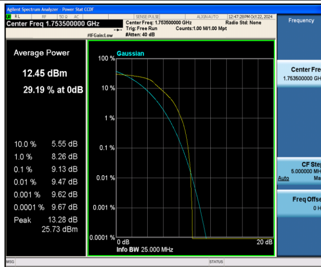
Band4-3MHz-16QAM-20385-6-0-Low-9.13-13-PASS
