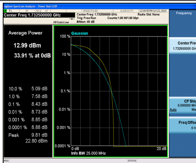
Band4-1.4MHz-QPSK-20175-6-0-Low-8.43-&lt;=13-PASS
