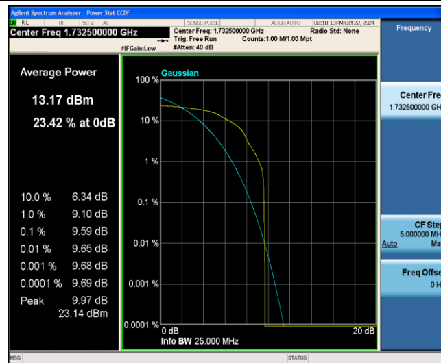
Band4-10MHz-16QAM-20175-1-0-Low-9.59-=&lt;=13-PASS
