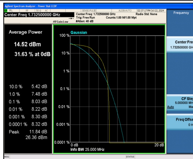
Band4-15MHz-QPSK-20175-6-0-Low-8.03-&lt;=13-PASS
