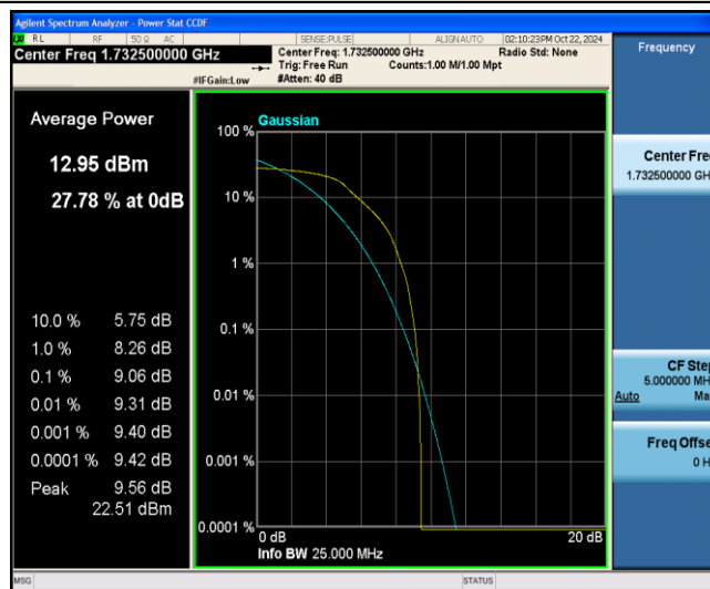
Band4-10MHz-QPSK-20175-6-0-Low-9.06-&lt;=13-PASS
