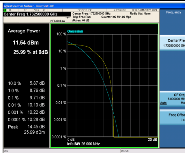
Band4-3MHz-16QAM-20175-6-0-Low-9.71-&lt;=13-PASS
