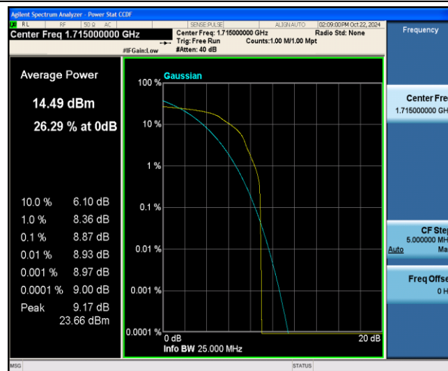
Band4-10MHz-16QAM-20000-1-0-Low-8.87-&lt;=13-PASS
