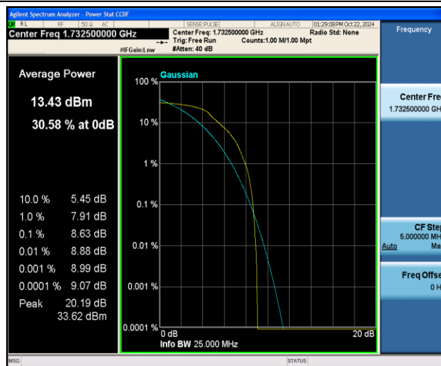
Band4-5MHz-QPSK-20175-6-0-Low-8.63-&lt;=13-PASS
