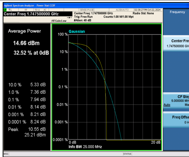
Band4-15MHz-QPSK-20325-6-0-Low-7.94-&lt;=13-PASS
