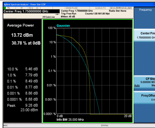
Band4-10MHz-QPSK-20350-6-0-Low-8.49-&lt;=13-PASS
