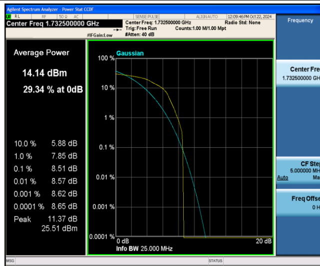
Band4-1.4MHz-16QAM-20175-1-0-Low-8.51- &lt;=13-PASS
