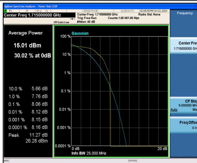
Band4-10MHz-QPSK-20000-1-0-Low-8.06-&lt;=13-PASS
