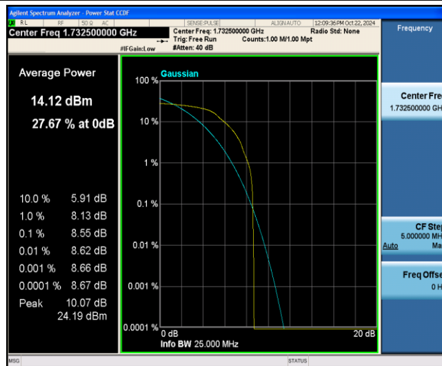
Band4-1.4MHz-QPSK-20175-1-0-Low-8.55-&lt;=13-PASS
