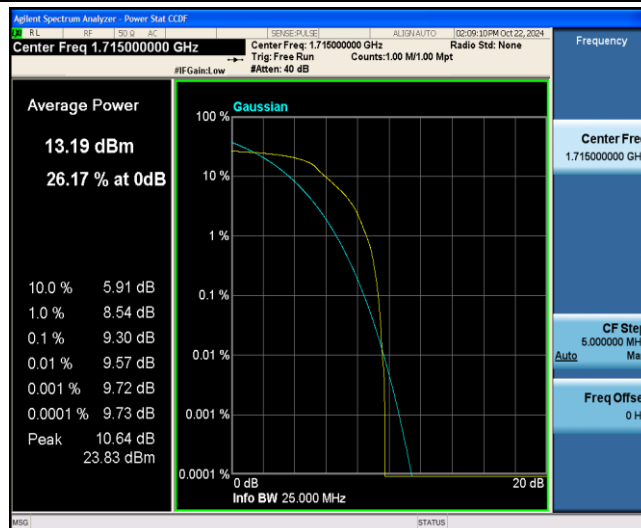
Band4-10MHz-QPSK-20000-6-0-Low-9.30-&lt;=13-PASS
