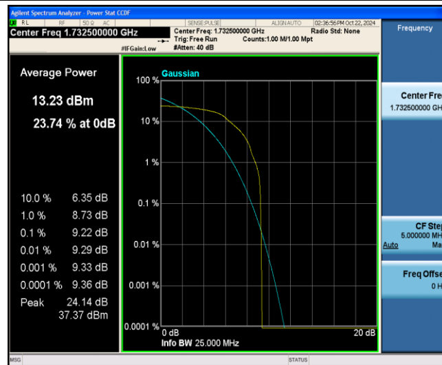
Band4-15MHz-QPSK-20175-1-0-Low-9.22-&lt;=13-PASS
