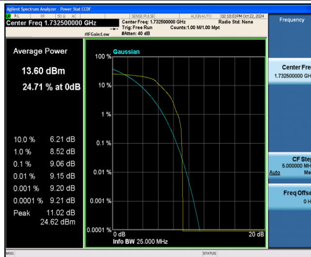
Band4-10MHz-QPSK-20175-1-0-Low-9.06-&lt;=13-PASS
