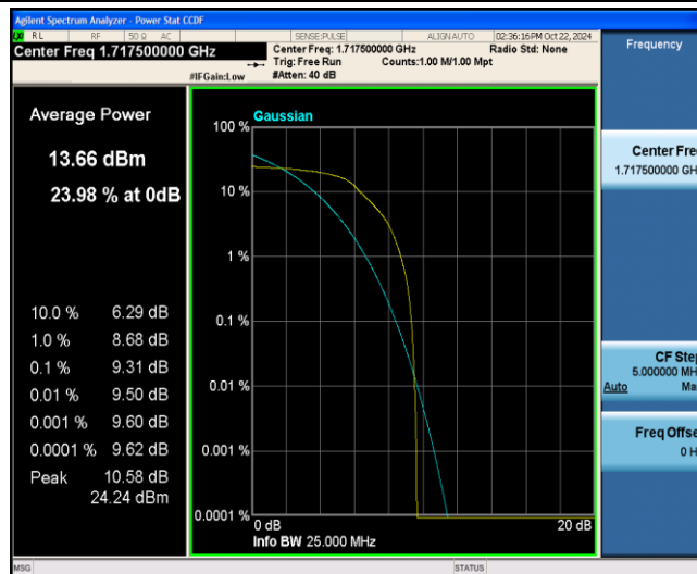
Band4-15MHz-16QAM-20025-6-0-Low-9.31-&lt;=13-PASS
