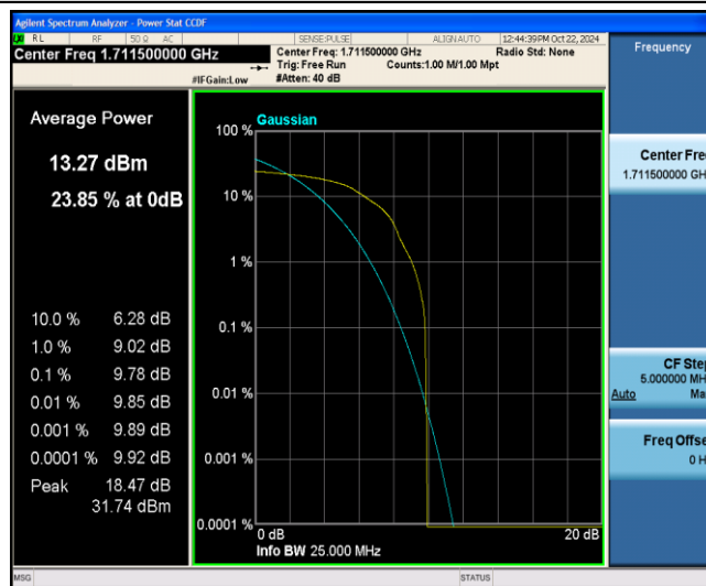
Band4-3MHz-16QAM-19965-1-0-Low-9.78-&lt;=13-PASS
