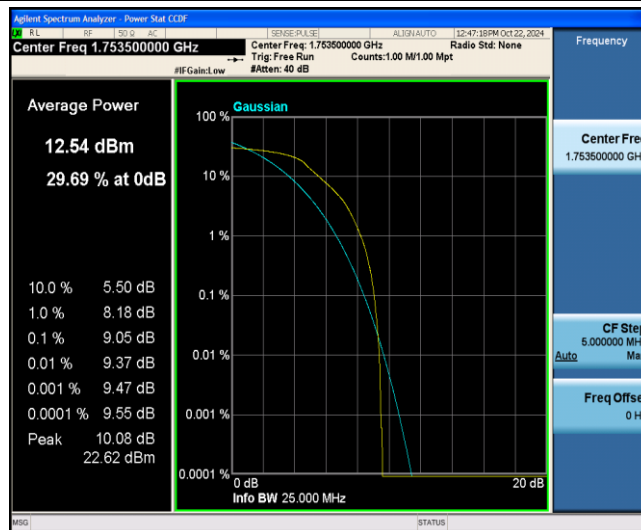
Band4-3MHz-QPSK-20385-6-0-Low-9.05-&lt;=13-PASS
