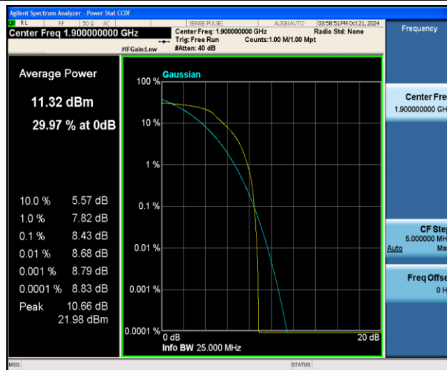
Band2-20MHz-16QAM-19100-6-0-Low-8.43-≤13-PASS
