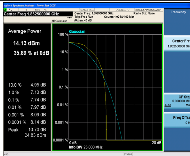
Band2-5MHz-QPSK-18625-6-0-Low-7.74-&lt;=13-PASS
