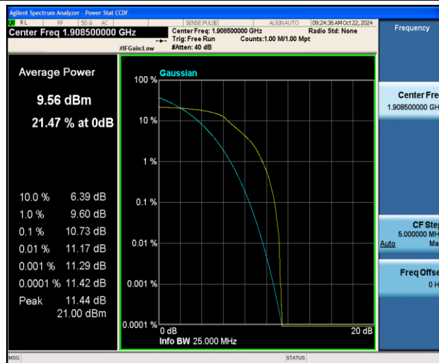
Band2-3MHz-16QAM-19185-6-0-Low-10.73-&lt;=13-PASS
