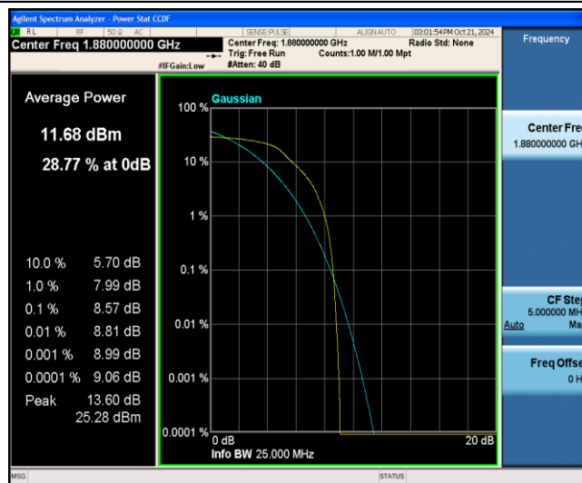
Band2-15MHz-16QAM-18900-6-0-Low-8.57-=&lt;=13-PASS
