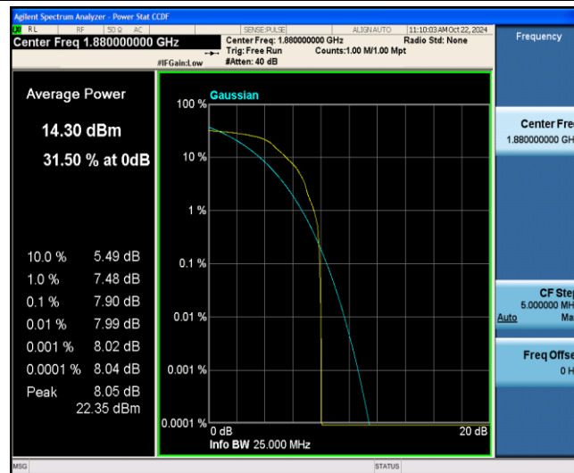
Band2-15MHz-QPSK-18900-1-0-Low-7.90-&lt;=13-PASS
