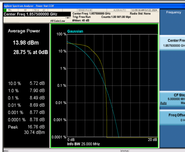
Band2-15MHz-QPSK-18675-6-0-Low-8.49-&lt;=13-PASS
