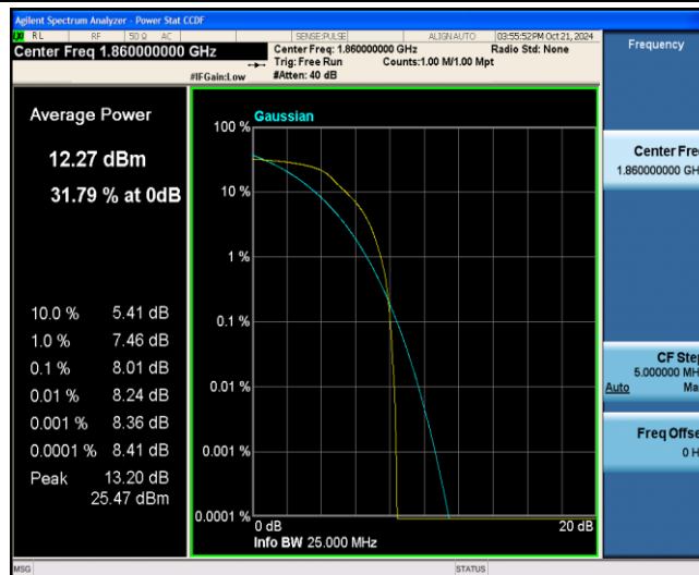
Band2-20MHz-16QAM-18700-6-0-Low-8.01-&lt;=13-PASS
