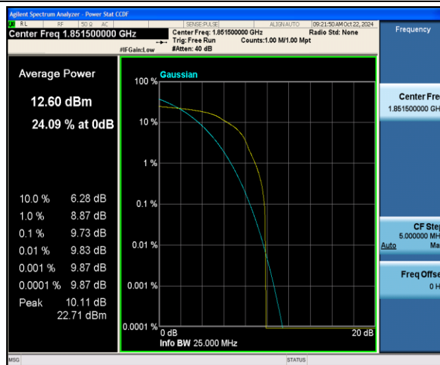
Band2-3MHz-16QAM-18615-1-0-Low-9.73-&lt;=13-PASS
