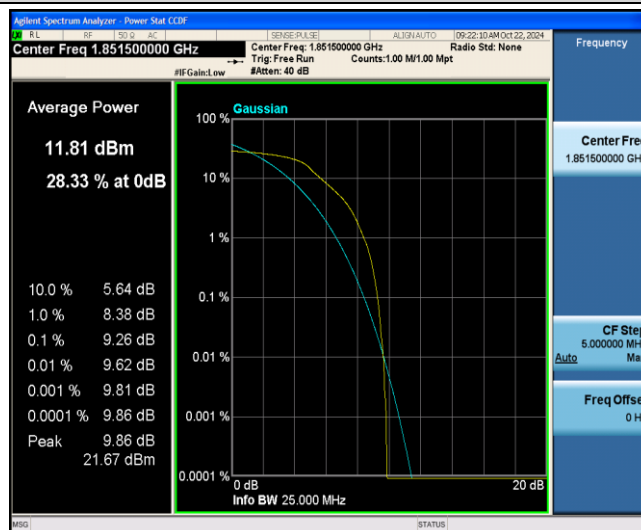
Band2-3MHz-16QAM-18615-6-0-Low-9.26-&lt;=13-PASS
