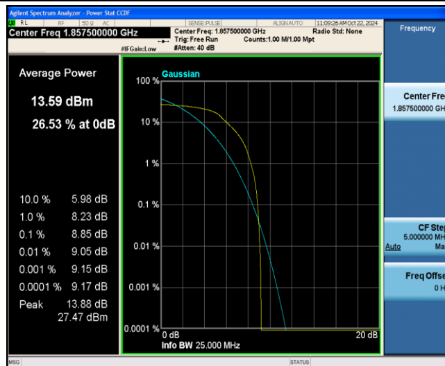
Band2-15MHz-16QAM-18675-6-0-Low-8.85-=&lt;=13-PASS
