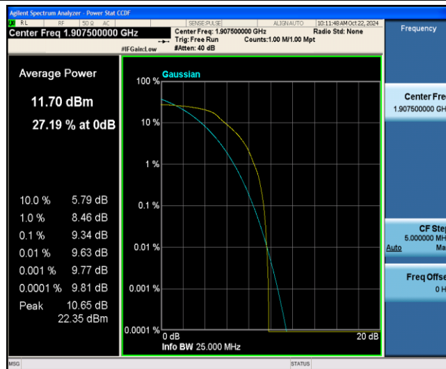
Band2-5MHz-16QAM-19175-6-0-Low-9.34-&lt;=13-PASS
