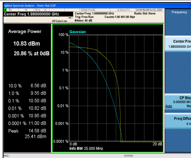
Band2-5MHz-QPSK-18900-6-0-Low-10.50-&lt;=13-PASS
