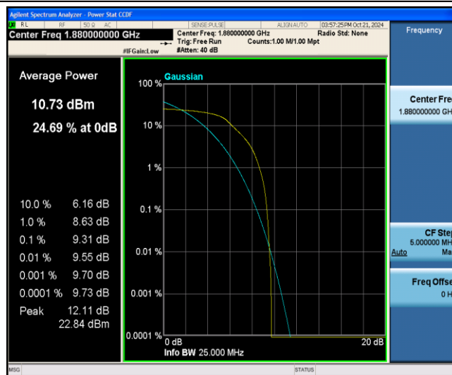
Band2-20MHz-16QAM-18900-6-0-Low-9.31-&lt;=13-PASS
