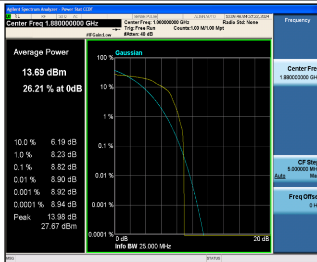
Band2-5MHz-16QAM-18900-1-0-Low-8.82-13-PASS
