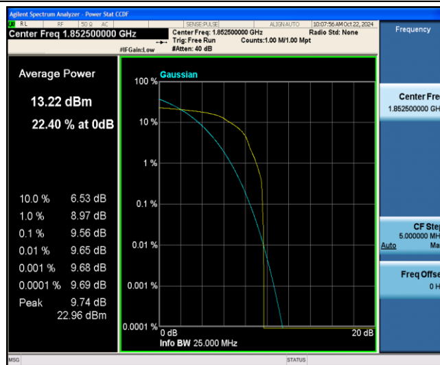
Band2-5MHz-16QAM-18625-1-0-Low-9.56-13-PASS
