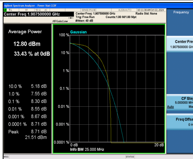
Band2-5MHz-QPSK-19175-6-0-Low-8.30-13-PASS
