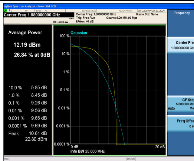
Band2-5MHz-16QAM-18900-6-0-Low-9.26-13-PASS
