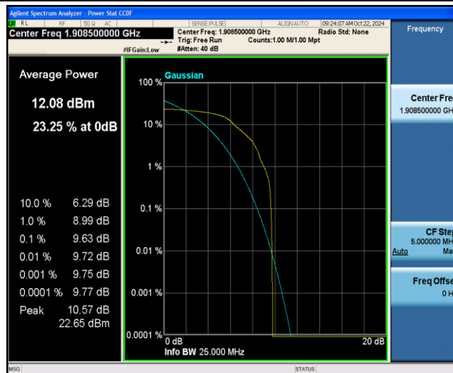
Band2-3MHz-QPSK-19185-1-0-Low-9.63-&lt;=13-PASS
