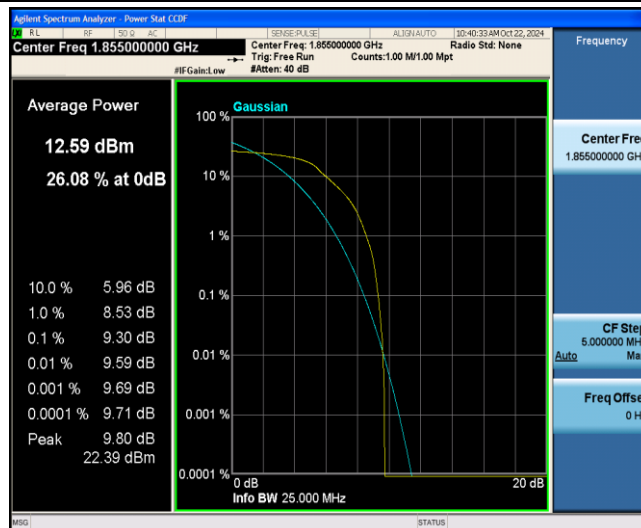
Band2-10MHz-16QAM-18650-6-0-Low-9.30-&lt;=13-PASS
