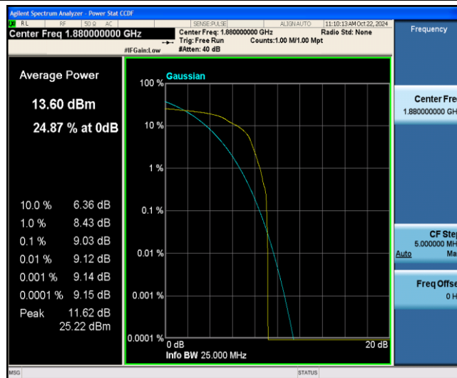
Band2-15MHz-16QAM-18900-1-0-Low-9.03-=&lt;=13-PASS
