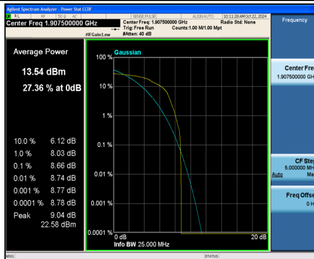
Band2-5MHz-16QAM-19175-1-0-Low-8.66-13-PASS
