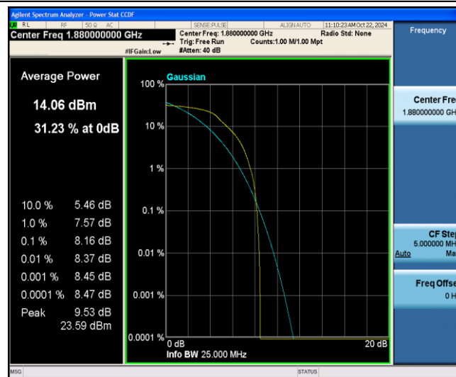
Band2-15MHz-QPSK-18900-6-0-Low-8.16-&lt;=13-PASS
