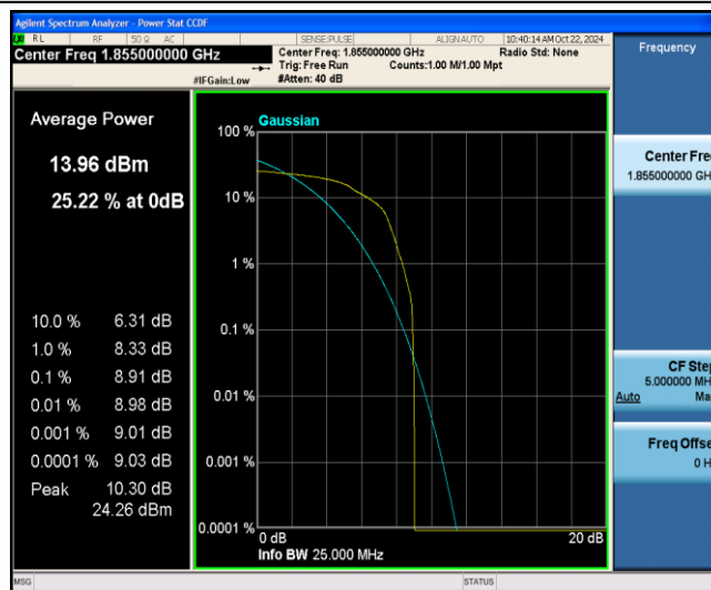
Band2-10MHz-16QAM-18650-1-0-Low-8.91-&lt;=13-PASS
