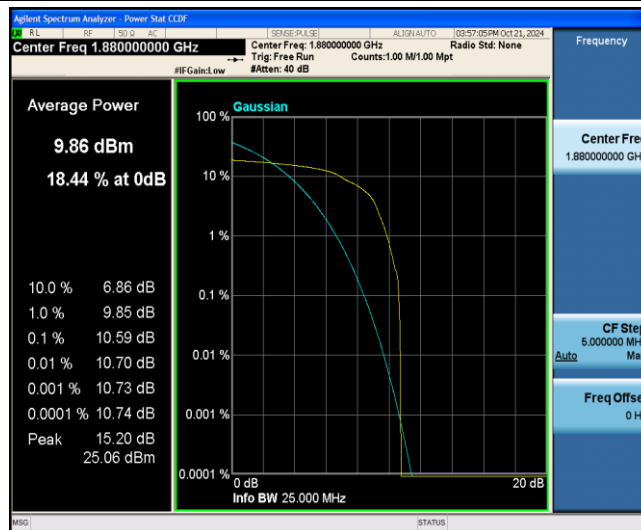
Band2-20MHz-16QAM-18900-1-0-Low-10.59-&lt;=13-PASS
