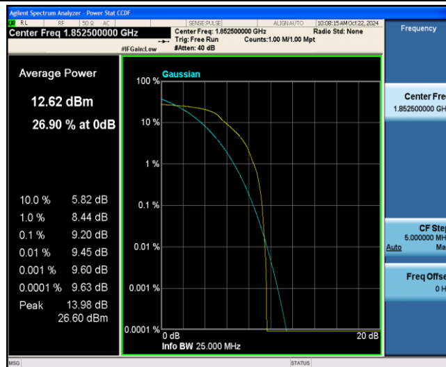
Band2-5MHz-16QAM-18625-6-0-Low-9.20-13-PASS
