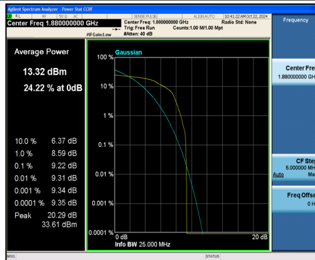
Band2-10MHz-16QAM-18900-1-0-Low-9.22-=&lt;=13-PASS
