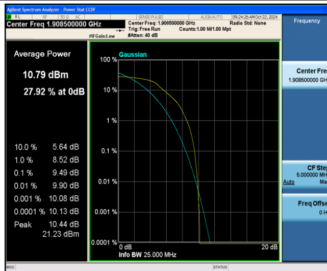
Band2-3MHz-QPSK-19185-6-0-Low-9.49-&lt;=13-PASS
