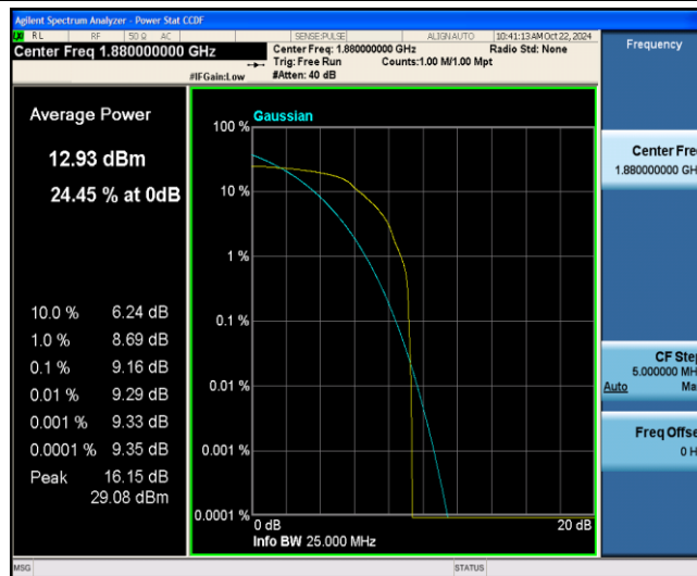
Band2-10MHz-QPSK-18900-1-0-Low-9.16-&lt;=13-PASS
