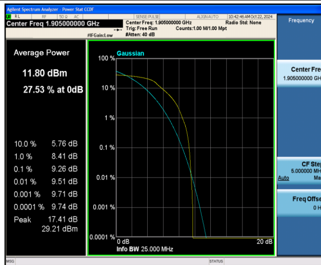
Band2-10MHz-16QAM-19150-6-0-Low-9.26-&lt;=13-PASS
