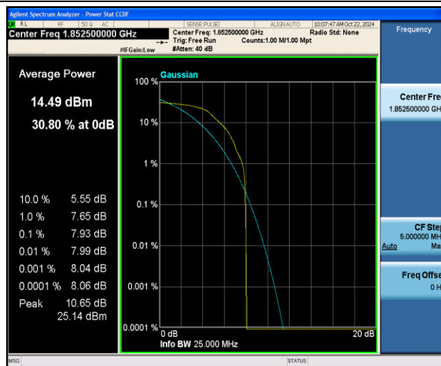
Band2-5MHz-QPSK-18625-1-0-Low-7.93-&lt;=13-PASS
