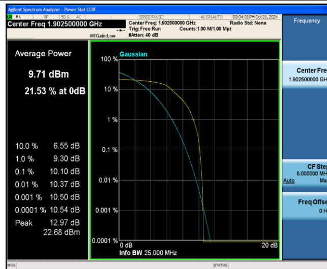
Band2-15MHz-16QAM-19125-6-0-Low-10.10-&lt;=13-PASS
