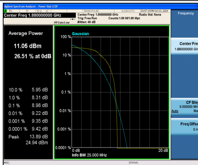
Band2-20MHz-QPSK-18900-6-0-Low-8.98-&lt;=13-PASS
