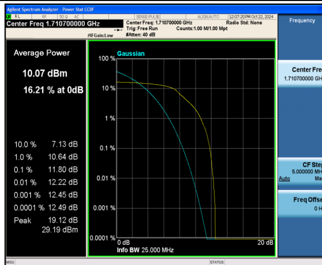
Band4-1.4MHz-QPSK-19957-6-0-Low-11.80-≤13-PASS
