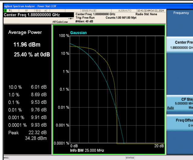
Band2-10MHz-QPSK-18900-6-0-Low-9.53-&lt;=13-PASS
