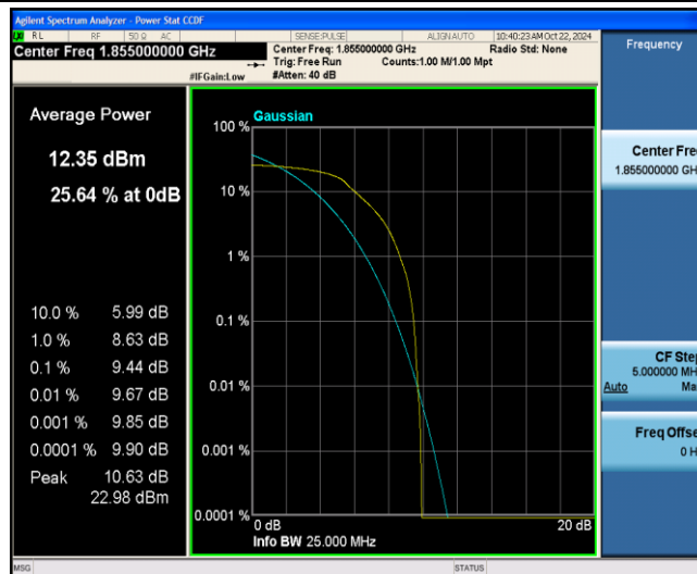
Band2-10MHz-QPSK-18650-6-0-Low-9.44-&lt;=13-PASS
