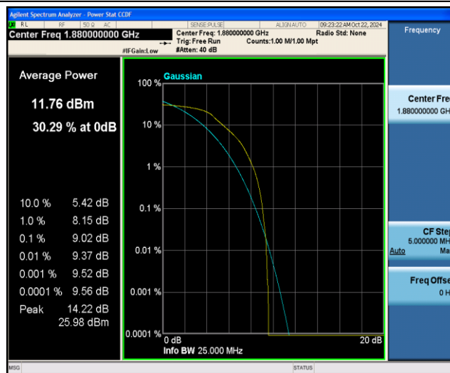
Band2-3MHz-16QAM-18900-6-0-Low-9.02-&lt;=13-PASS
