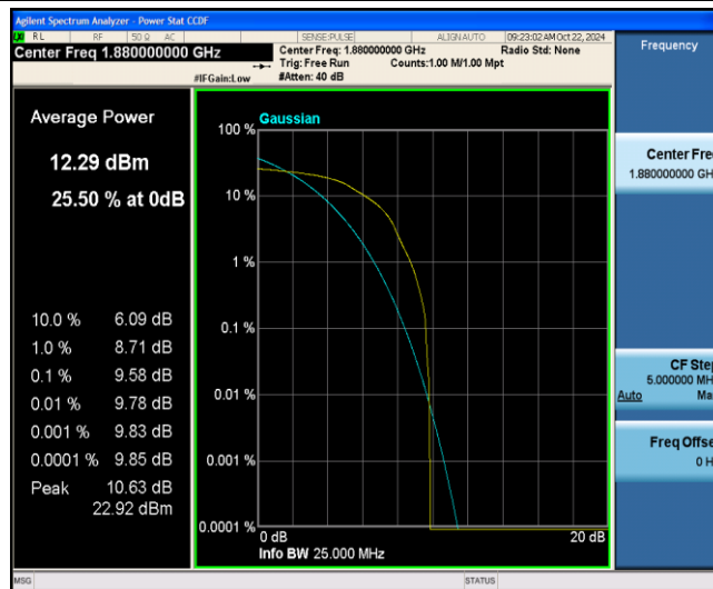
Band2-3MHz-16QAM-18900-1-0-Low-9.58-&lt;=13-PASS
