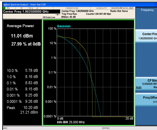
Band2-15MHz-QPSK-19125-6-0-Low-8.83-=&lt;=13-PASS
