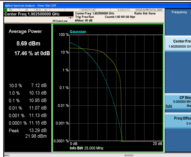
Band2-15MHz-QPSK-19125-1-0-Low-10.95-&lt;=13-PASS
