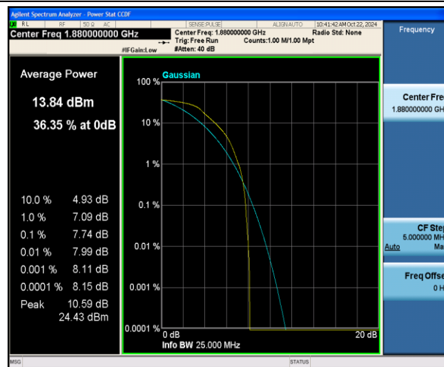
Band2-10MHz-16QAM-18900-6-0-Low-7.74-=&lt;=13-PASS
