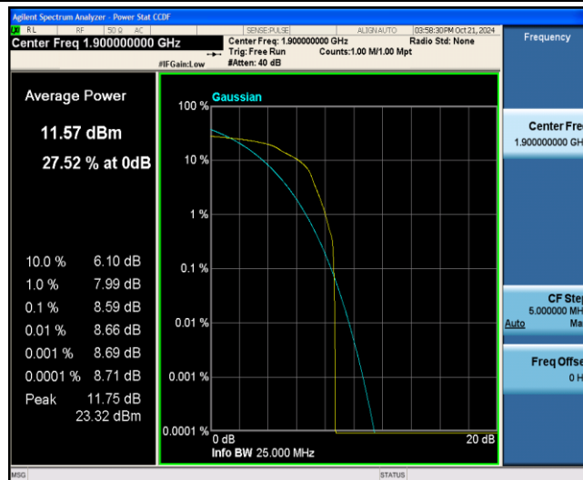
Band2-20MHz-16QAM-19100-1-0-Low-8.59-&lt;=13-PASS
