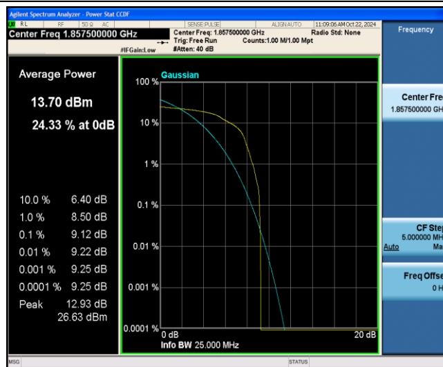
Band2-15MHz-16QAM-18675-1-0-Low-9.12-=&lt;=13-PASS
