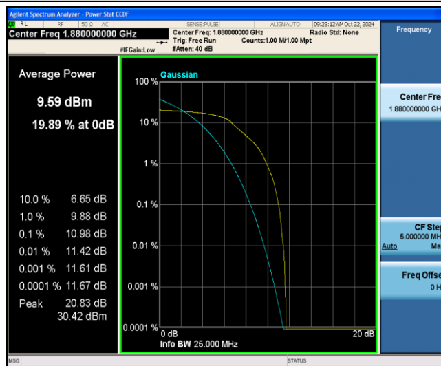
Band2-3MHz-QPSK-18900-6-0-Low-10.98-&lt;=13-PASS
