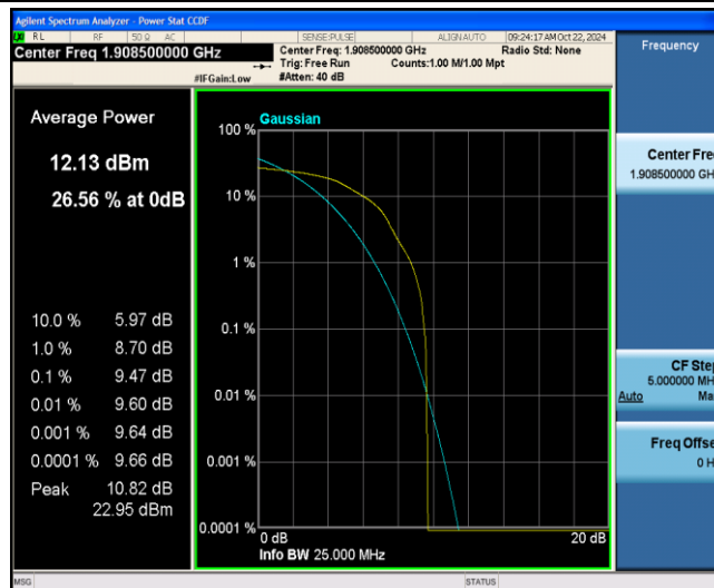
Band2-3MHz-16QAM-19185-1-0-Low-9.47-&lt;=13-PASS
