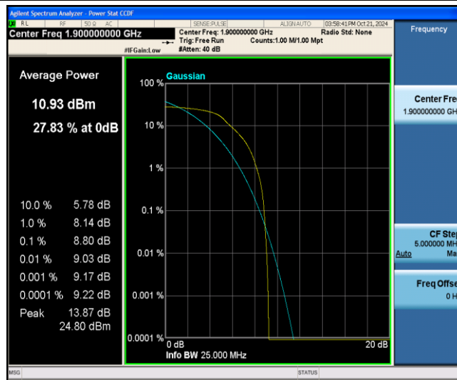
Band2-20MHz-QPSK-19100-6-0-Low-8.80-&lt;=13-PASS
