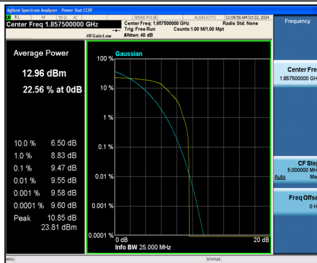
Band2-15MHz-QPSK-18675-1-0-Low-9.47-&lt;=13-PASS
