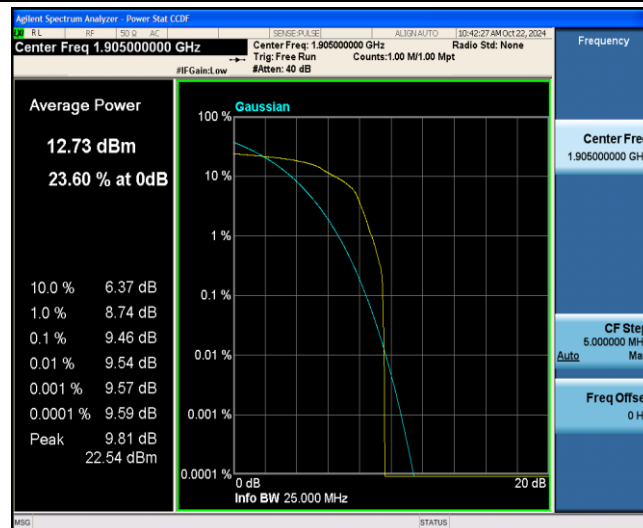
Band2-10MHz-16QAM-19150-1-0-Low-9.46-=&lt;=13-PASS
