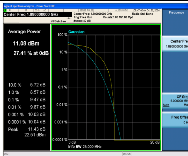
Band2-1.4MHz-QPSK-18900-6-0-Low-9.47-13-PASS
