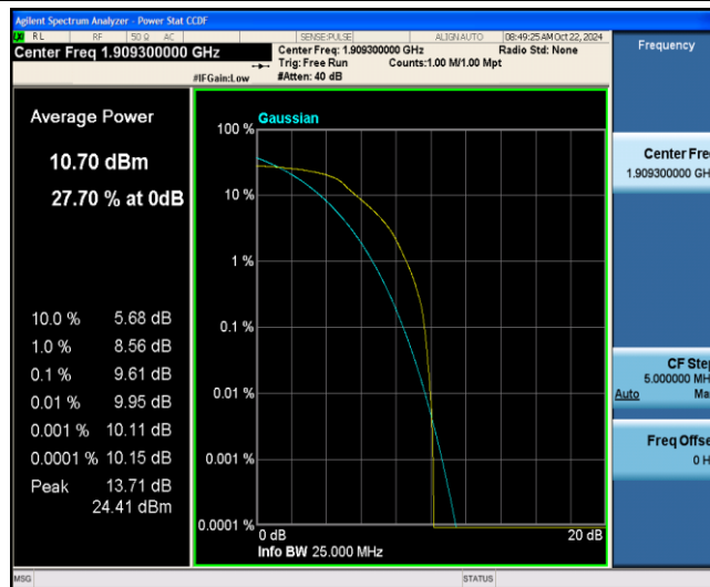
Band2-1.4MHz-QPSK-19193-6-0-Low-9.61-&lt;=13-PASS
