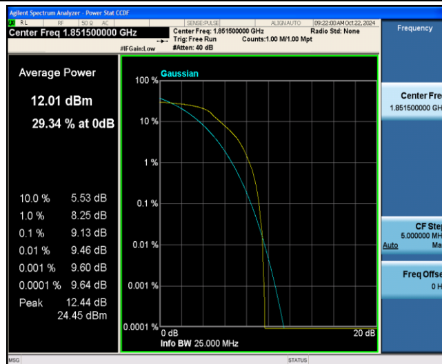
Band2-3MHz-QPSK-18615-6-0-Low-9.13-≤13-PASS
