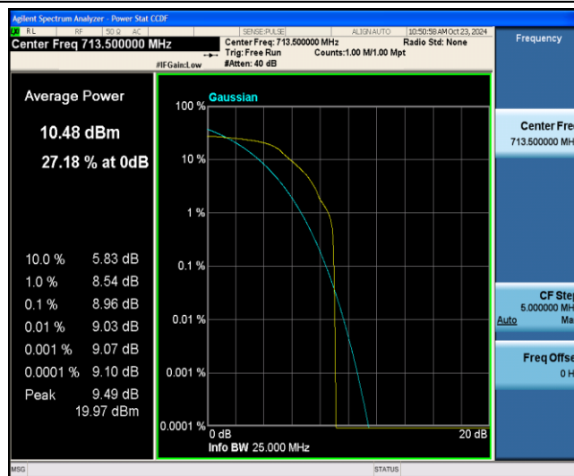
Band12-5MHz-QPSK-23155-1-0-Low-8.96-&lt;=13-PASS
