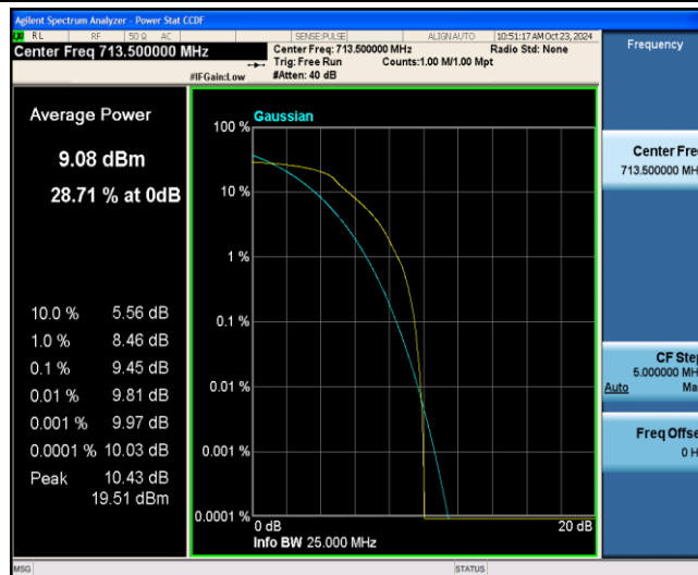
Band12-5MHz-QPSK-23155-6-0-Low-9.45-&lt;=13-PASS
