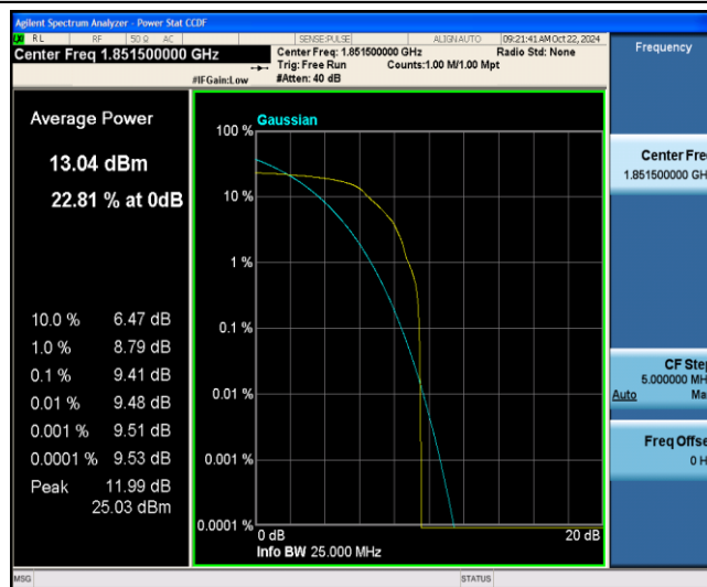
Band2-3MHz-QPSK-18615-1-0-Low-9.41-≤13-PASS
