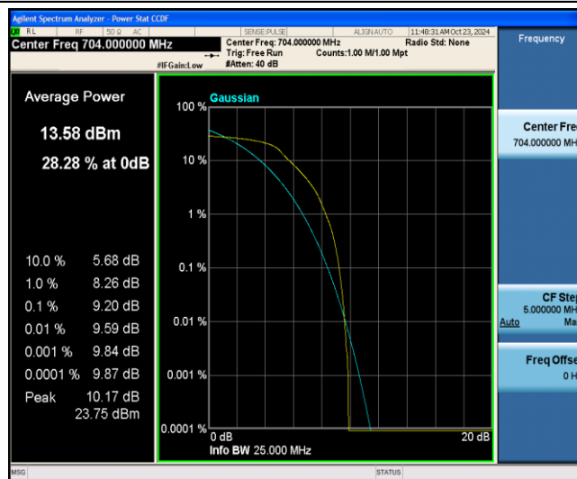
Band12-10MHz-16QAM-23060-6-0-Low-9.20-&lt;=13-PASS
