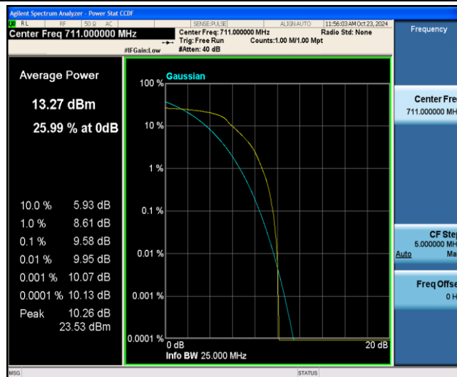
Band12-10MHz-QPSK-23130-6-0-High-9.58-&lt;=13-PASS
