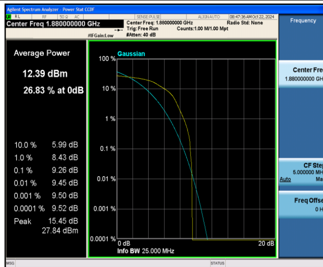
Band2-1.4MHz-16QAM-18900-1-0-Low-9.26-13-PASS
