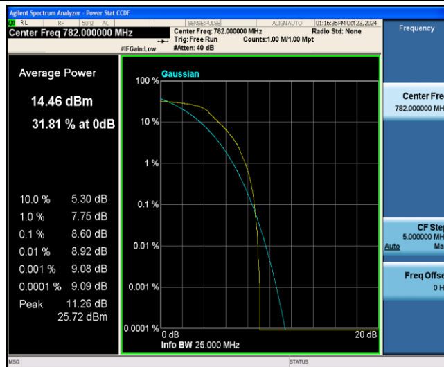
Band13-5MHz-16QAM-23230-6-0-Low-8.60-&lt;=13-PASS
