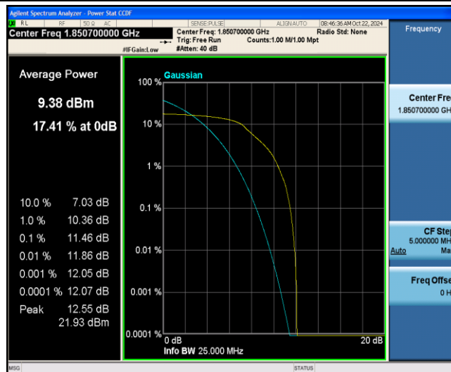
Band2-1.4MHz-16QAM-18607-6-0-Low-11.46-&lt;=13-PASS
