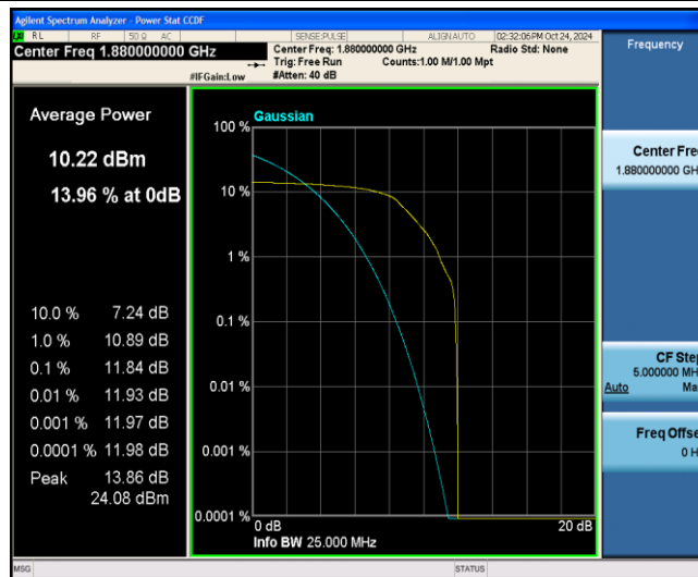
Band2-1.4MHz-QPSK-18900-1-0-Low-11.84-13-PASS
