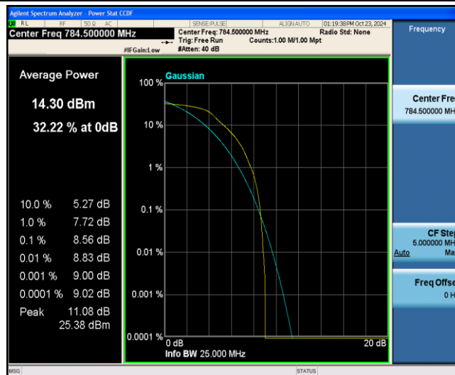
Band13-5MHz-16QAM-23255-6-0-Low-8.56-&lt;=13-PASS
