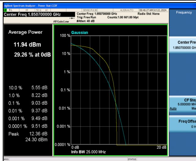
Band2-1.4MHz-QPSK-18607-6-0-Low-9.03-13-PASS
