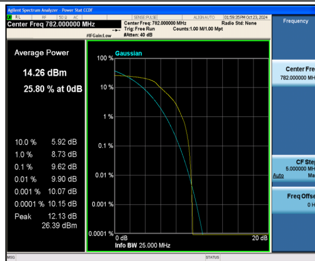
Band13-10MHz-QPSK-23230-6-0-Low-9.62-=&lt;=13-PASS
