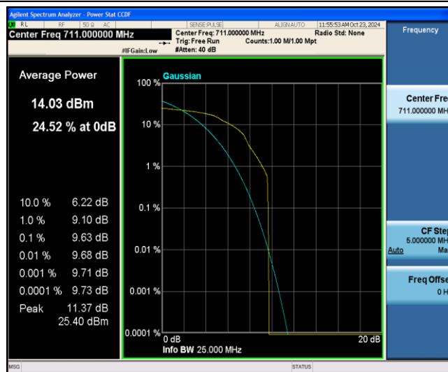
Band12-10MHz-16QAM-23130-1-5-High-9.63-&lt;=13-PASS
