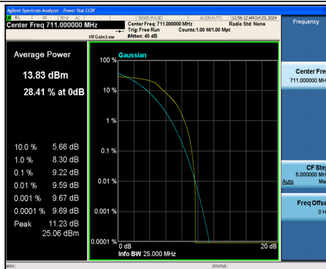
Band12-10MHz-16QAM-23130-6-0-High-9.22-&lt;=13-PASS
