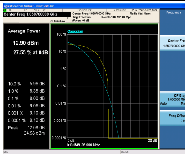
Band2-1.4MHz-16QAM-18607-1-0-Low-9.00-&lt;=13-PASS
