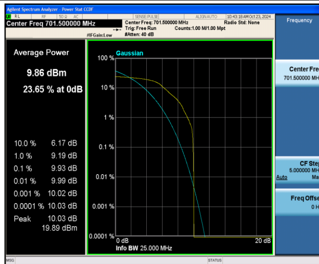
Band12-5MHz-QPSK-23035-1-0-Low-9.93-&lt;=13-PASS
