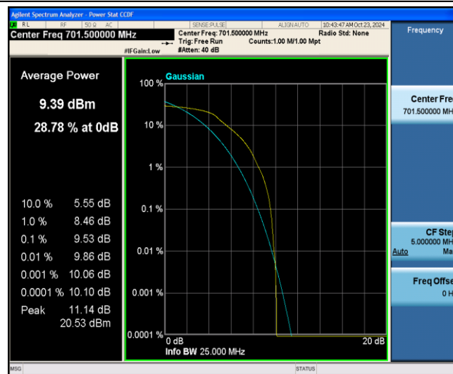
Band12-5MHz-16QAM-23035-6-0-Low-9.53-=&lt;=13-PASS
