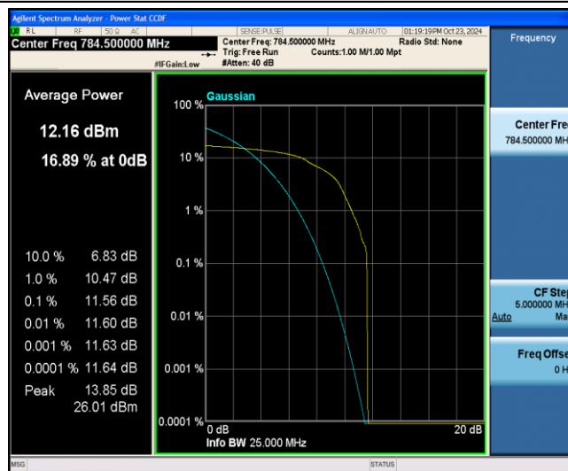
Band13-5MHz-16QAM-23255-1-0-Low-11.56-&lt;=13-PASS
