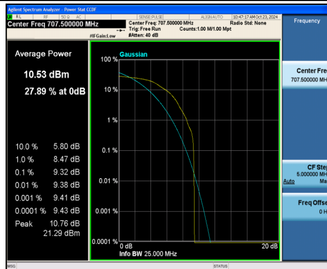
Band12-5MHz-16QAM-23095-1-0-Low-9.32-=&lt;=13-PASS
