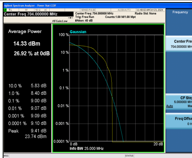
Band12-10MHz-QPSK-23060-1-0-Low-9.00-13-PASS
