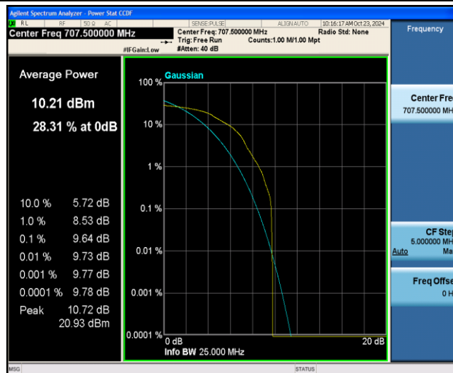
Band12-3MHz-16QAM-23095-1-0-Low-9.64-&lt;=13-PASS
