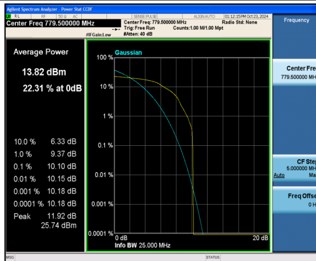
Band13-5MHz-16QAM-23205-1-0-Low-10.10-13-PASS
