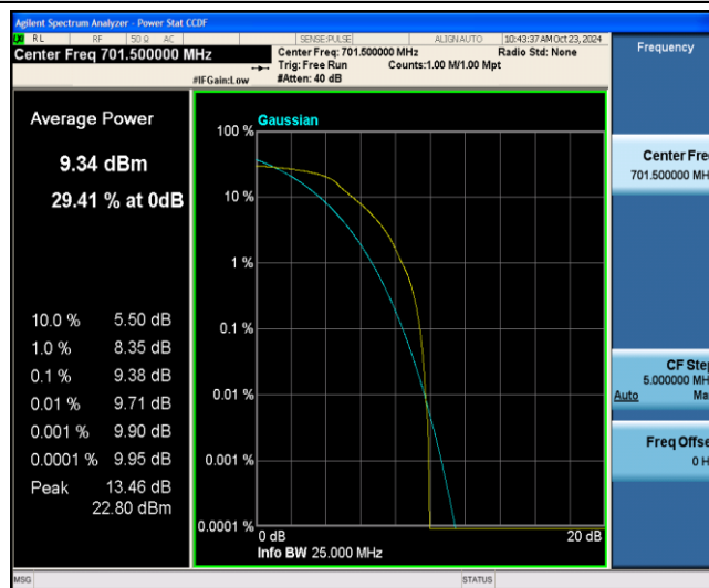
Band12-5MHz-QPSK-23035-6-0-Low-9.38-&lt;=13-PASS
