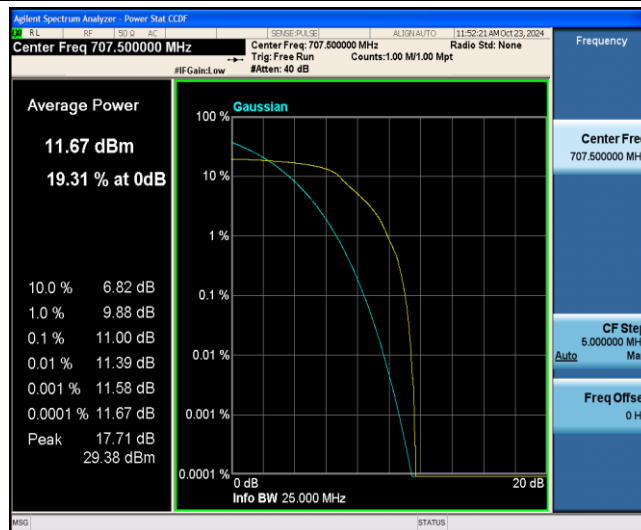
Band12-10MHz-16QAM-23095-6-0-Low-11.00-&lt;=13-PASS
