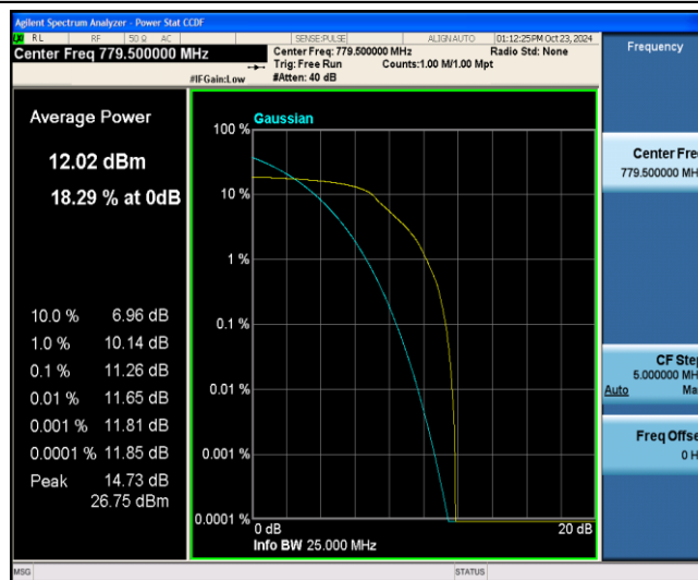
Band13-5MHz-QPSK-23205-6-0-Low-11.26-&lt;=13-PASS
