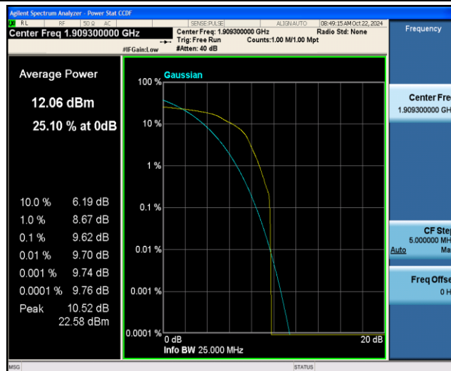
Band2-1.4MHz-16QAM-19193-1-0-Low-9.62-13-PASS
