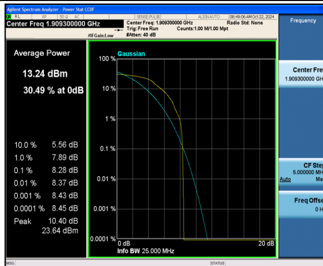
Band2-1.4MHz-QPSK-19193-1-0-Low-8.28-13-PASS
