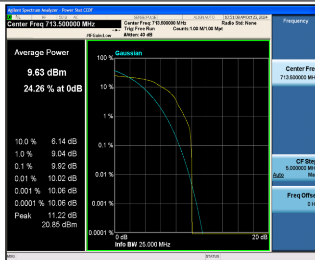
Band12-5MHz-16QAM-23155-1-0-Low-9.92-13-PASS
