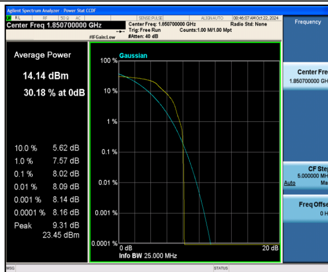
Band2-1.4MHz-QPSK-18607-1-0-Low-8.02-13-PASS
