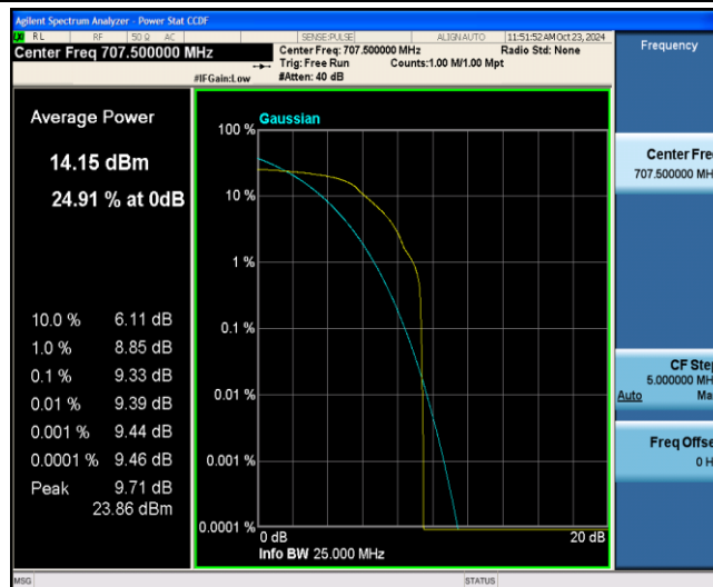
Band12-10MHz-QPSK-23095-1-0-Low-9.33-13-PASS
