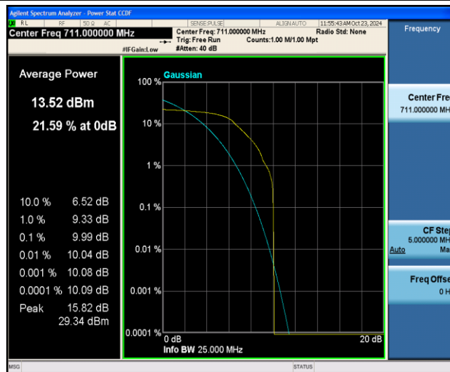
Band12-10MHz-QPSK-23130-1-5-High-9.99-&lt;=13-PASS
