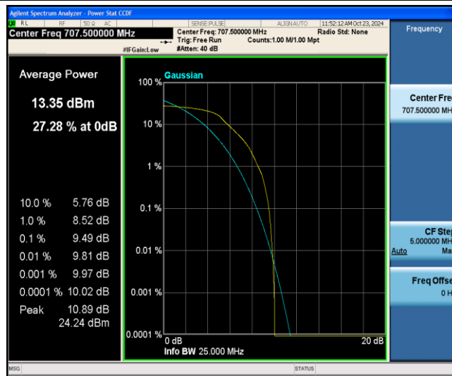
Band12-10MHz-QPSK-23095-6-0-Low-9.49-&lt;=13-PASS
