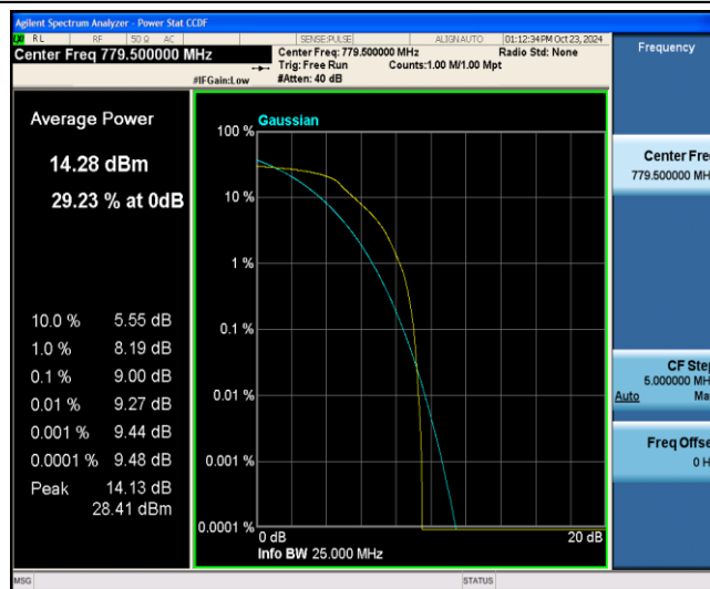
Band13-5MHz-16QAM-23205-6-0-Low-9.00-13-PASS
