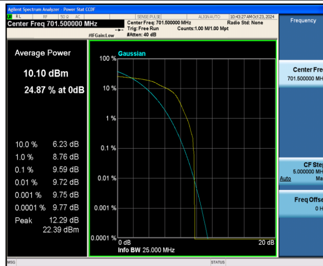
Band12-5MHz-16QAM-23035-1-0-Low-9.59-=&lt;=13-PASS
