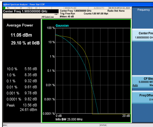
Band2-1.4MHz-16QAM-19193-6-0-Low-9.32-≤13-PASS
