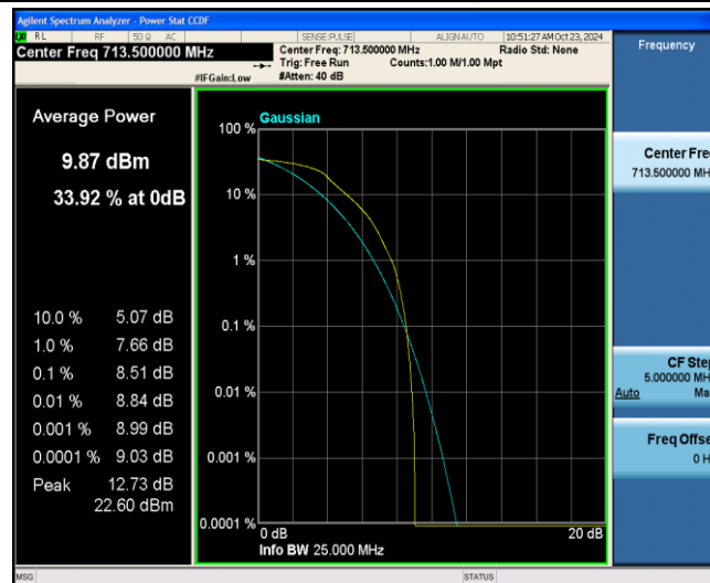
Band12-5MHz-16QAM-23155-6-0-Low-8.51-13-PASS
