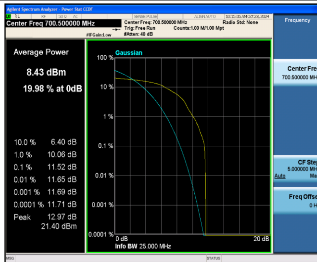
Band12-3MHz-16QAM-23025-1-0-Low-11.52-&lt;=13-PASS
