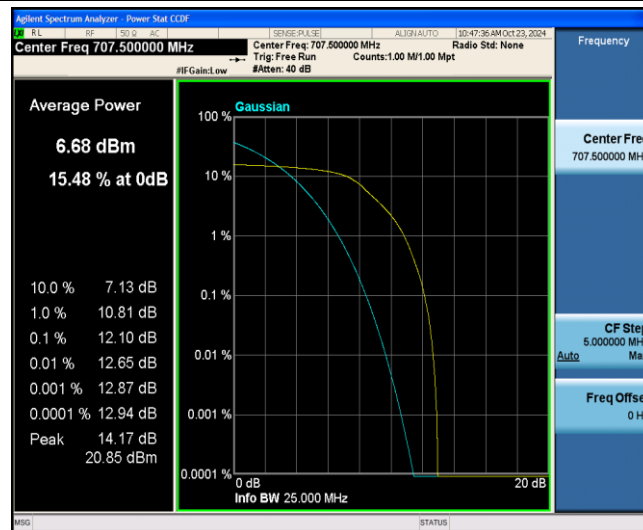
Band12-5MHz-16QAM-23095-6-0-Low-12.10-13-PASS
