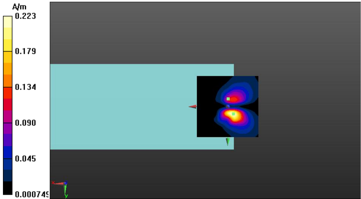
Fig A.10 T-Coil LTE-Band 17-Y
