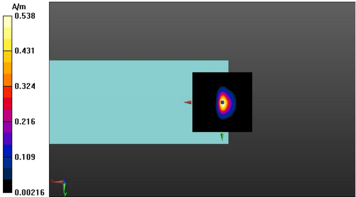
Fig A.12 T-Coil LTE-Band 26-Z
