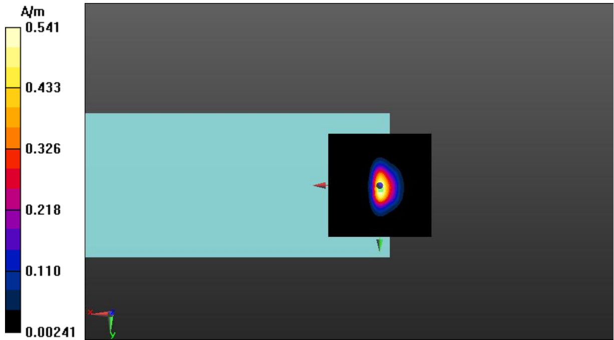
Fig A.11 T-Coil LTE-Band 25-Z
