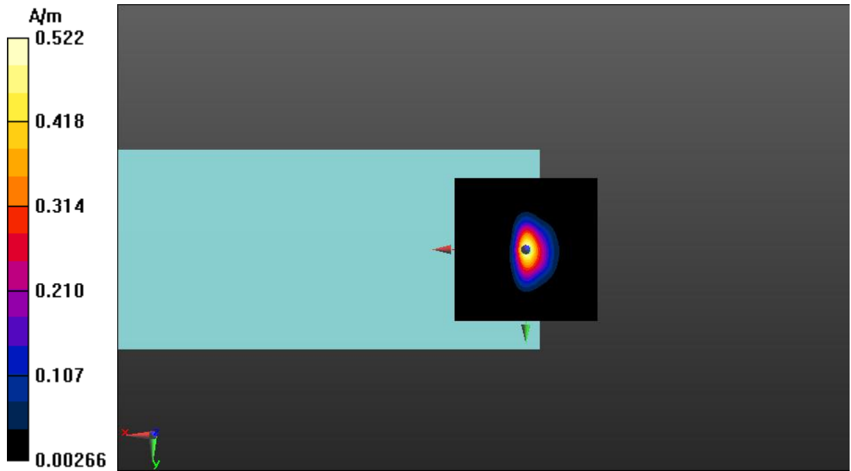
Fig A.10 T-Coil LTE-Band 17-Z
