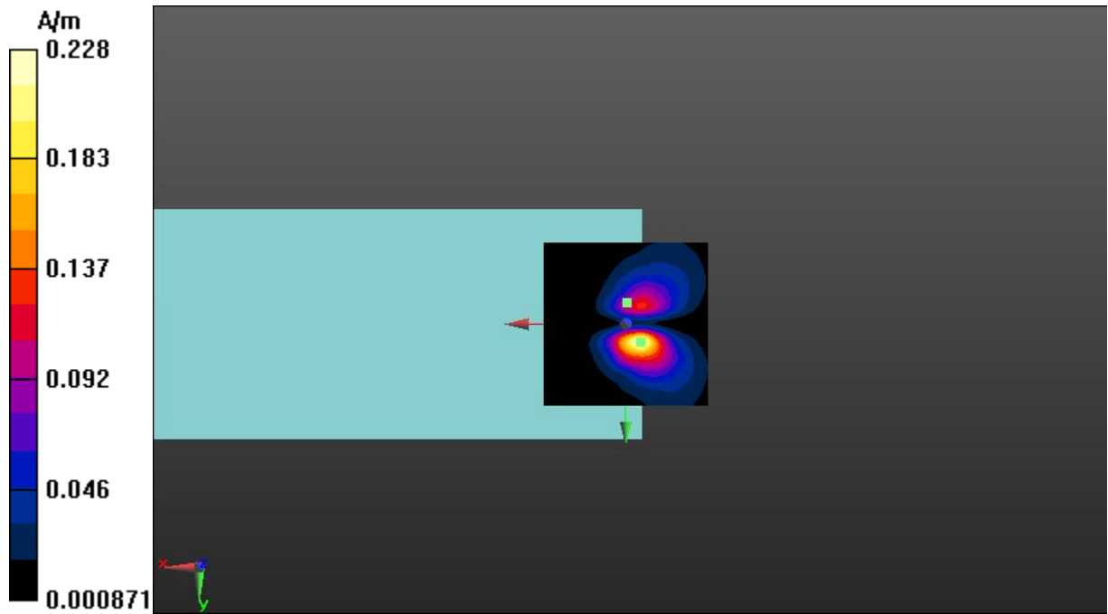
Fig A.11 T-Coil LTE-Band 25-Y
