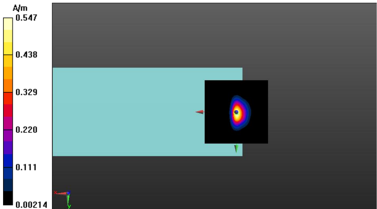
Fig A.13 T-Coil LTE-Band 66-Z
