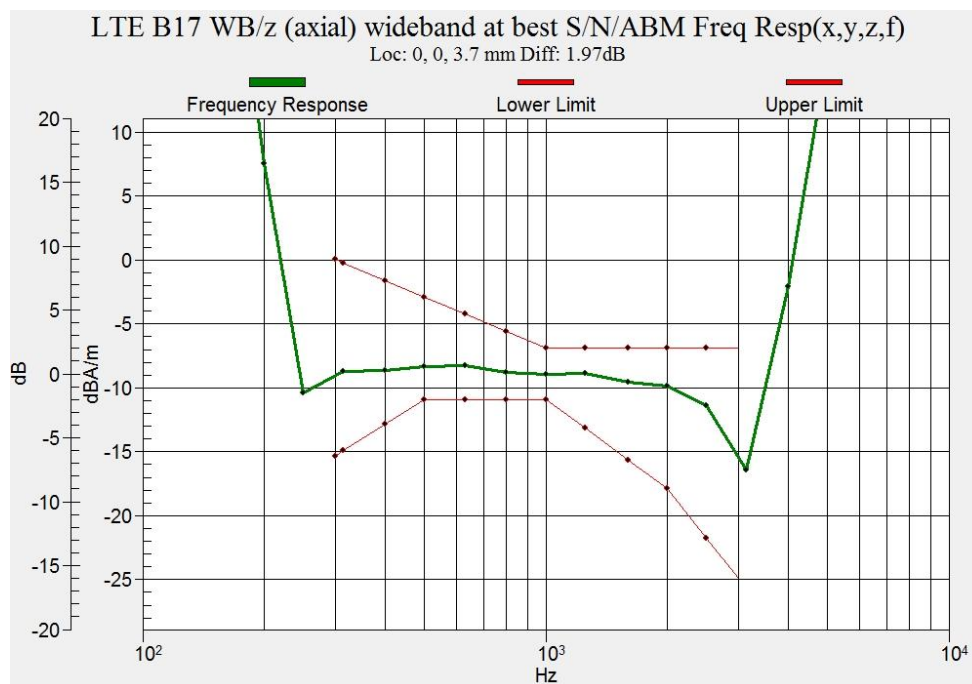
Figure B.10 Frequency Response of LTE Band 17
