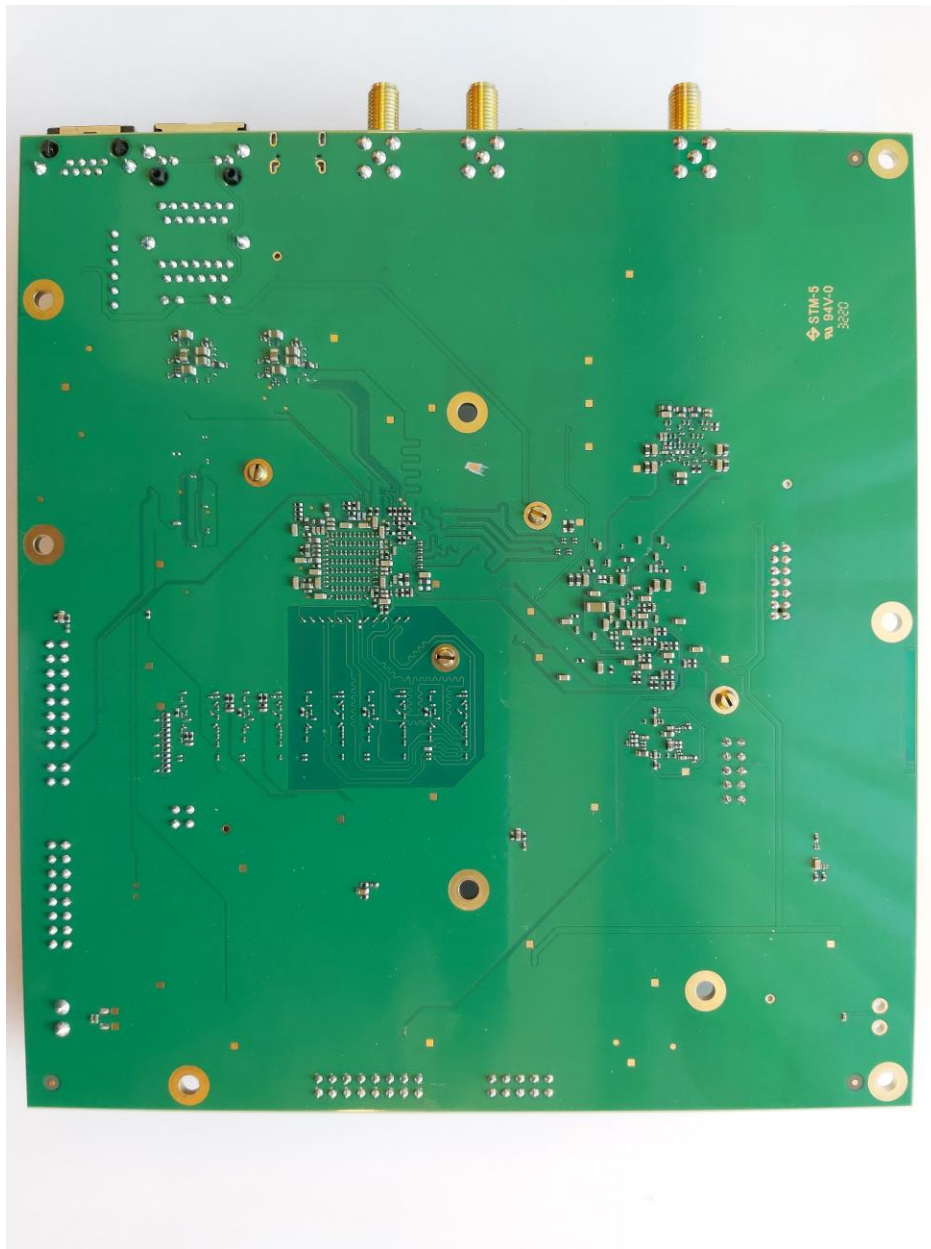
Main board underneath
