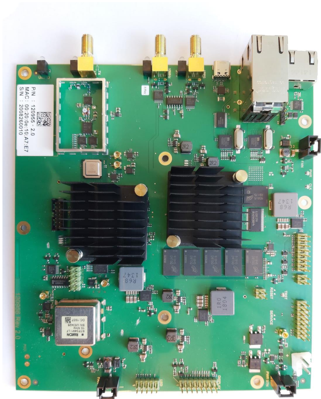
Main board – topside
