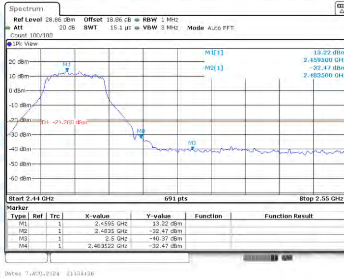
11AX20SISO_Ant1_High_2462_Peak
