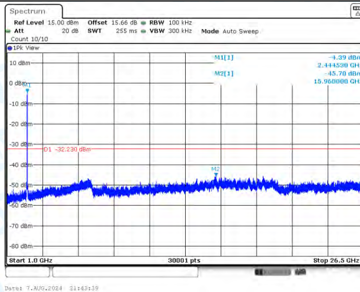
11AX40SISO_Ant1_2437_1000~26500
