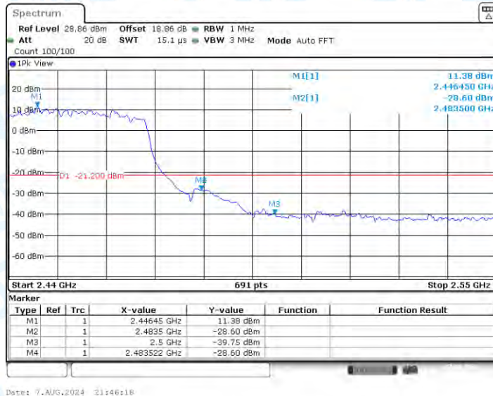
11AX40SISO_Ant1_High_2452_Peak
