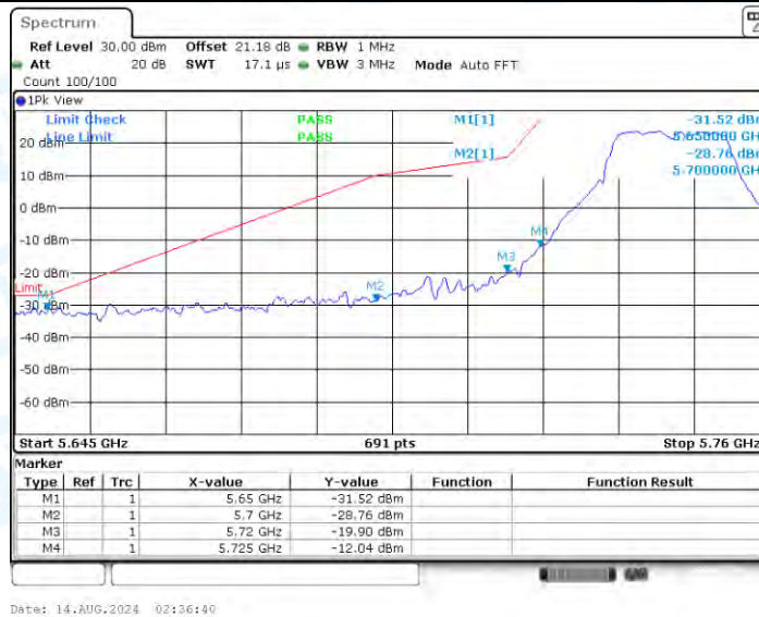
11N20SISO_Ant1_Low_5745_Peak
