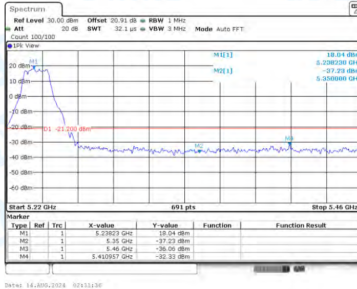
11N20SISO_Ant1_High_5240_Peak
