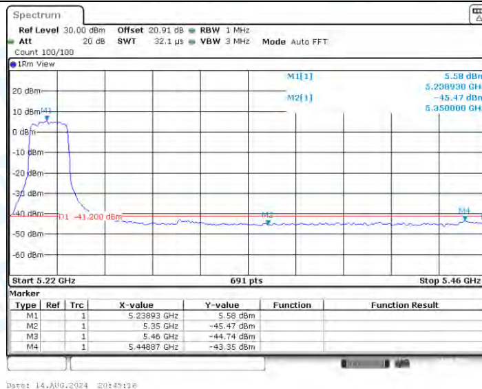
11AX20SISO_Ant1_High_5240_AV
