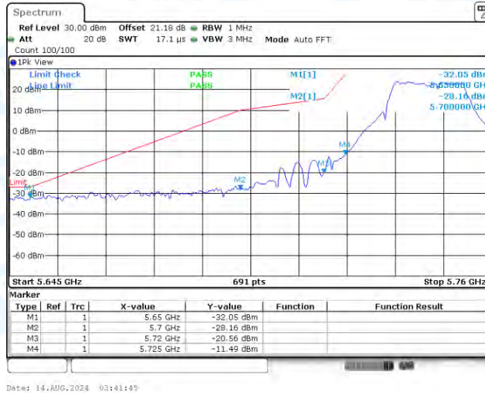
11AC20SISO_Ant1_Low_5745_Peak
