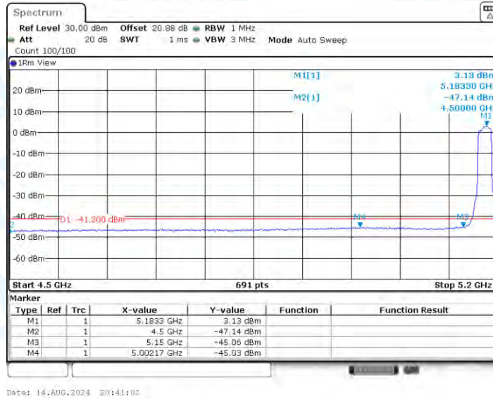
11AX20SISO_Ant1_Low_5180_AV
