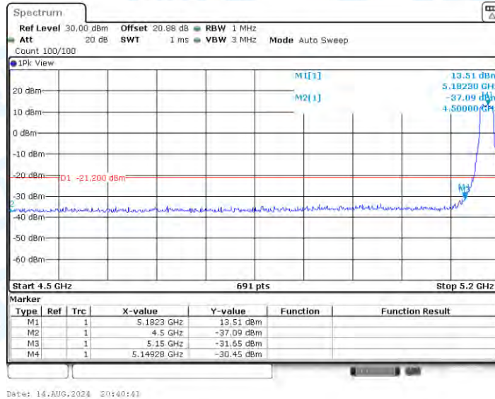
11AX20SISO_Ant1_Low_5180_Peak
