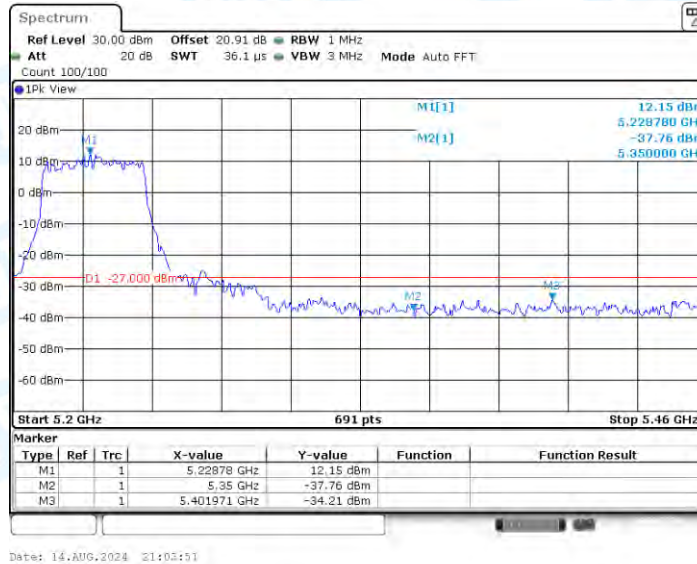
11AX40SISO_Ant1_High_5230
