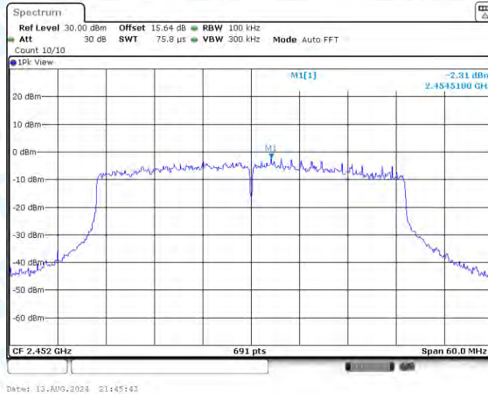
11AX40SISO_Ant1_2452_0~Reference
