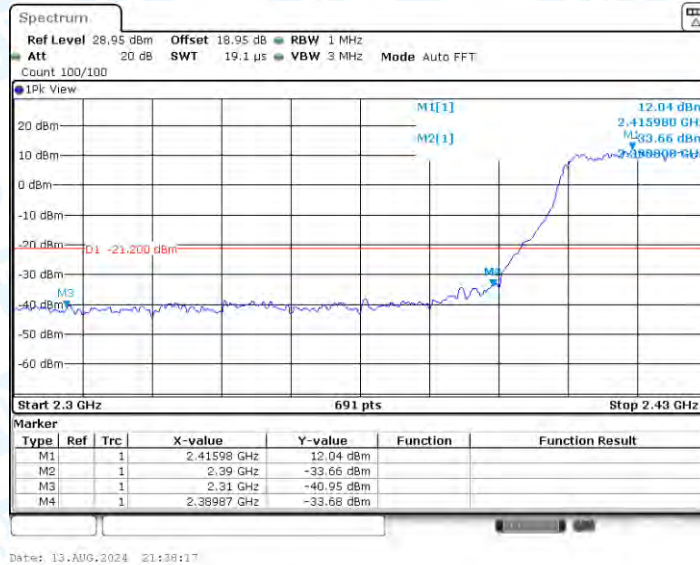
11AX40SISO_Ant1_Low_2422_Peak
