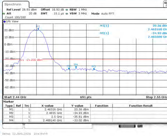
11B_Ant1_High_2462_Peak
