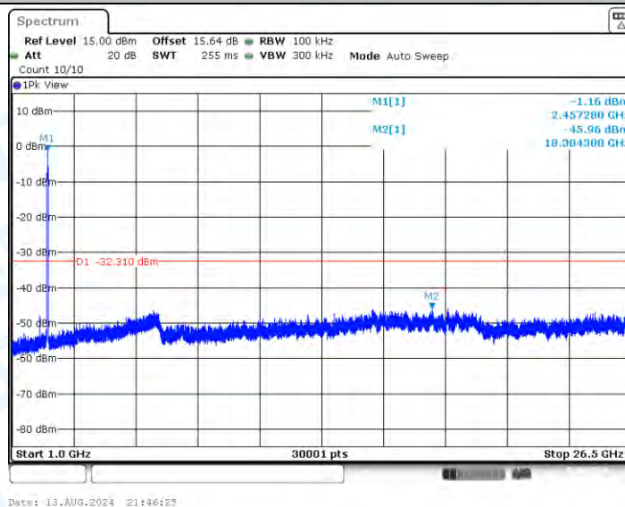
11AX40SISO_Ant1_2452_1000~26500
