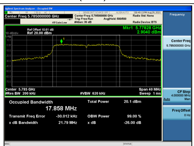
11ac (HT20) CH157
