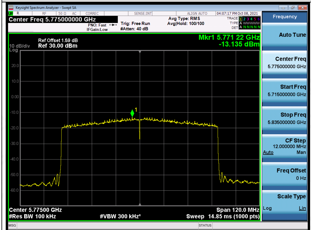
Test_Graph_802.11ax80_ANT2_5775_MCS0_PSD
