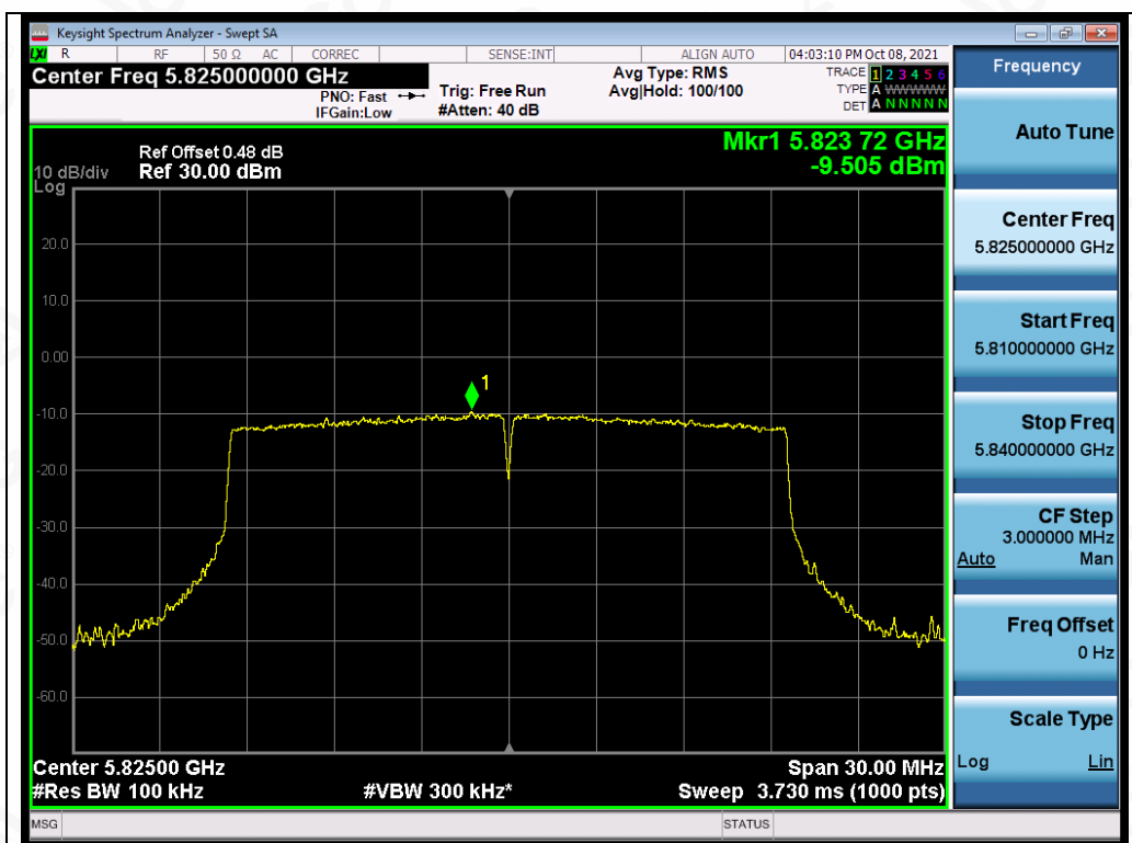
Test_Graph_802.11ax20_ANT2_5825_MCS0_PSD
