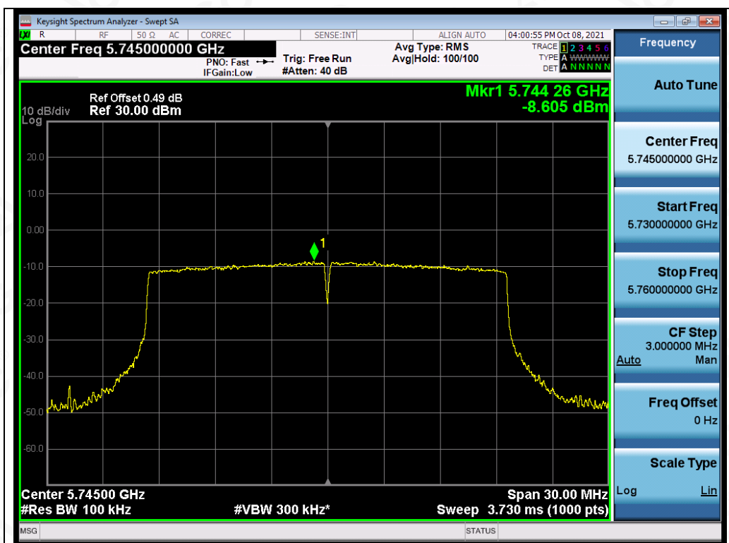
Test_Graph_802.11ax20_ANT2_5745_MCS0_PSD
