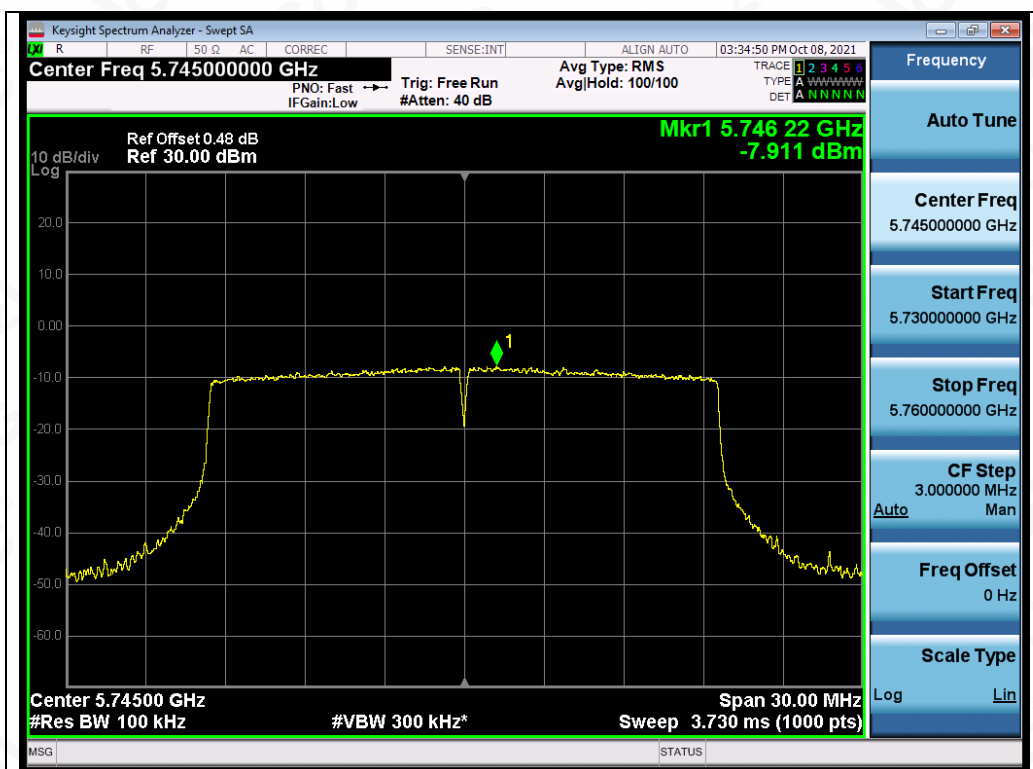
Test_Graph_802.11ax20_ANT1_5745_MCS0_PSD
