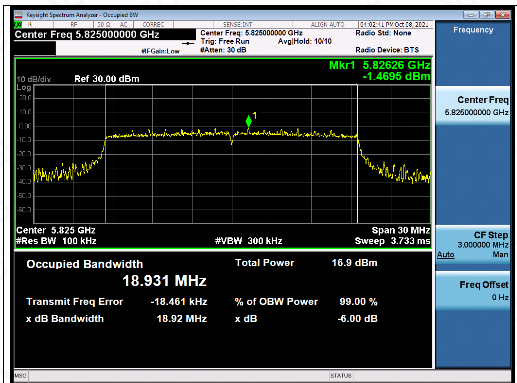
Test_Graph_802.11ax20_ANT2_5825_MCS0_DTSBW
