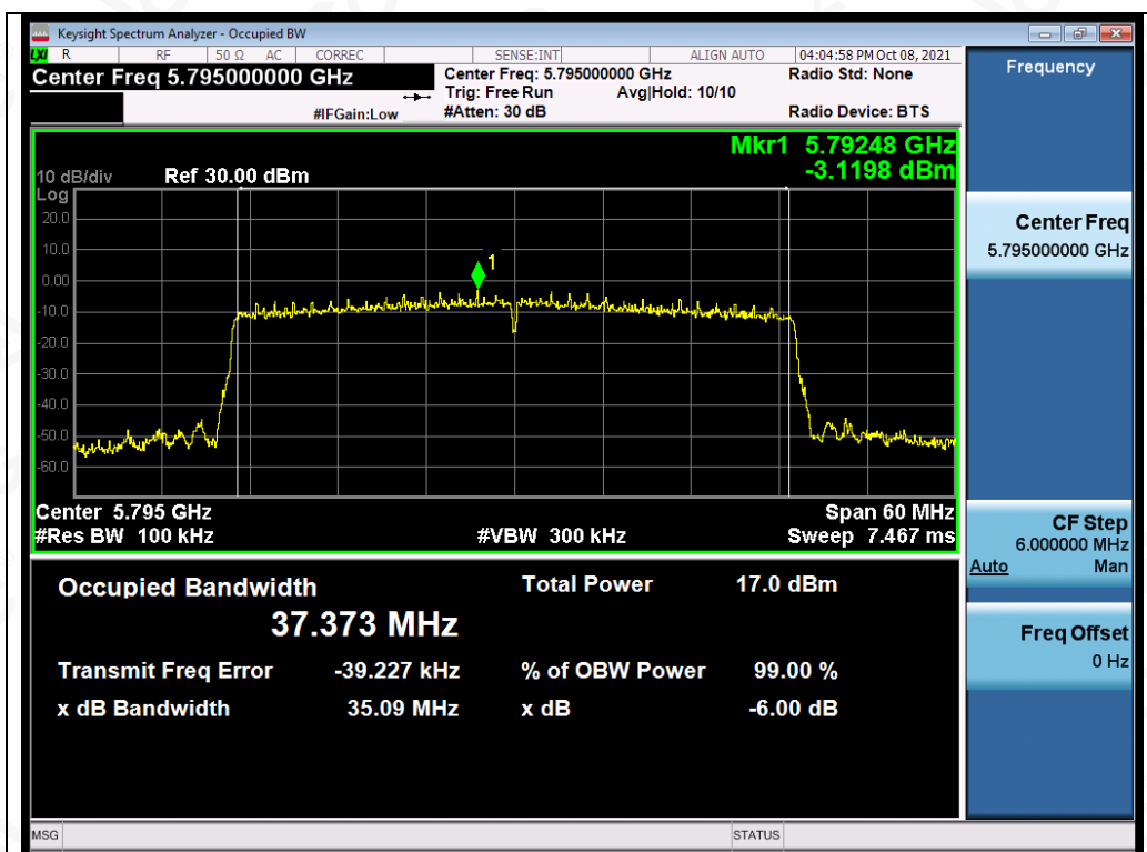
Test_Graph_802.11ax40_ANT2_5795_MCS0_DTSBW
