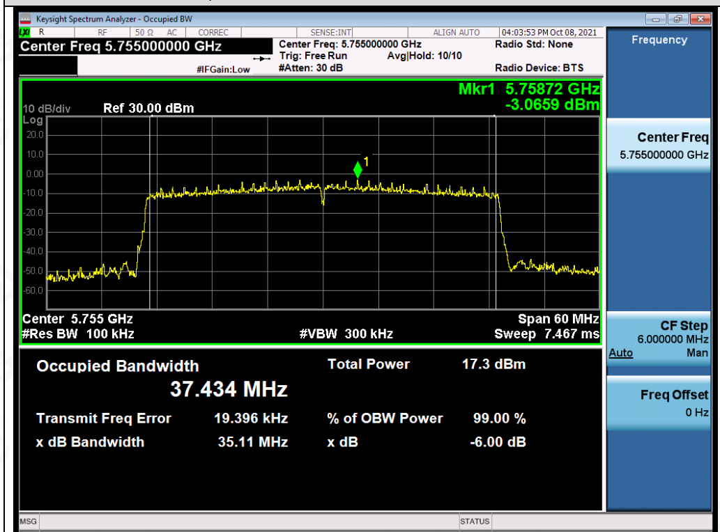
Test_Graph_802.11ax40_ANT2_5755_MCS0_DTSBW
