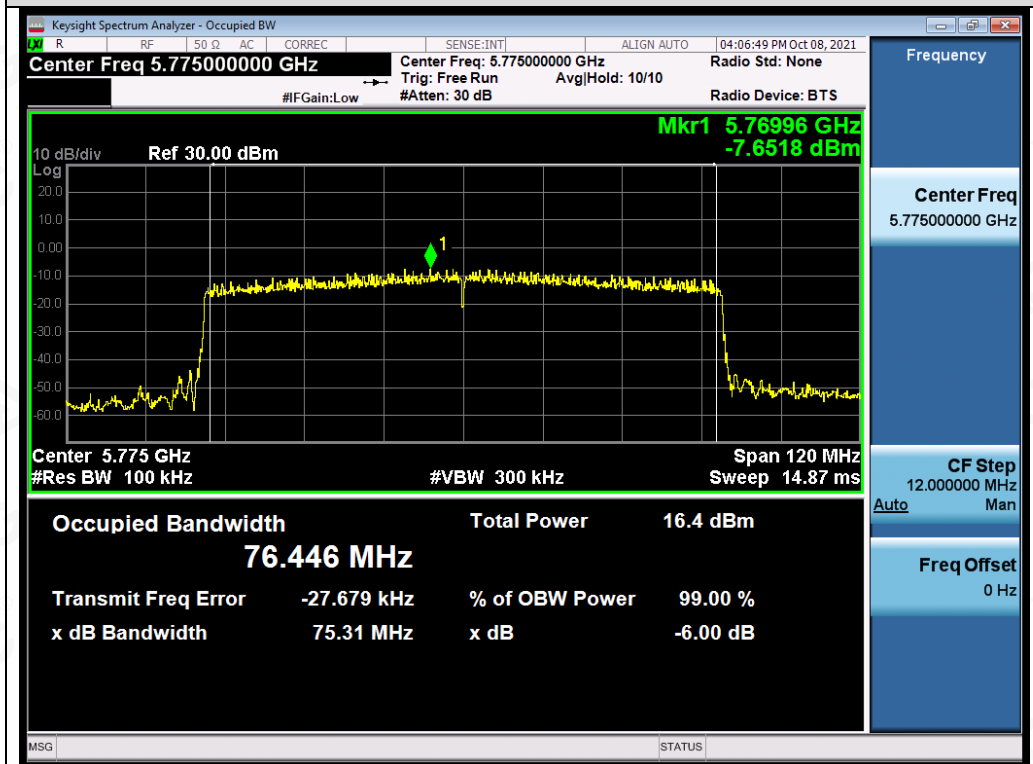
Test_Graph_802.11ax80_ANT2_5775_MCS0_DTSBW
