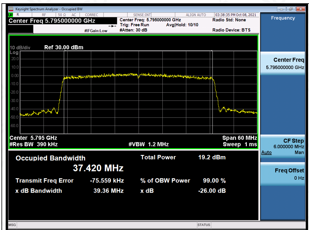
Test_Graph_802.11ax40_ANT1_5795_MCS0_OBW
