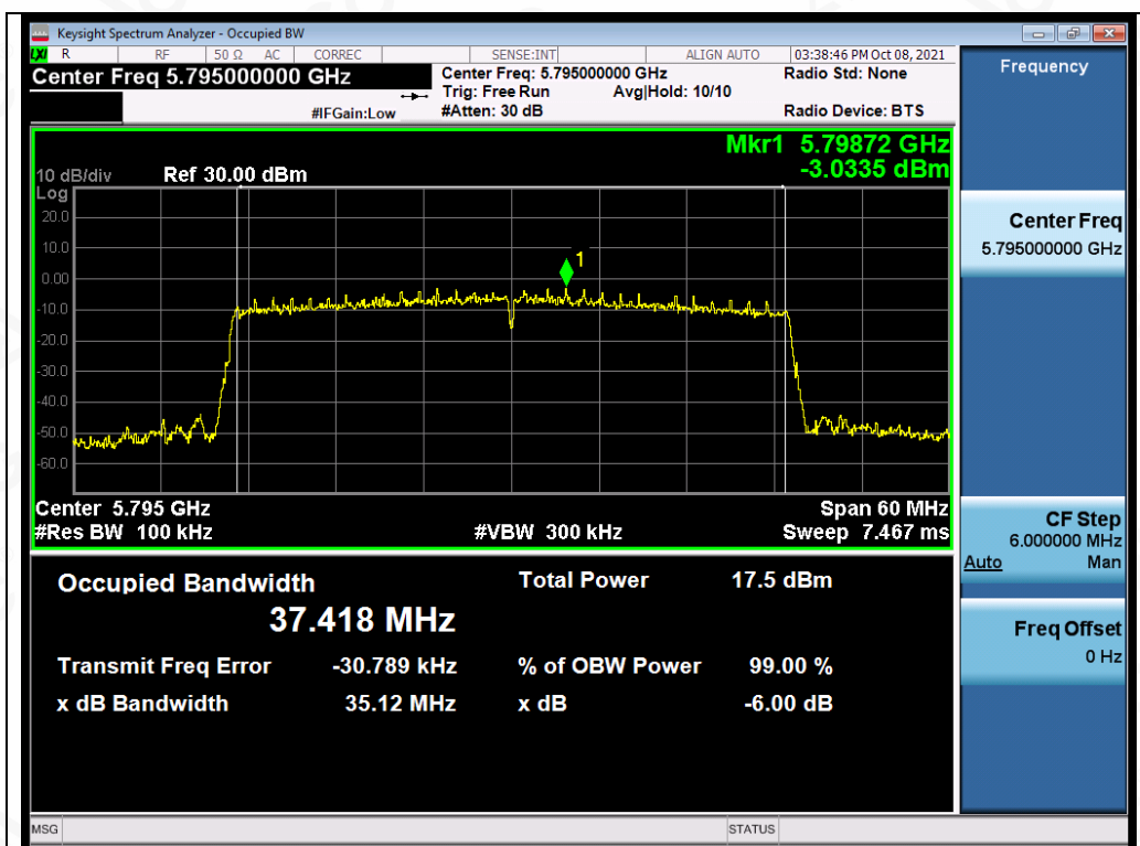
Test_Graph_802.11ax40_ANT1_5795_MCS0_DTSBW
