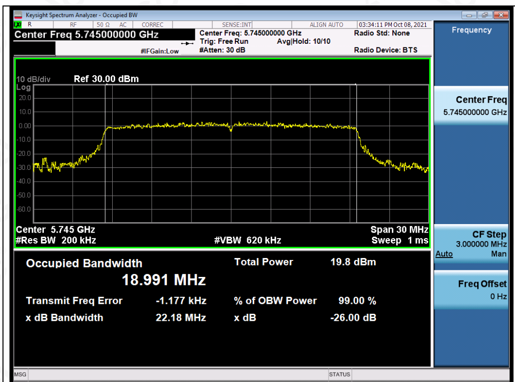
Test_Graph_802.11ax20_ANT1_5745_MCS0_OBW
