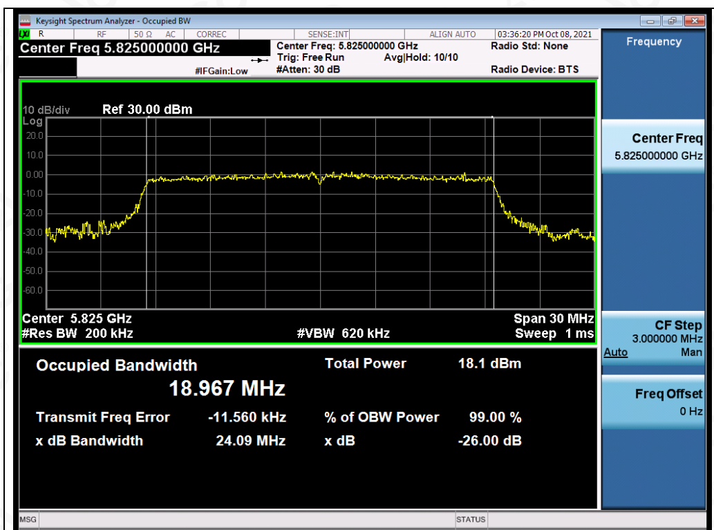
Test_Graph_802.11ax20_ANT1_5825_MCS0_OBW
