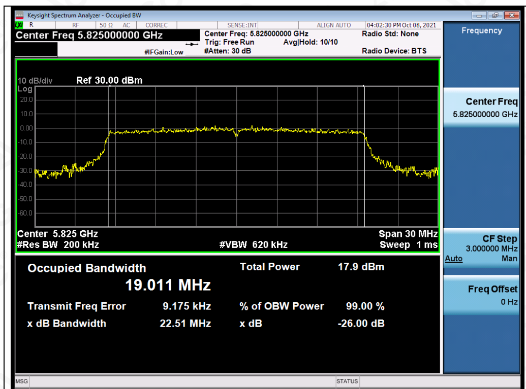
Test_Graph_802.11ax20_ANT2_5825_MCS0_OBW
