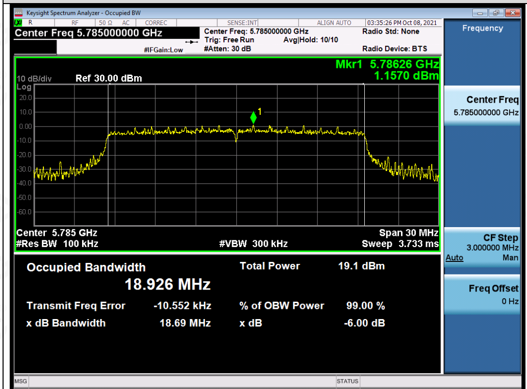
Test_Graph_802.11ax20_ANT1_5785_MCS0_DTSBW
