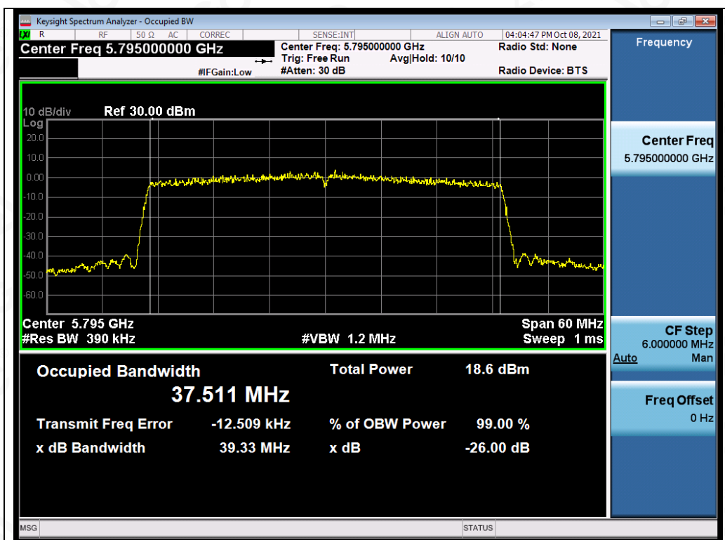
Test_Graph_802.11ax40_ANT2_5795_MCS0_OBW
