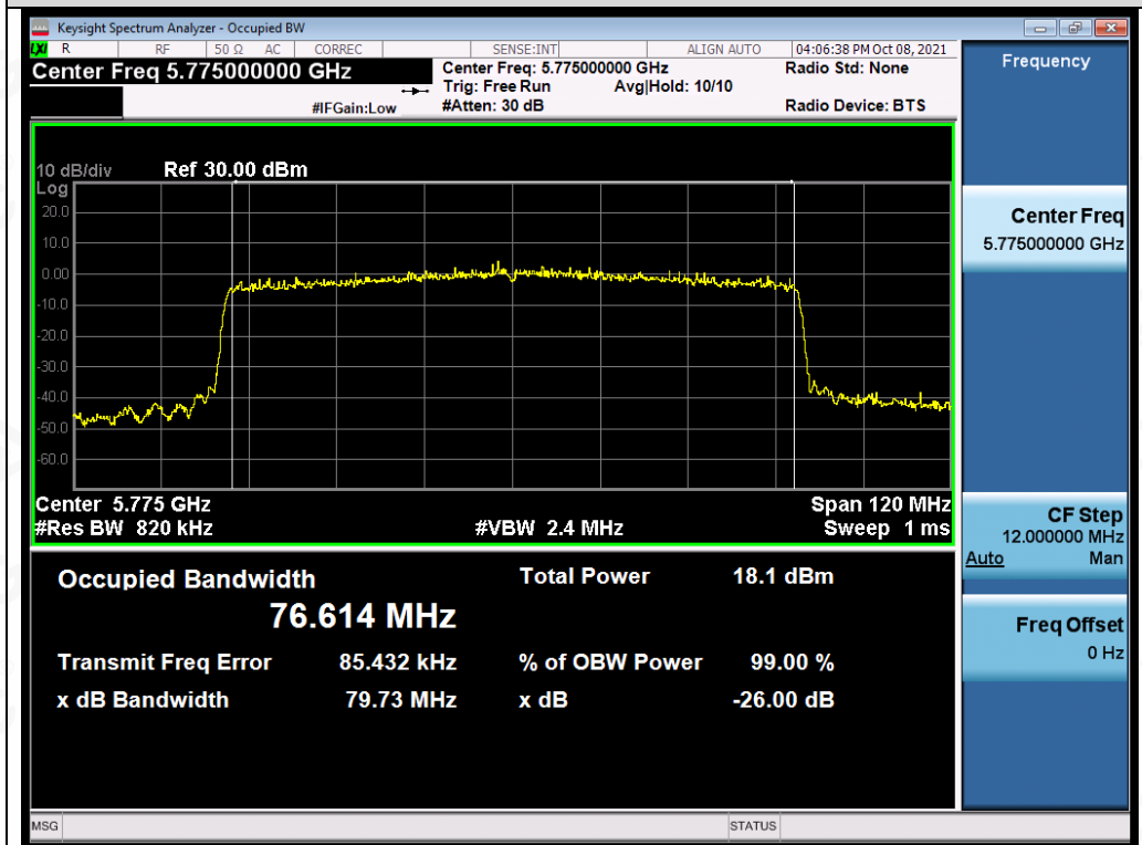
Test_Graph_802.11ax80_ANT2_5775_MCS0_OBW
