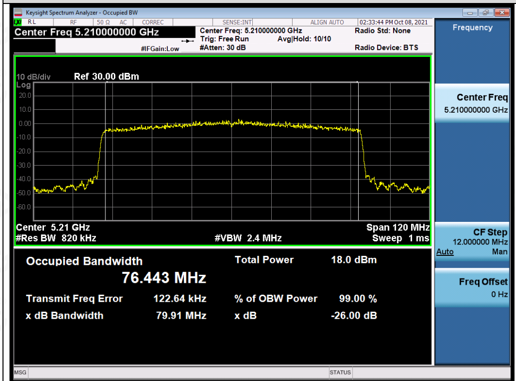
Test_Graph_802.11ax80_ANT2_5210_MCS0_OBW
