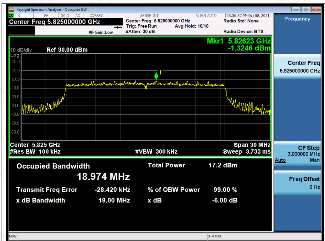
Test_Graph_802.11ax20_ANT1_5825_MCS0_DTSBW
