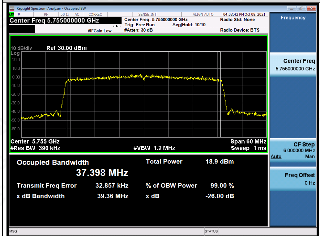
Test_Graph_802.11ax40_ANT2_5755_MCS0_OBW
