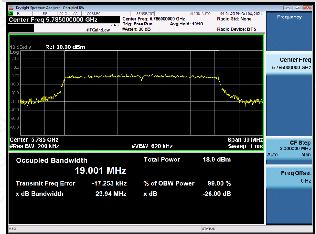
Test_Graph_802.11ax20_ANT2_5785_MCS0_OBW
