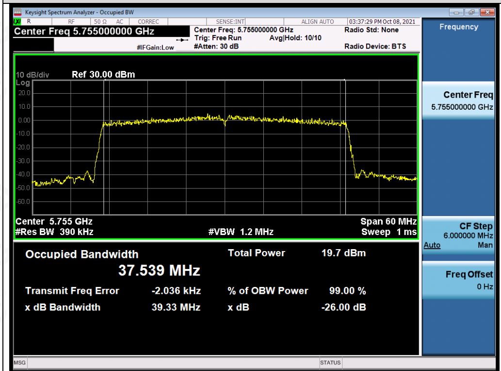
Test_Graph_802.11ax40_ANT1_5755_MCS0_OBW
