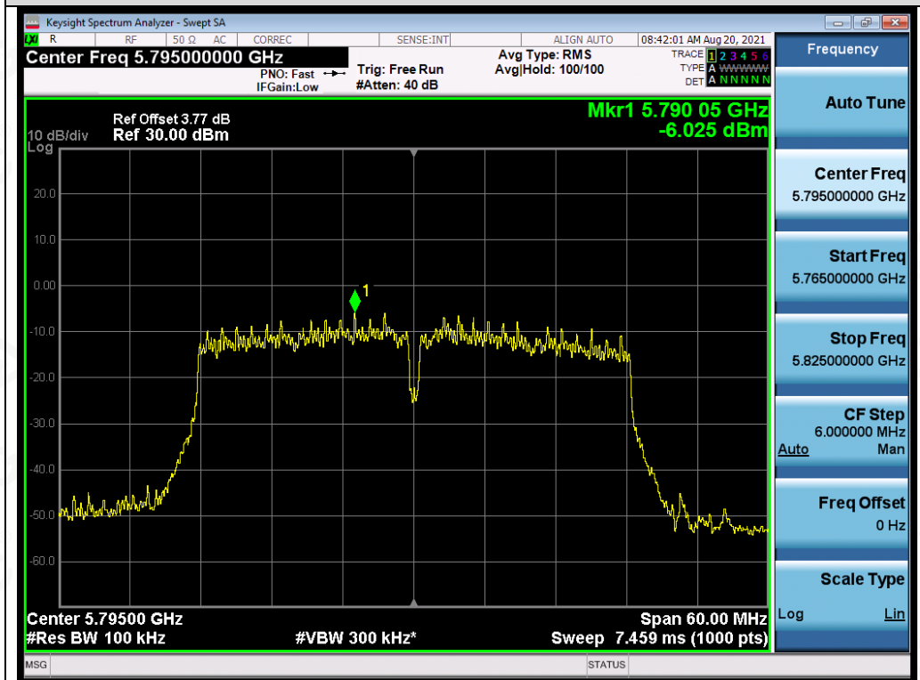
Test_Graph_802.11n40_ANT4_5795_MCS0_PSD
