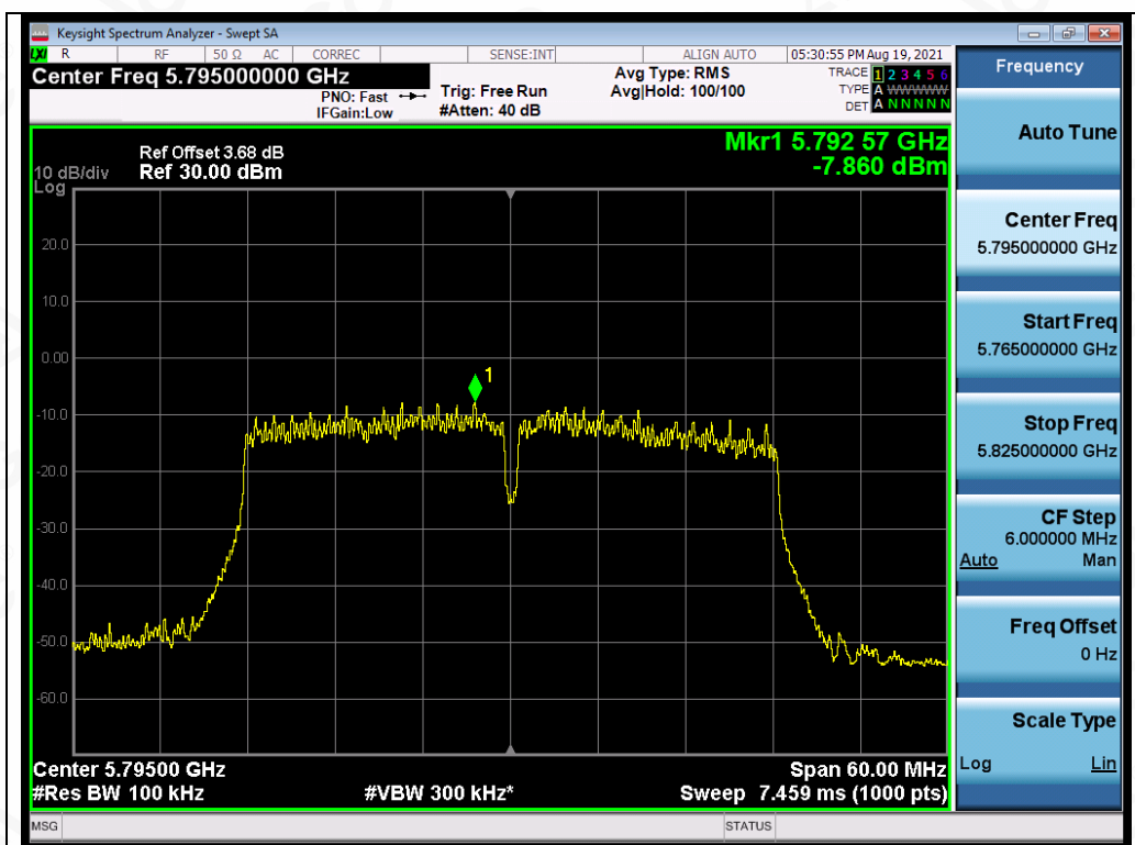
Test_Graph_802.11ac40_ANT3_5795_MCS9_PSD
