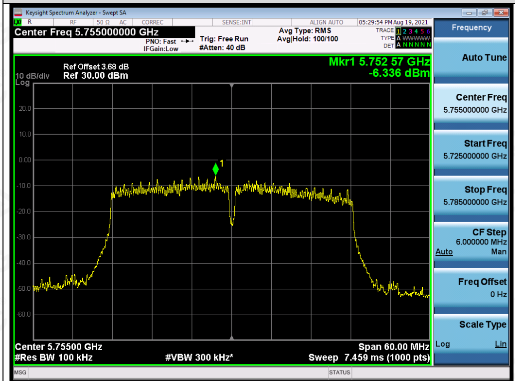
Test_Graph_802.11ac40_ANT3_5755_MCS9_PSD
