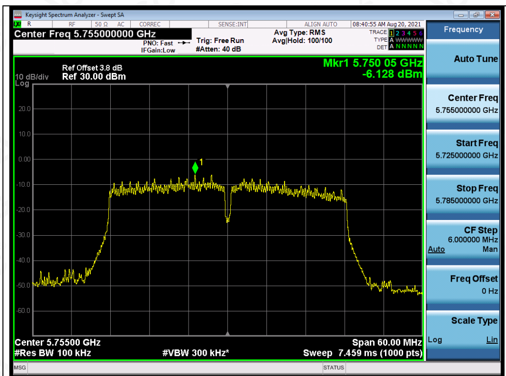
Test_Graph_802.11n40_ANT4_5755_MCS0_PSD
