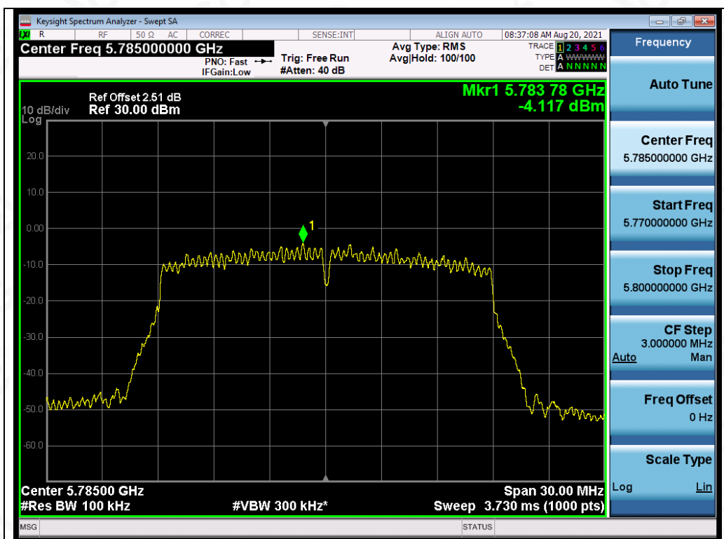
Test_Graph_802.11n20_ANT4_5785_MCS0_PSD
