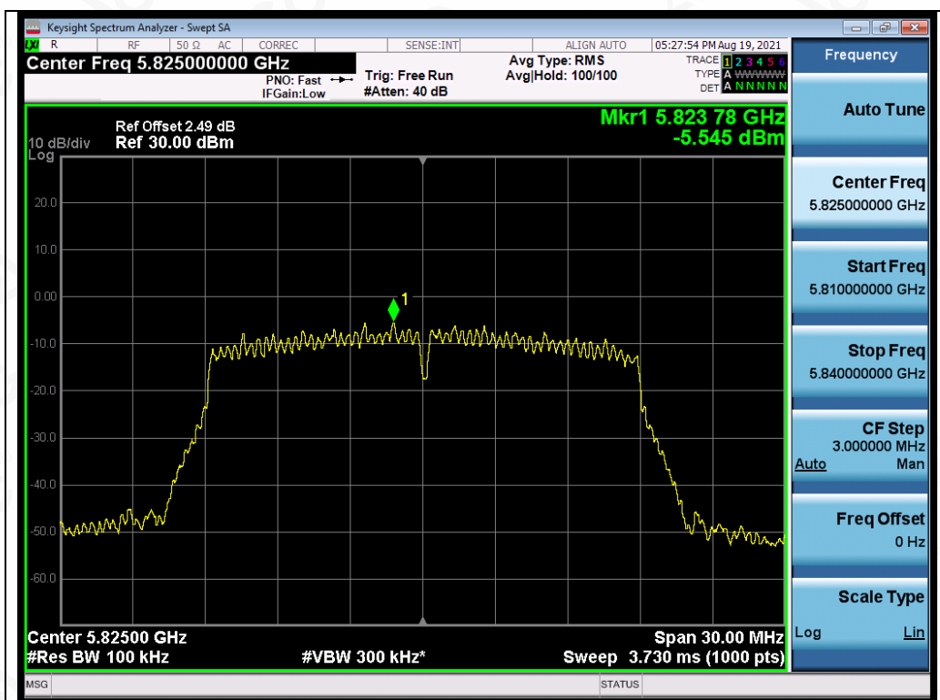
Test_Graph_802.11ac20_ANT3_5825_MCS9_PSD
