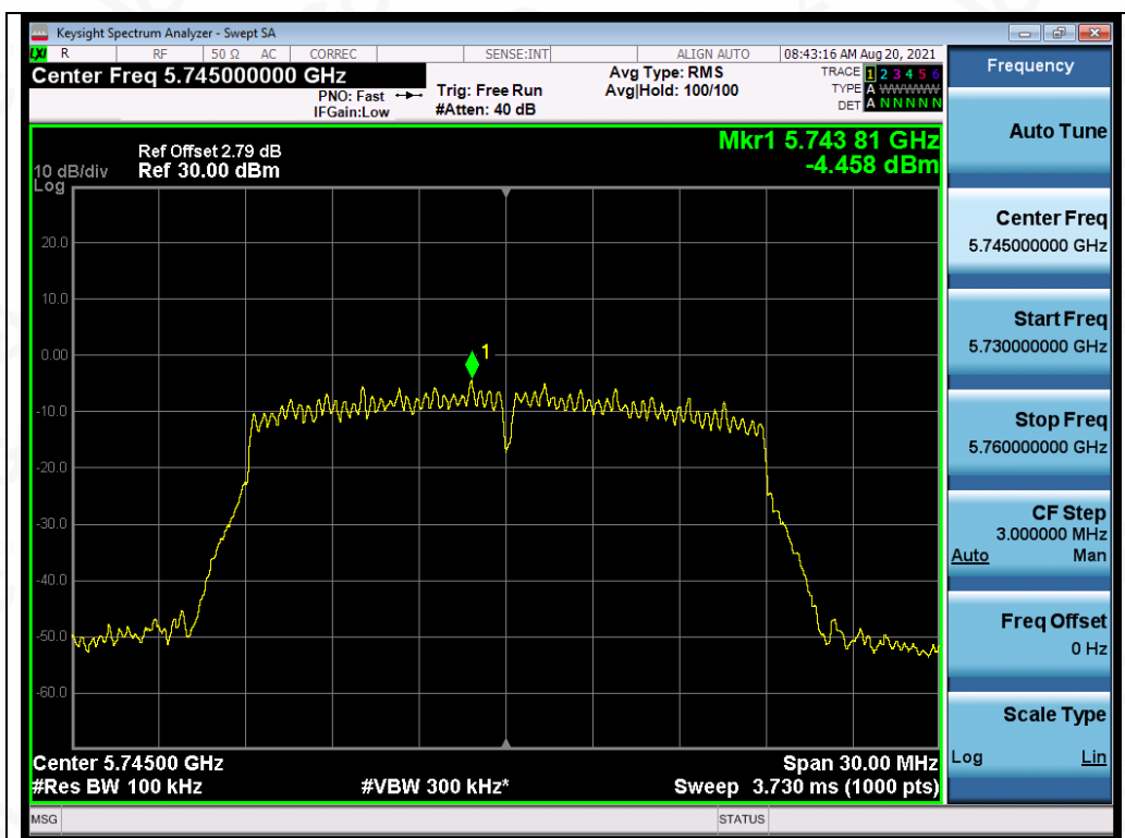
Test_Graph_802.11ac20_ANT4_5745_MCS0_PSD
