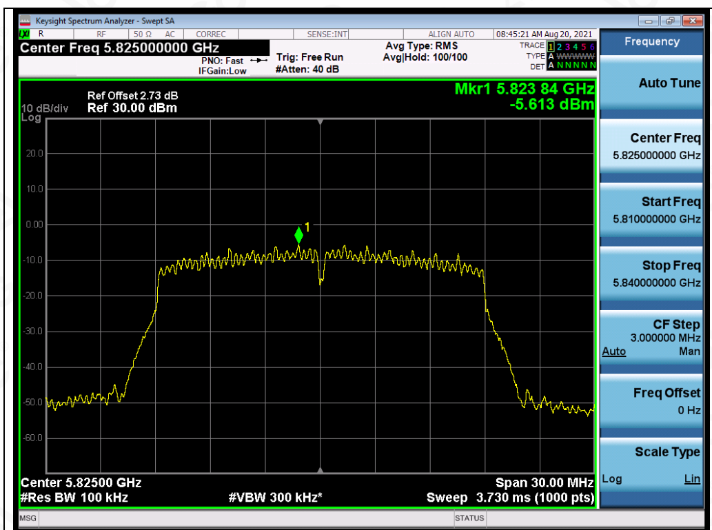
Test_Graph_802.11ac20_ANT4_5825_MCS9_PSD
