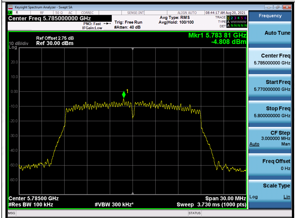
Test_Graph_802.11ac20_ANT4_5785_MCS0_PSD
