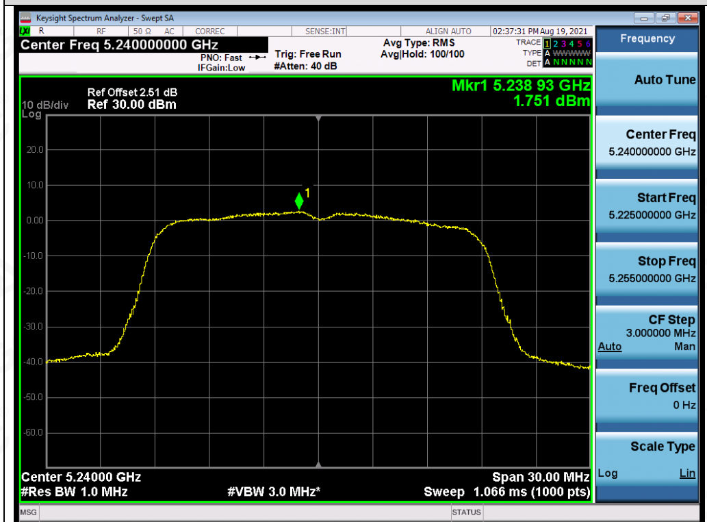
Test_Graph_802.11n20_ANT3_5240_MCS0_PSD
