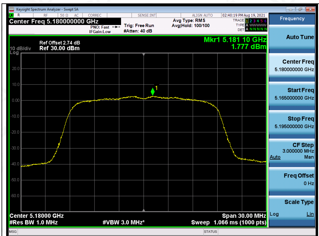
Test_Graph_802.11ac20_ANT3_5180_MCS0_PSD
