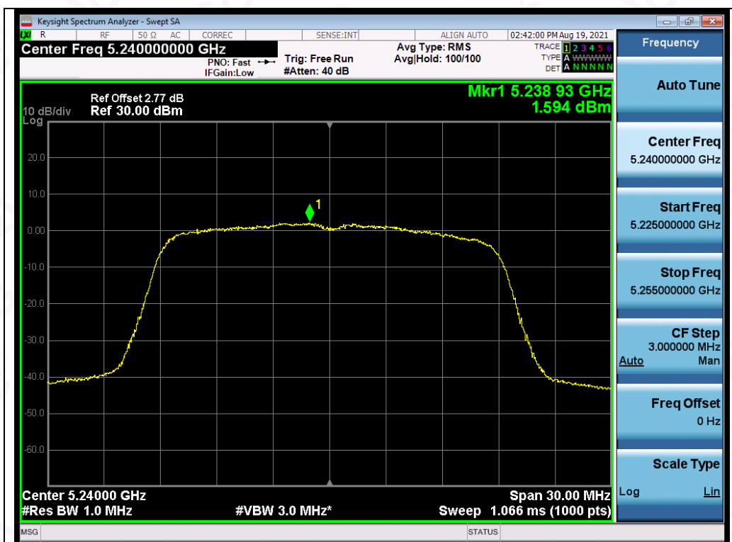
Test_Graph_802.11ac20_ANT3_5240_MCS9_PSD
