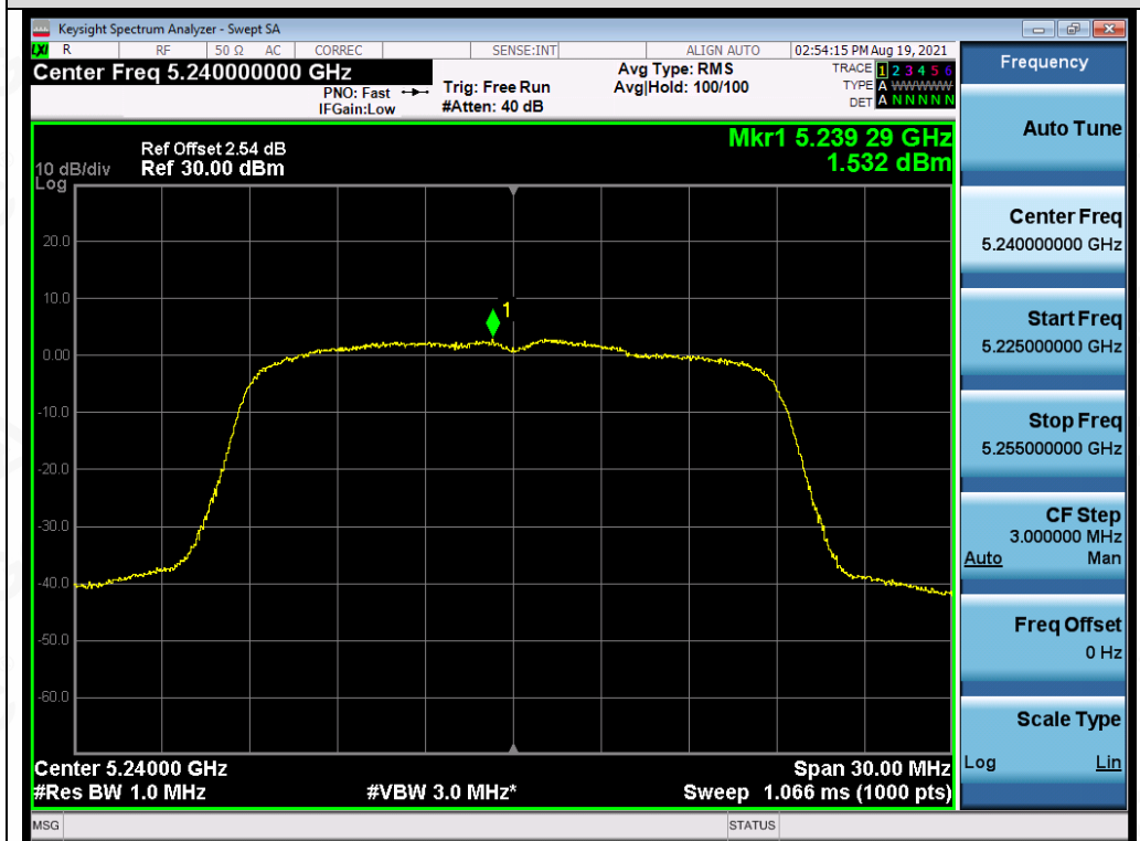
Test_Graph_802.11n20_ANT4_5240_MCS0_PSD
