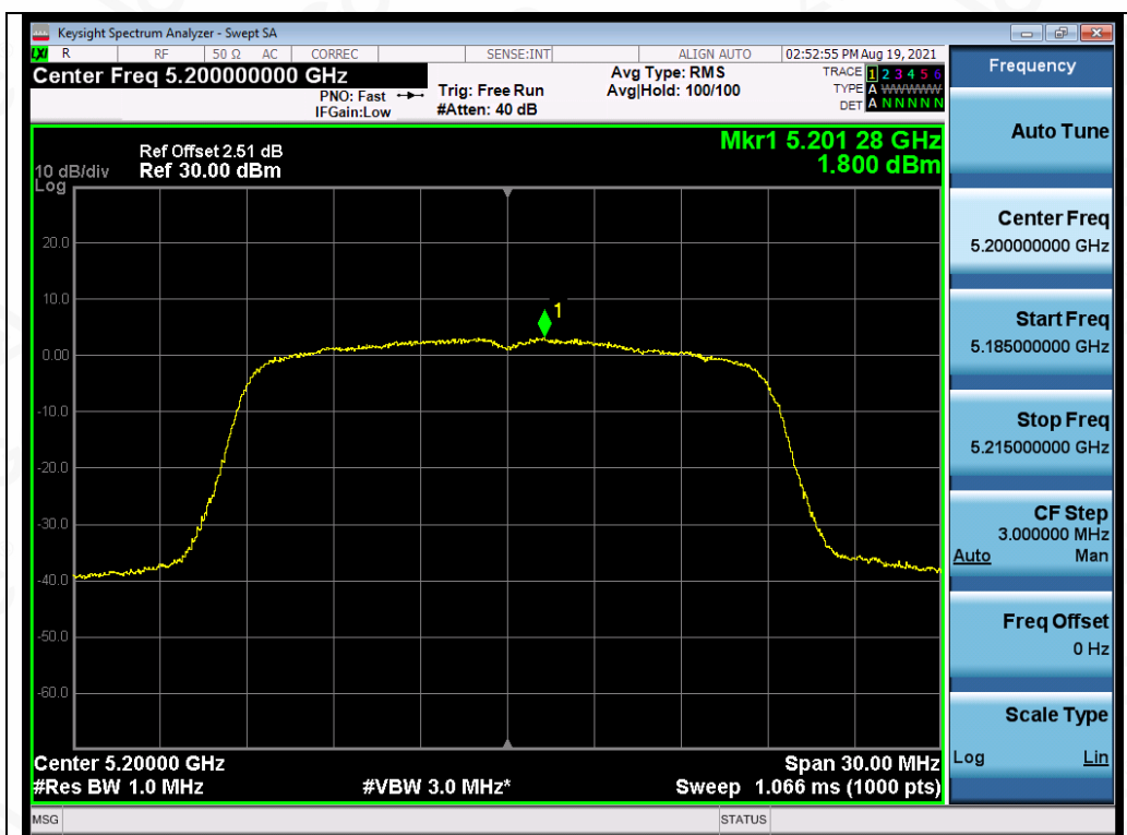
Test_Graph_802.11n20_ANT4_5200_MCS0_PSD
