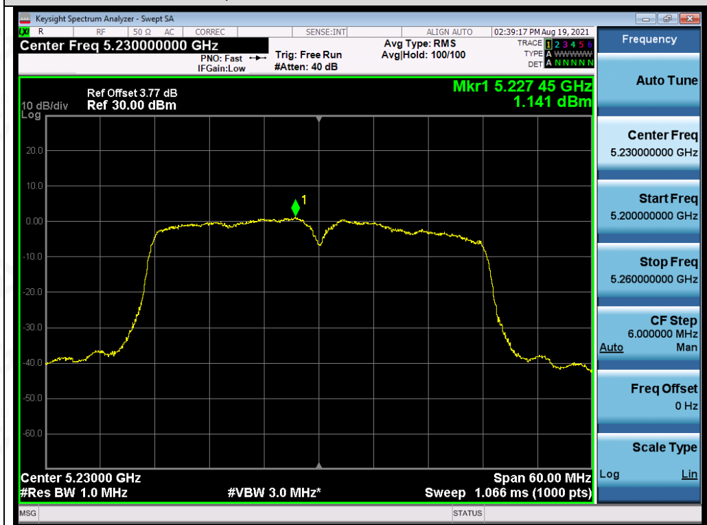
Test_Graph_802.11n40_ANT3_5230_MCS0_PSD
