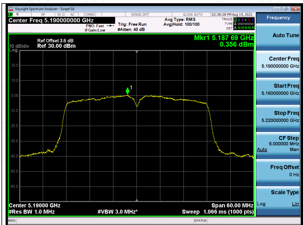
Test_Graph_802.11n40_ANT3_5190_MCS0_PSD
