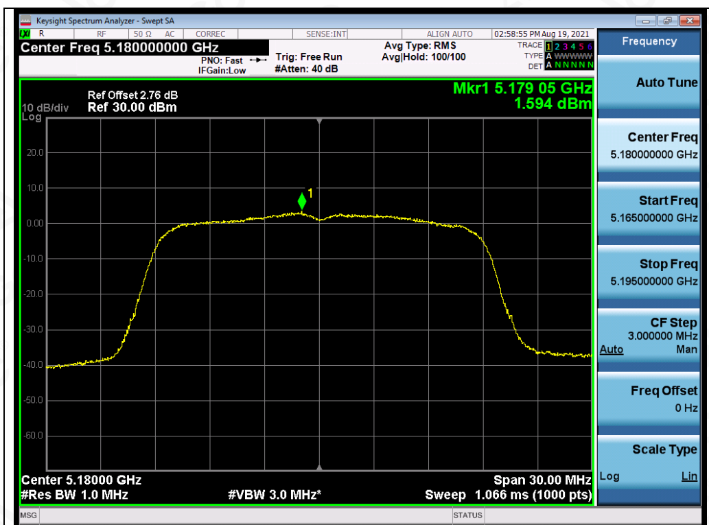
Test_Graph_802.11ac20_ANT4_5180_MCS0_PSD
