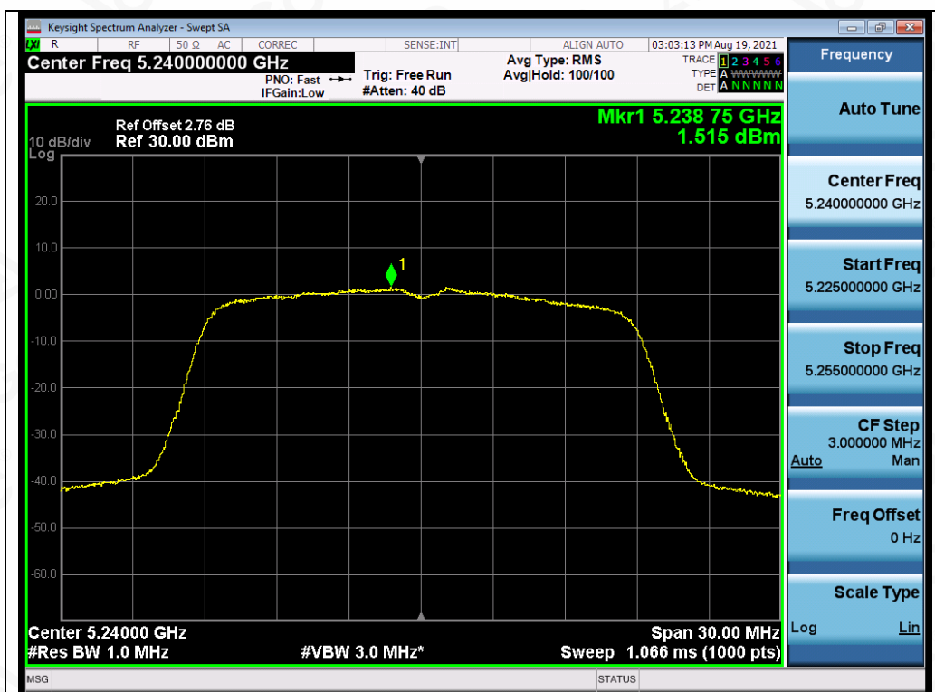
Test_Graph_802.11ac20_ANT4_5240_MCS9_PSD
