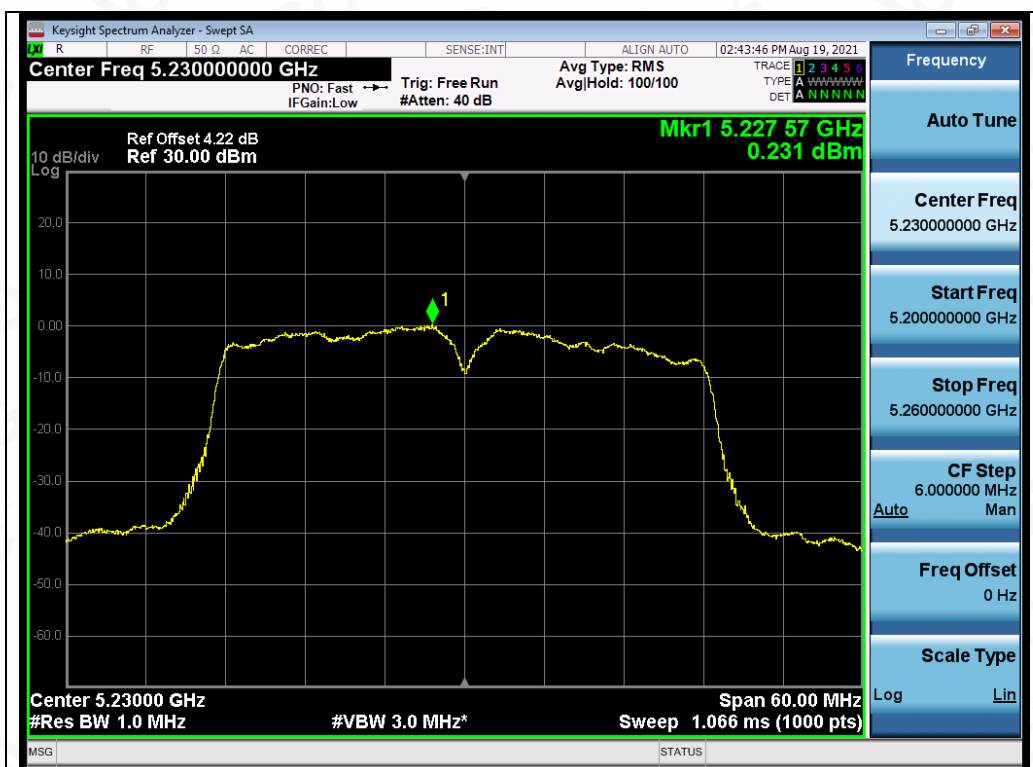
Test_Graph_802.11ac40_ANT3_5230_MCS9_PSD
