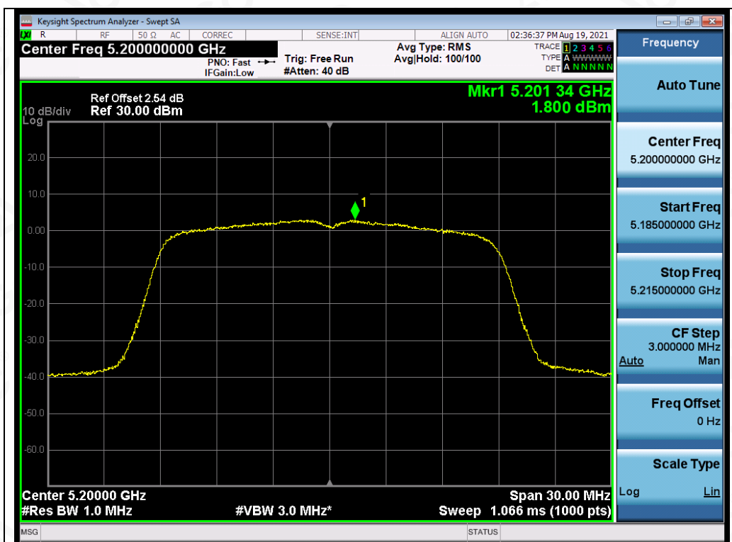
Test_Graph_802.11n20_ANT3_5200_MCS0_PSD
