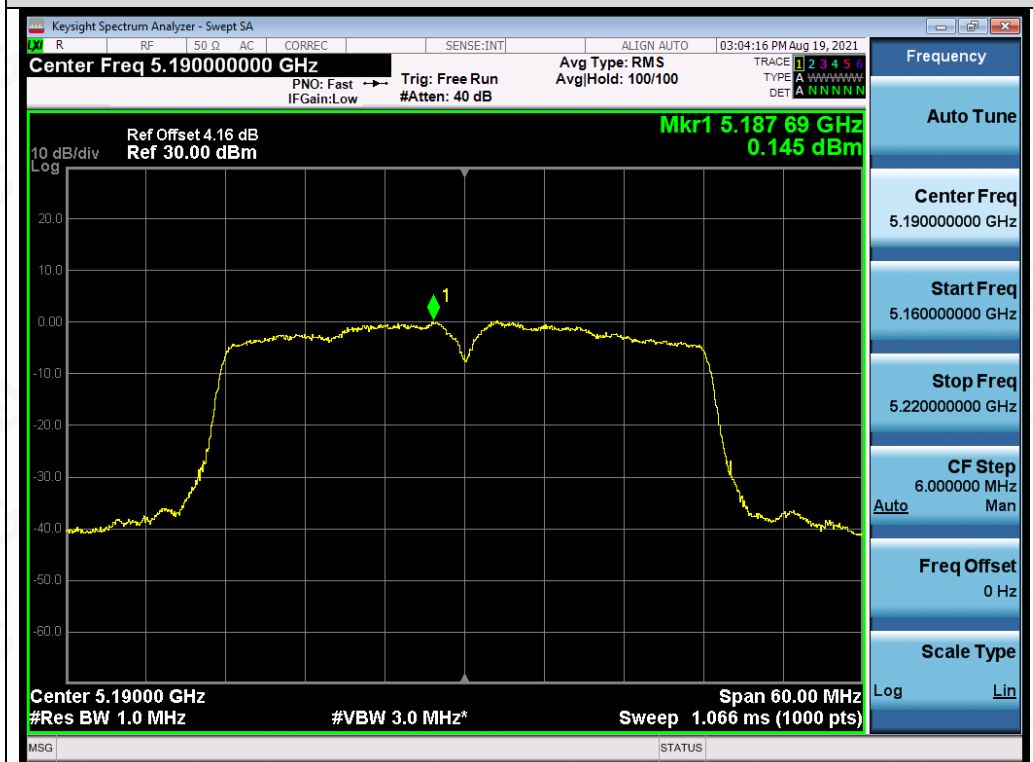
Test_Graph_802.11ac40_ANT4_5190_MCS9_PSD
