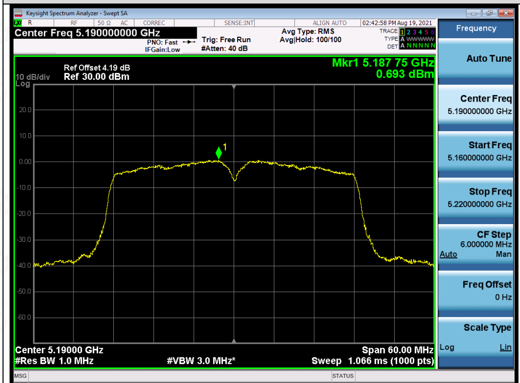
Test_Graph_802.11ac40_ANT3_5190_MCS9_PSD
