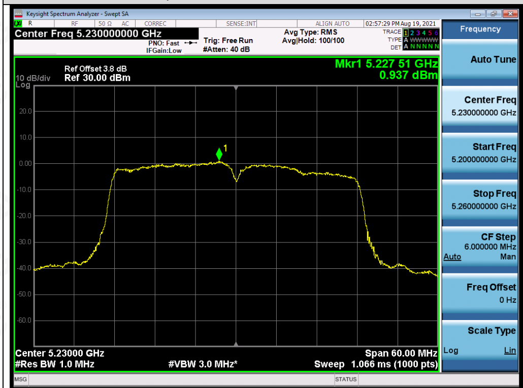
Test_Graph_802.11n40_ANT4_5230_MCS0_PSD
