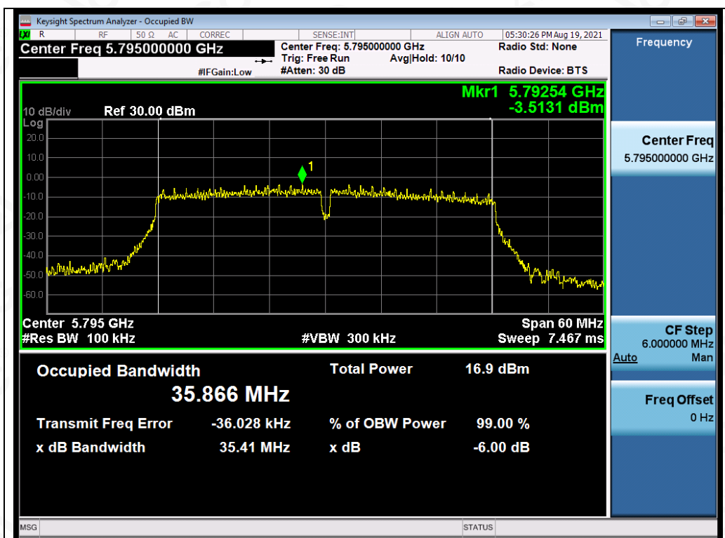
Test_Graph_802.11ac40_ANT3_5795_MCS9_DTSBW
