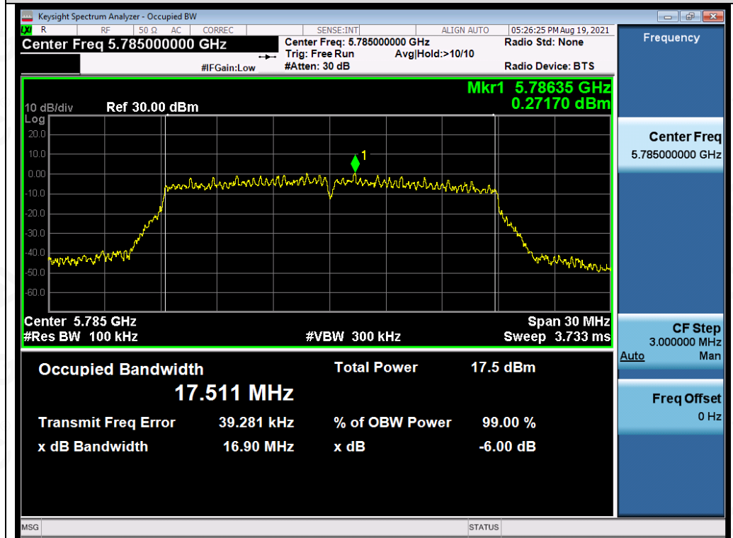
Test_Graph_802.11ac20_ANT3_5785_MCS0_DTSBW
