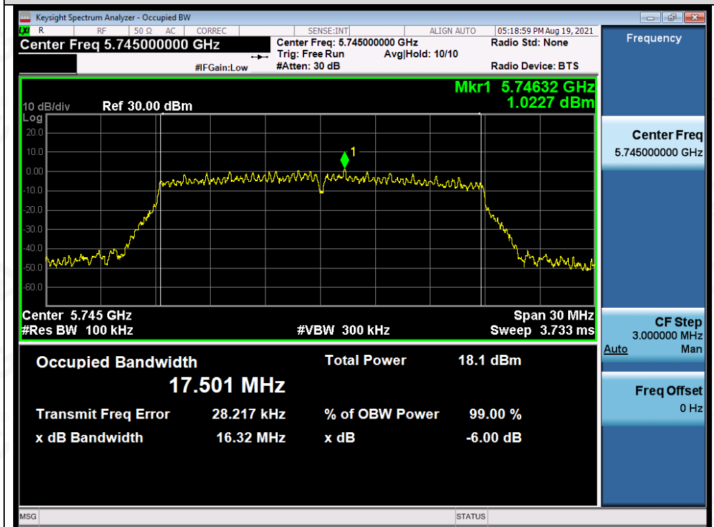
Test_Graph_802.11n20_ANT3_5745_MCS0_DTSBW
