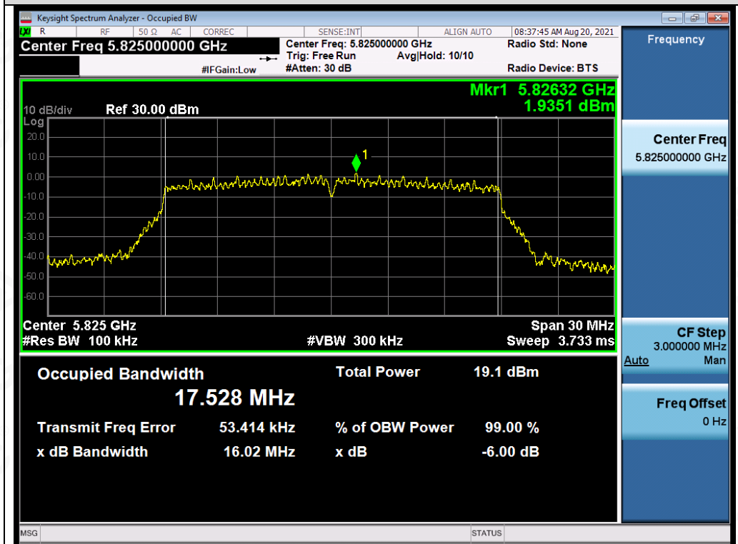
Test_Graph_802.11n20_ANT4_5825_MCS0_DTSBW
