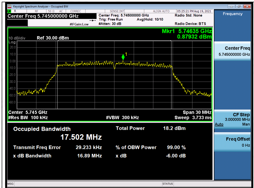
Test_Graph_802.11ac20_ANT3_5745_MCS0_DTSBW
