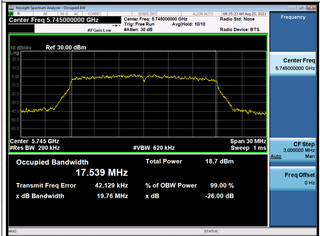
Test_Graph_802.11n20_ANT4_5745_MCS0_OBW
