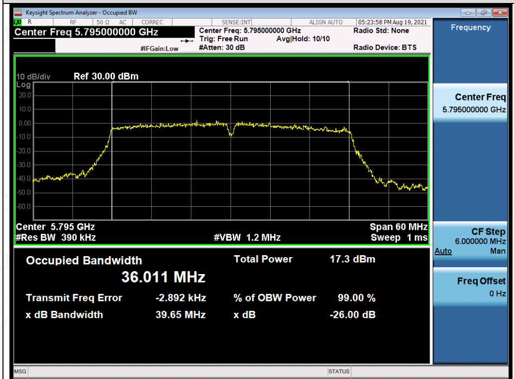
Test_Graph_802.11n40_ANT3_5795_MCS0_OBW
