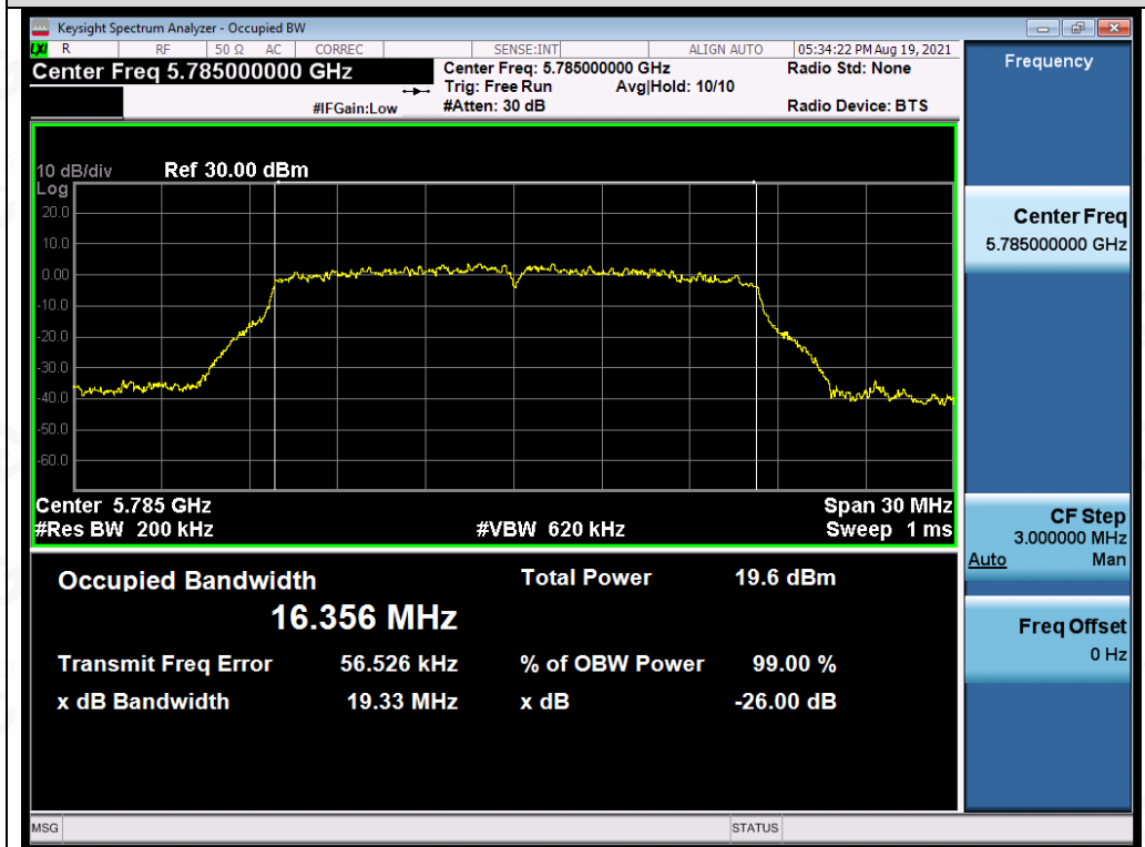
Test_Graph_802.11a_ANT4_5785_6Mbps_OBW
