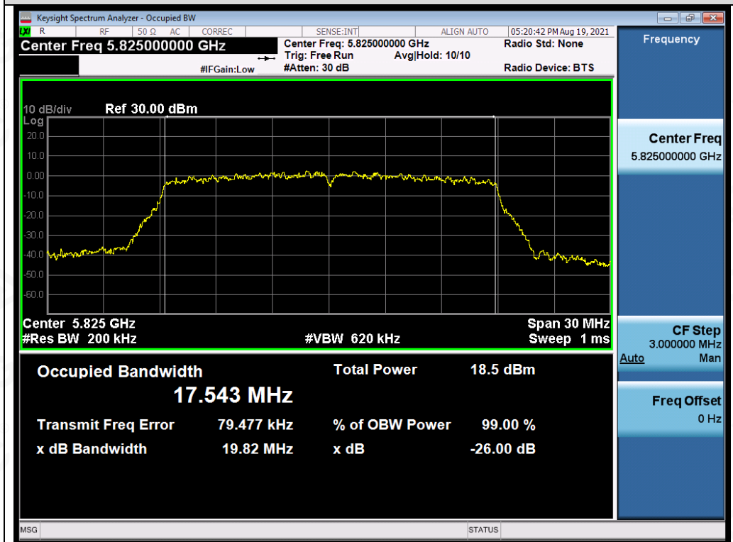
Test_Graph_802.11n20_ANT3_5825_MCS0_OBW
