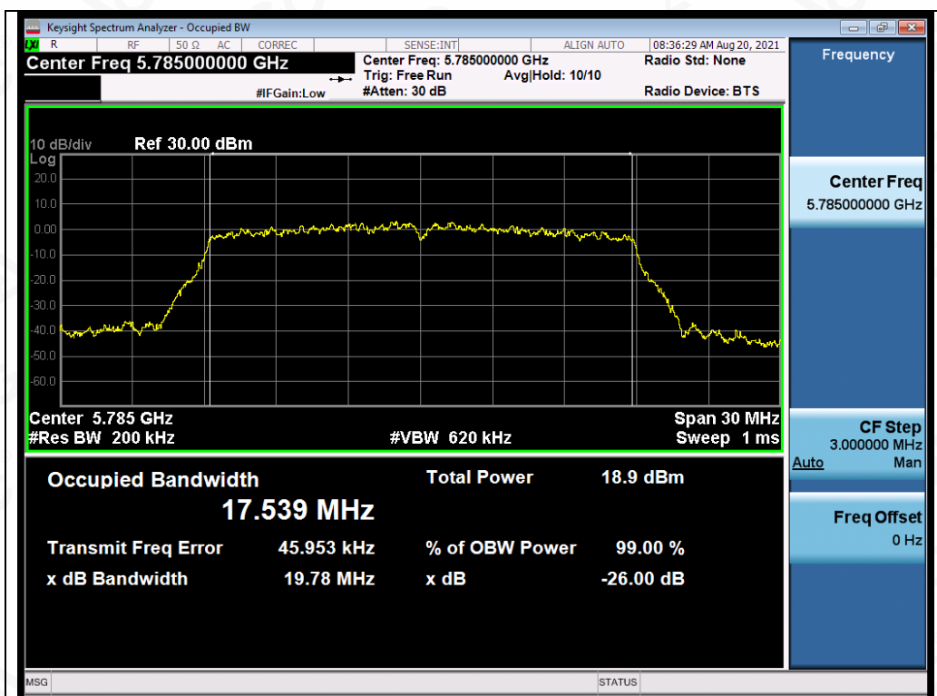
Test_Graph_802.11n20_ANT4_5785_MCS0_OBW
