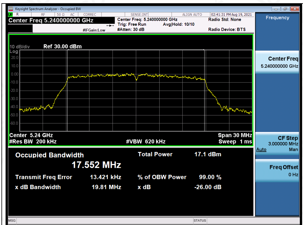
Test_Graph_802.11ac20_ANT3_5240_MCS9_OBW
