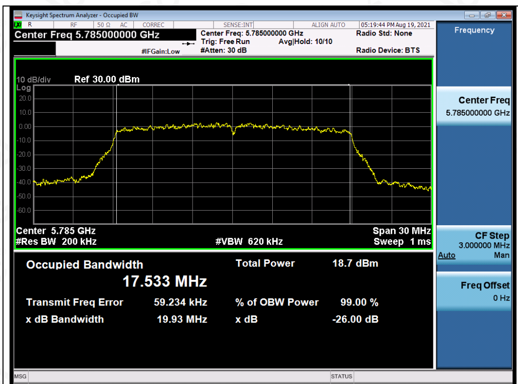
Test_Graph_802.11n20_ANT3_5785_MCS0_OBW
