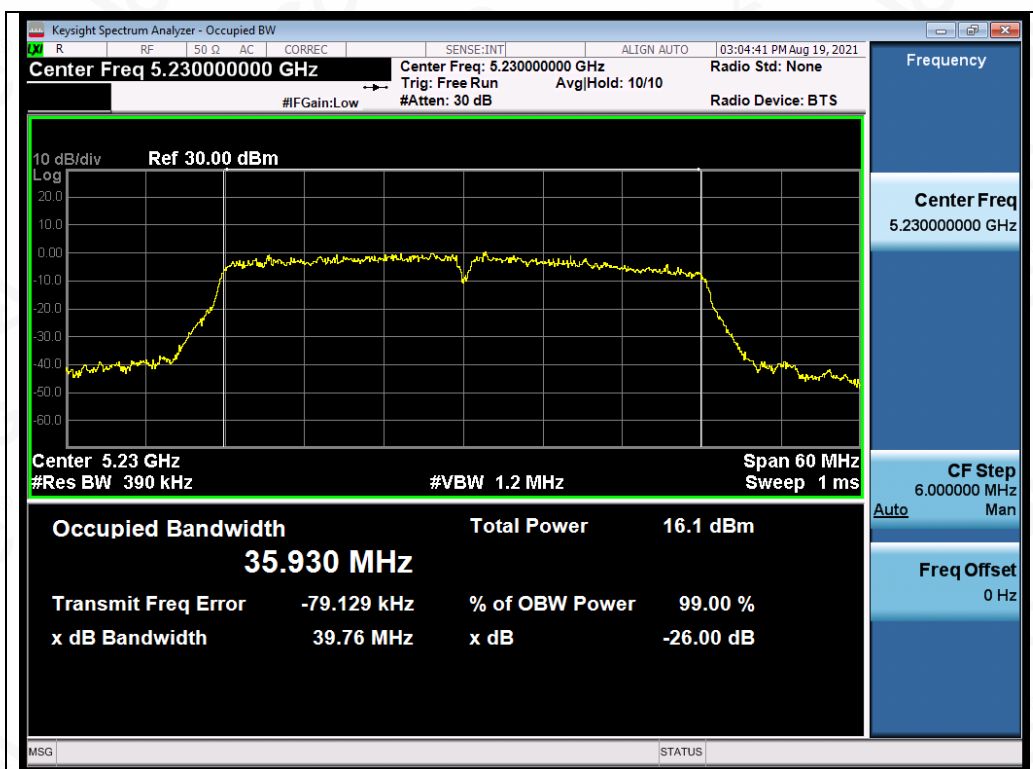
Test_Graph_802.11ac40_ANT4_5230_MCS9_OBW
