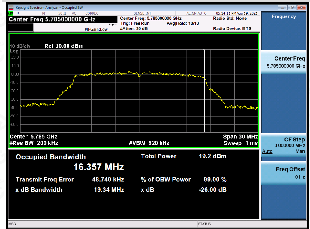
Test_Graph_802.11a_ANT3_5785_6Mbps_OBW
