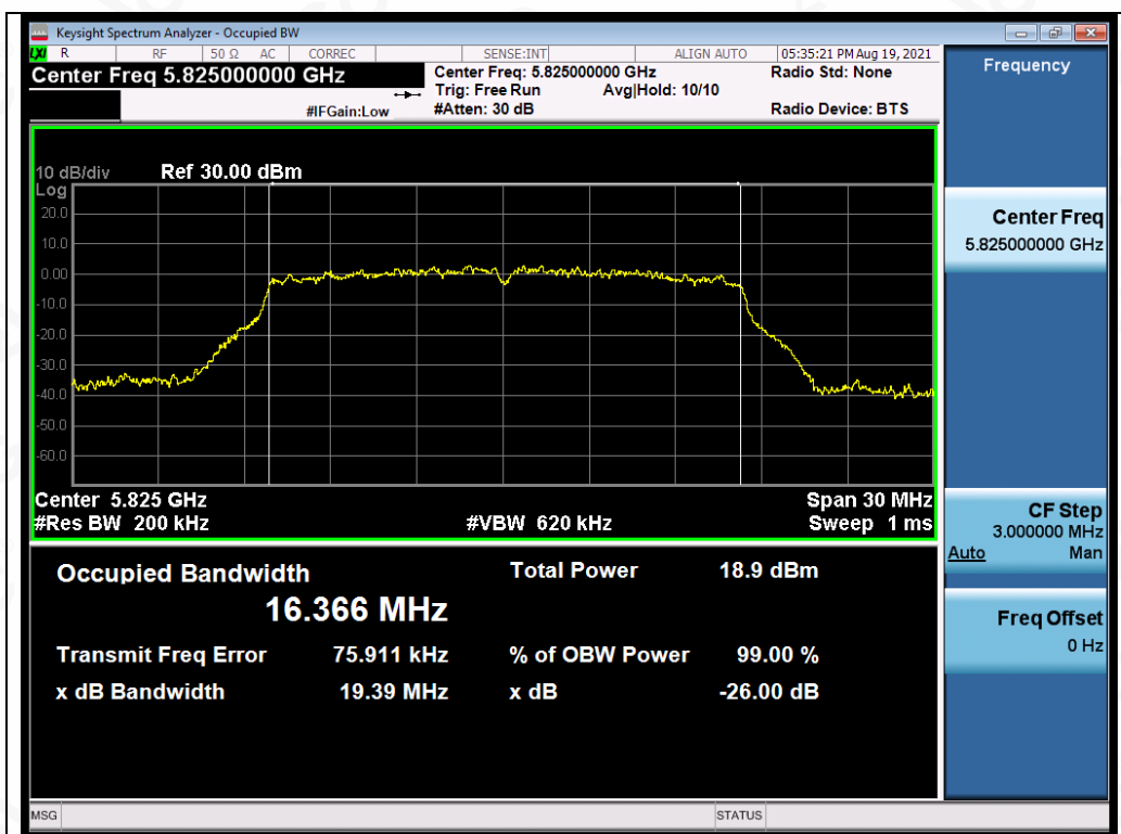
Test_Graph_802.11a_ANT4_5825_6Mbps_OBW
