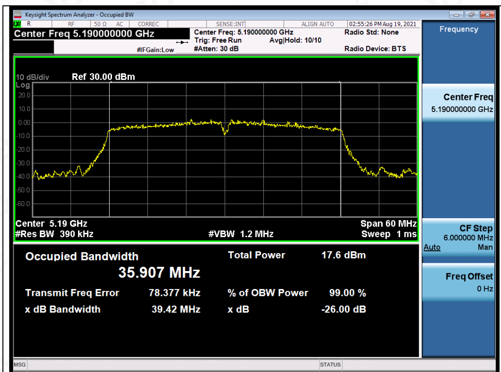
Test_Graph_802.11n40_ANT4_5190_MCS0_OBW
