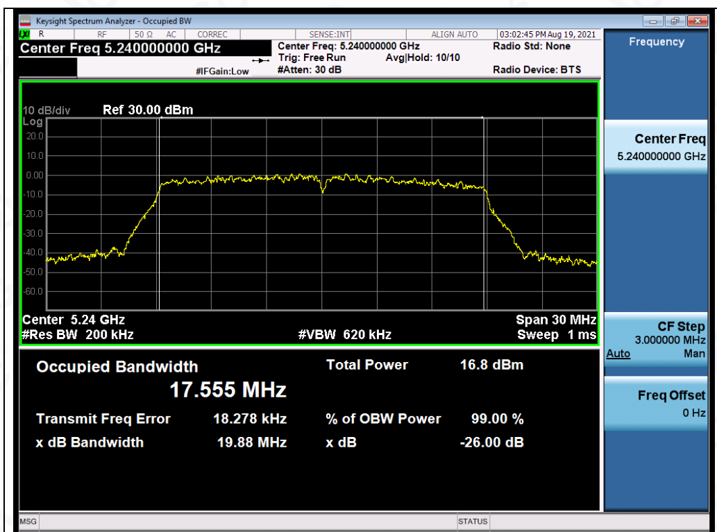
Test_Graph_802.11ac20_ANT4_5240_MCS9_OBW
