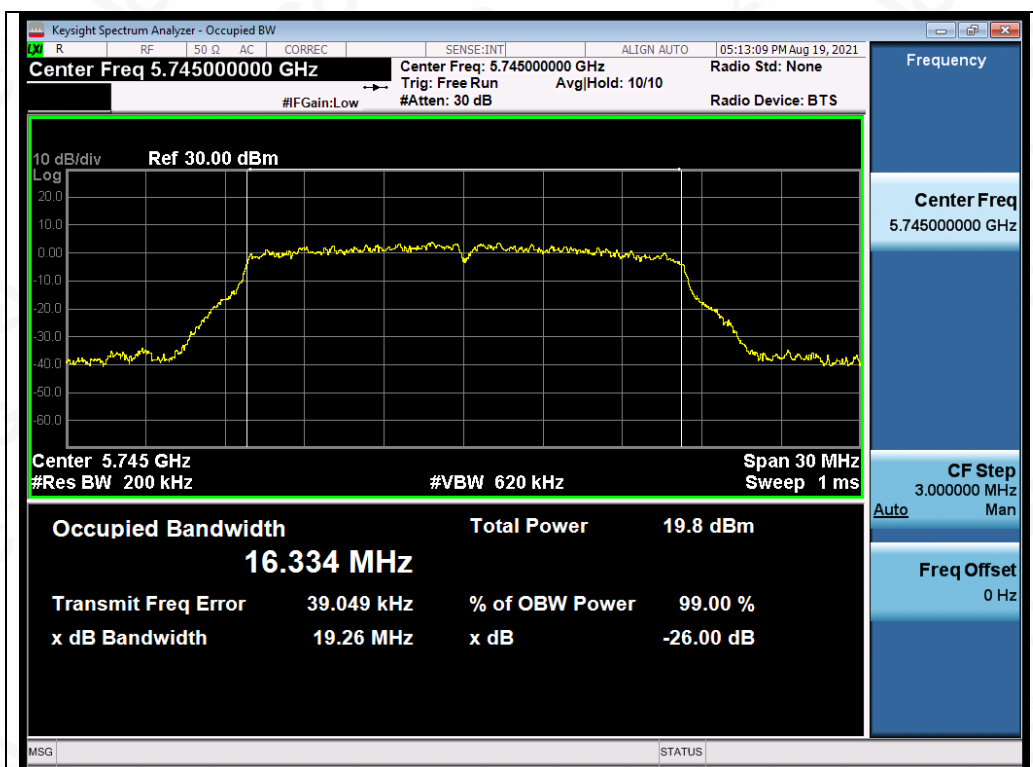
Test_Graph_802.11a_ANT3_5745_6Mbps_OBW
