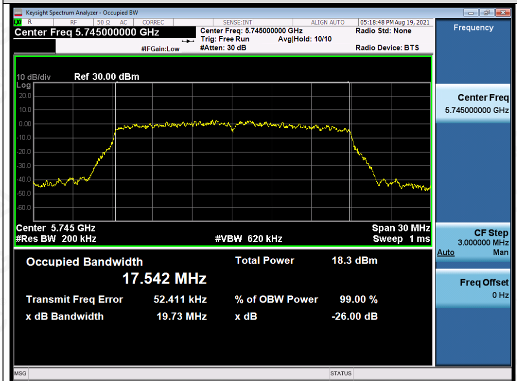
Test_Graph_802.11n20_ANT3_5745_MCS0_OBW
