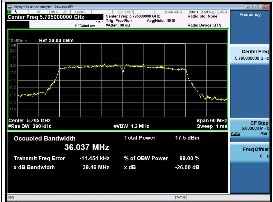
Test_Graph_802.11n40_ANT4_5795_MCS0_OBW
