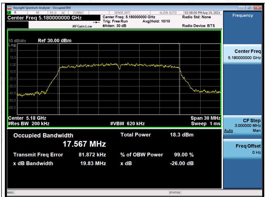
Test_Graph_802.11ac20_ANT4_5180_MCS0_OBW
