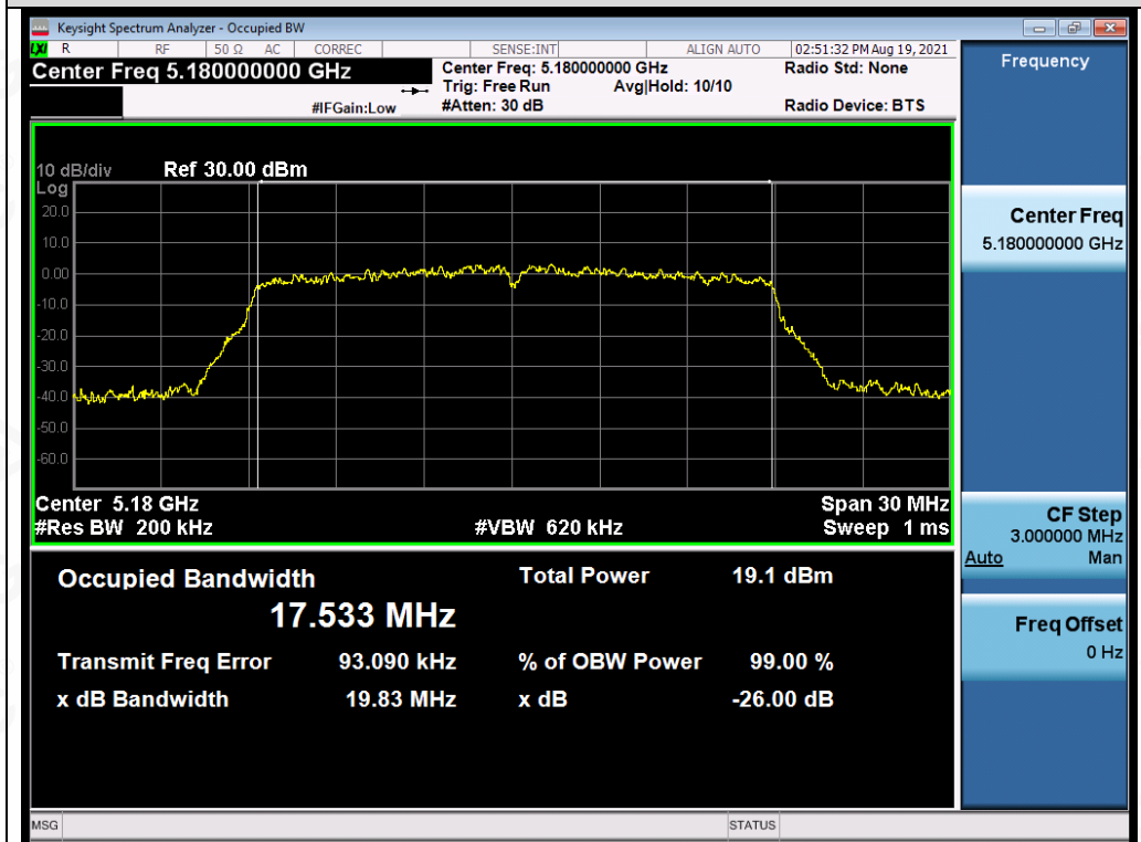
Test_Graph_802.11n20_ANT4_5180_MCS0_OBW
