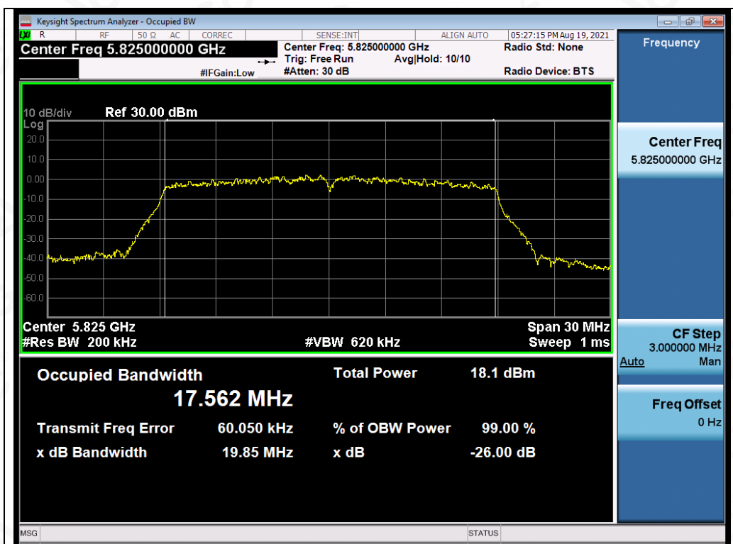
Test_Graph_802.11ac20_ANT3_5825_MCS9_OBW
