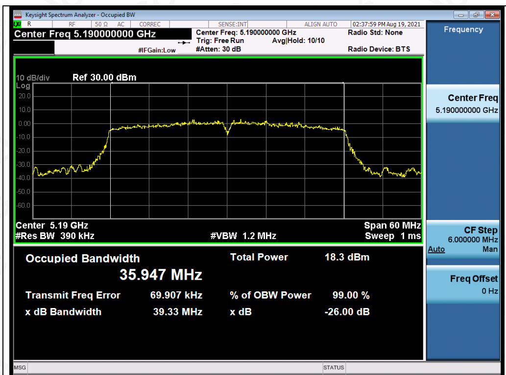
Test_Graph_802.11n40_ANT3_5190_MCS0_OBW
