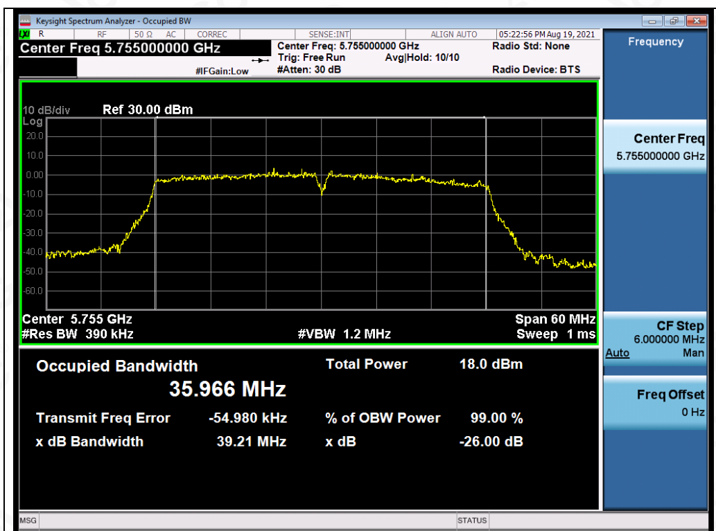
Test_Graph_802.11n40_ANT3_5755_MCS0_OBW
