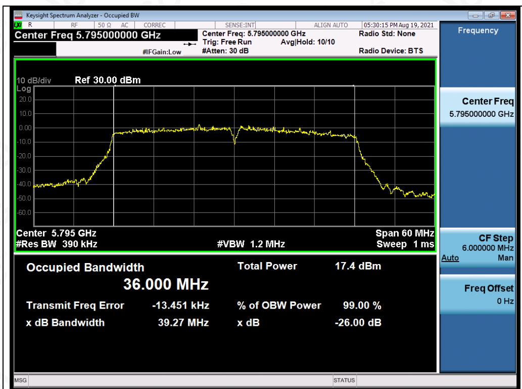
Test_Graph_802.11ac40_ANT3_5795_MCS9_OBW
