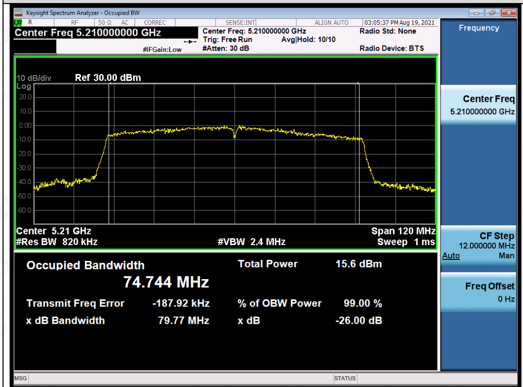
Test_Graph_802.11ac80_ANT4_5210_MCS9_OBW
