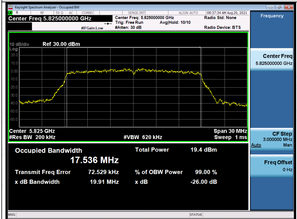
Test_Graph_802.11n20_ANT4_5825_MCS0_OBW
