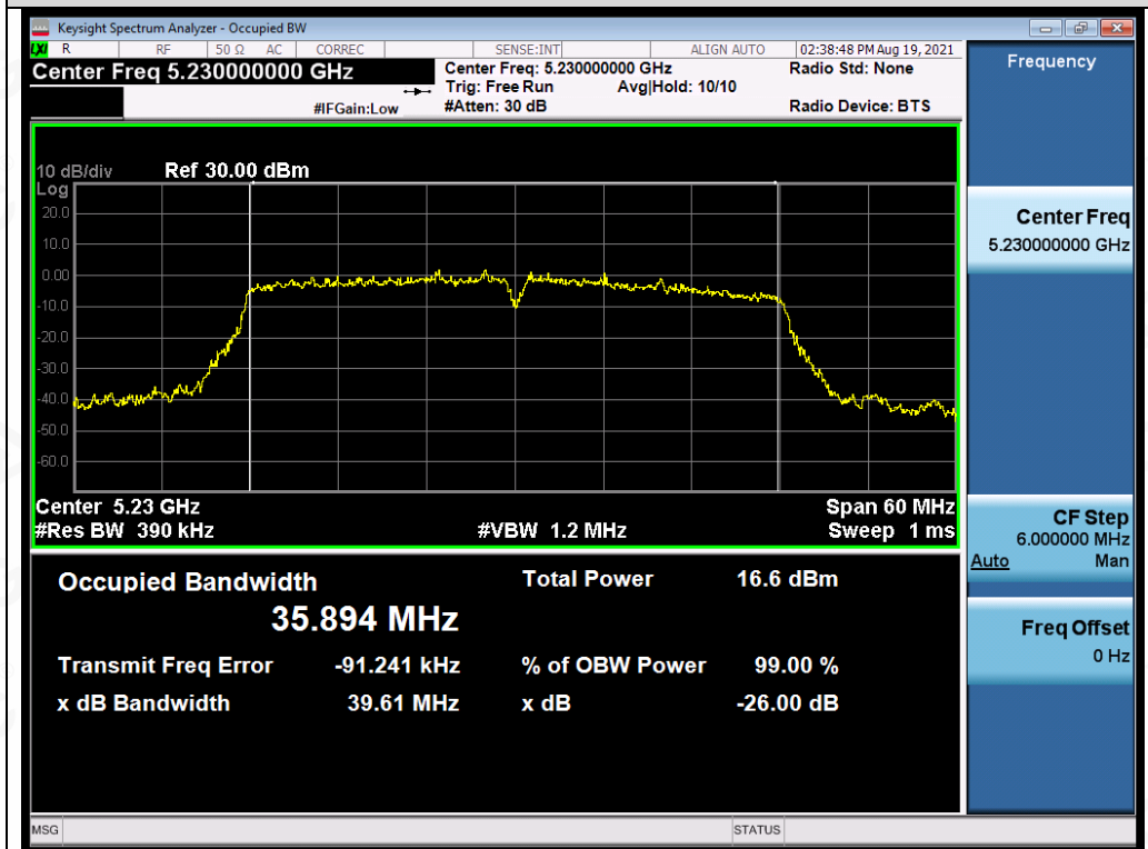
Test_Graph_802.11n40_ANT3_5230_MCS0_OBW
