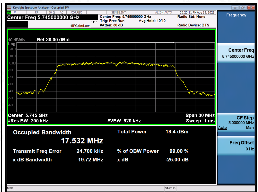
Test_Graph_802.11ac20_ANT3_5745_MCS0_OBW
