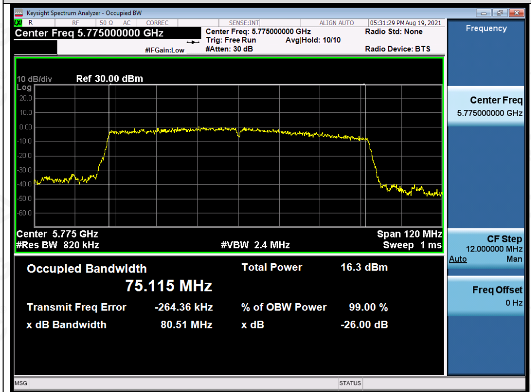
Test_Graph_802.11ac80_ANT3_5775_MCS9_OBW
