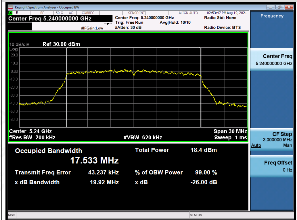
Test_Graph_802.11n20_ANT4_5240_MCS0_OBW
