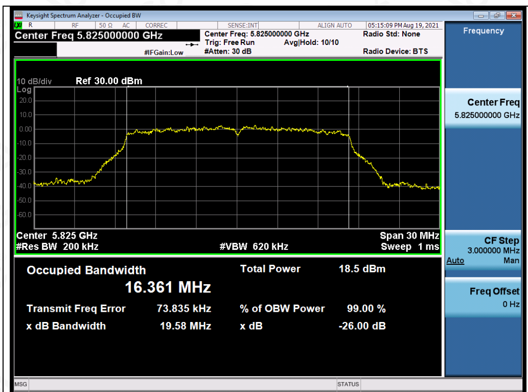
Test_Graph_802.11a_ANT3_5825_6Mbps_OBW
