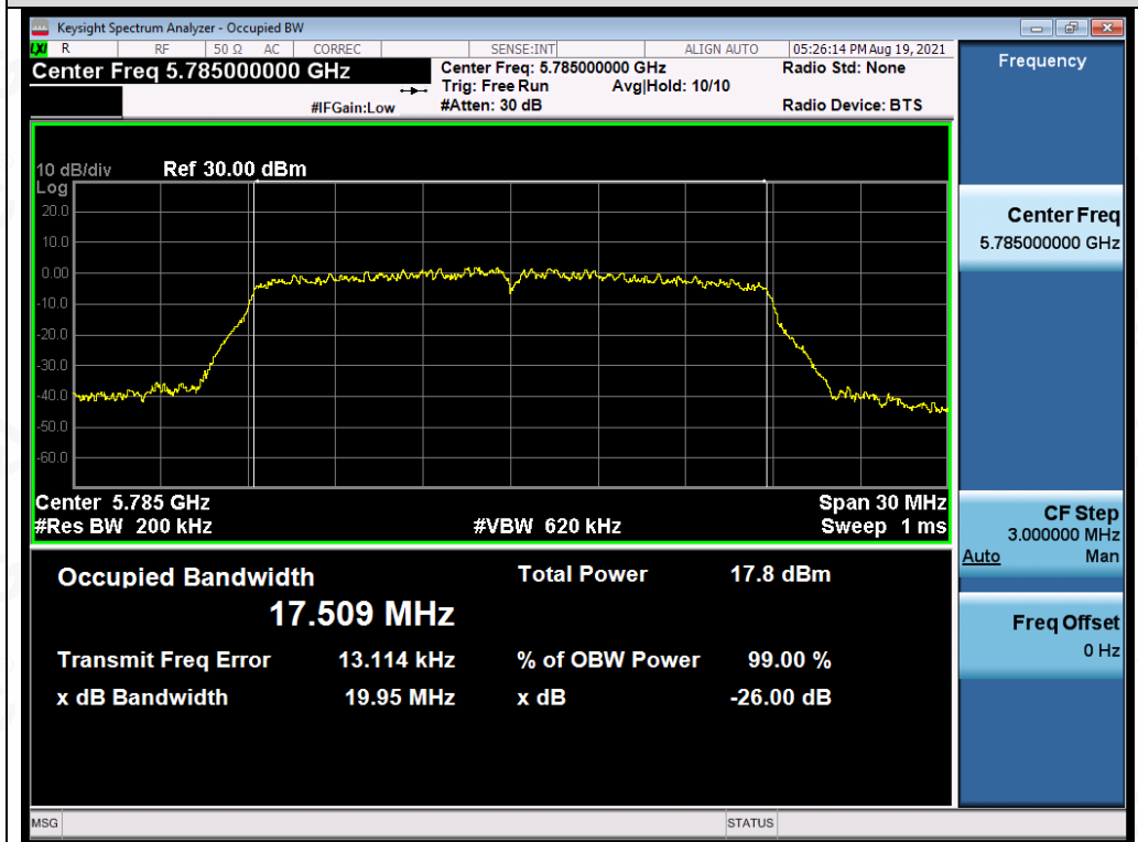
Test_Graph_802.11ac20_ANT3_5785_MCS0_OBW
