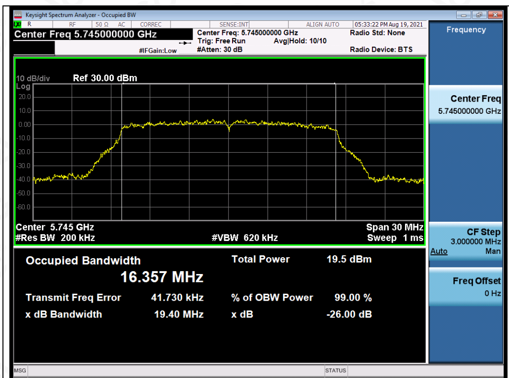
Test_Graph_802.11a_ANT4_5745_6Mbps_OBW
