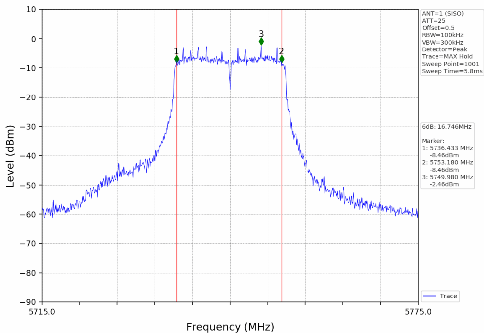
Bandwidth NTNV_802.11ac(VHT20)_SISO_5745MHz_ANT1
