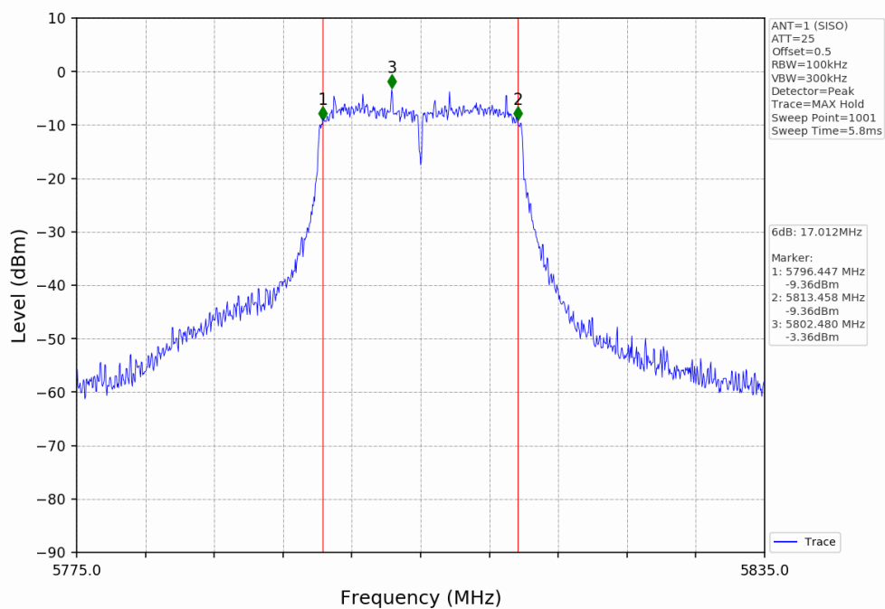
Bandwidth NTNV_802.11n(HT20)_SISO_5805MHz_ANT1
