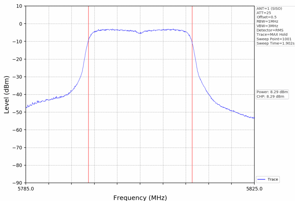
Maximum Conducted Outpower NTNV_802.11n(HT20)_SISO_5805MHz_ANT1
