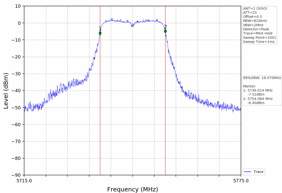
Bandwidth NTN 802.11ac(VHT20) SISO 5745MHz ANT1
