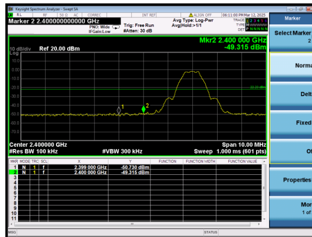
Bluetooth Low Energy 1Mbps
