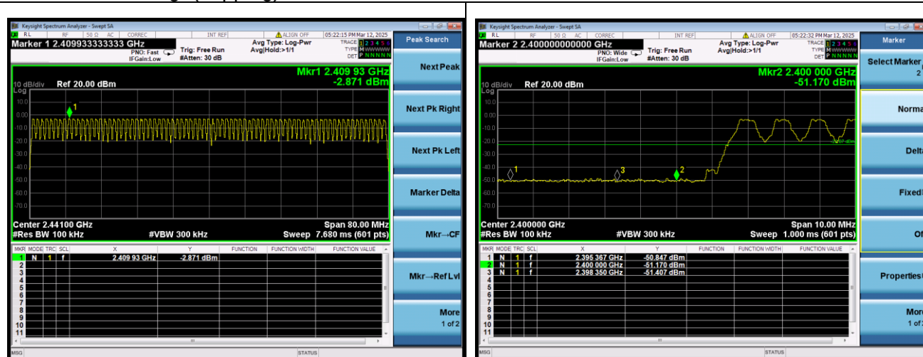
Bluetooth For Classic 1-DH5
