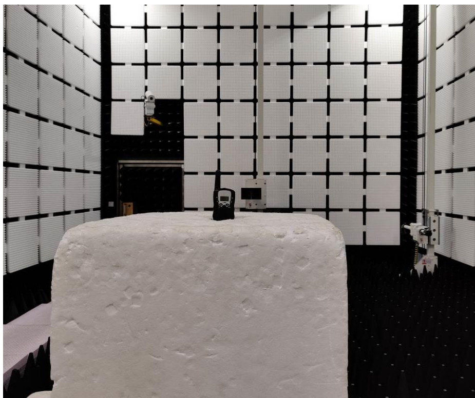
Above 1GHz
