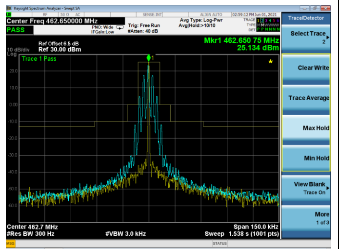
Channel 19: 462.6500MHz
