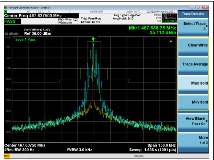
Channel 11: 467.6375MHz
