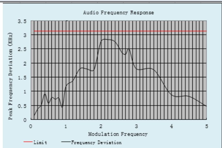
Channel 11: 467.6375MHz
