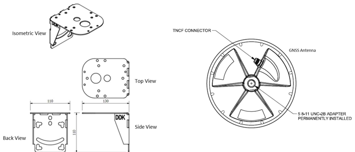
Figure 1: Universal Mounting Bracket and C-Nav289 GNSS Antenna
