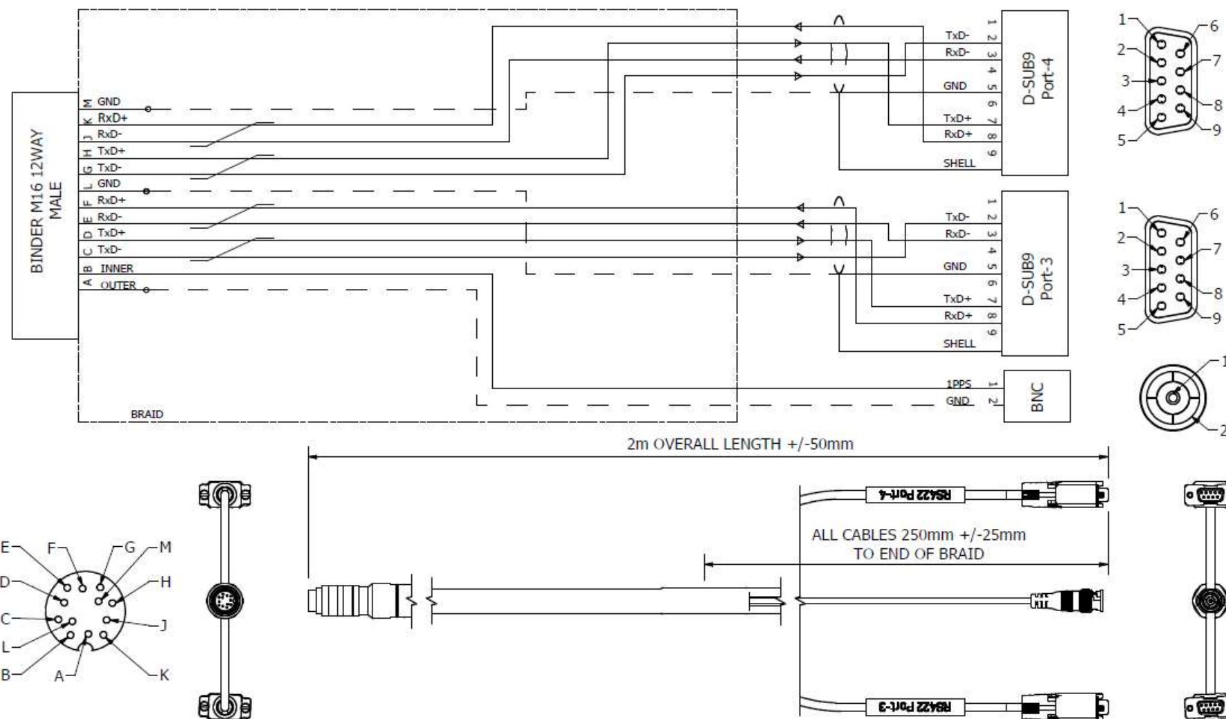
Figure 11: C-NavX1 3-Way AUX Spider Cable Schematic
