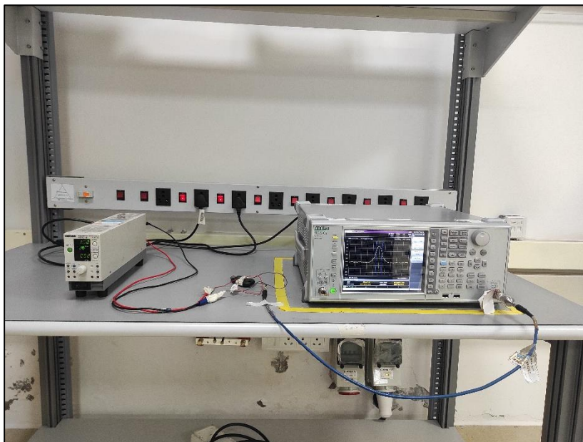
Conducted Test Setup Photo
