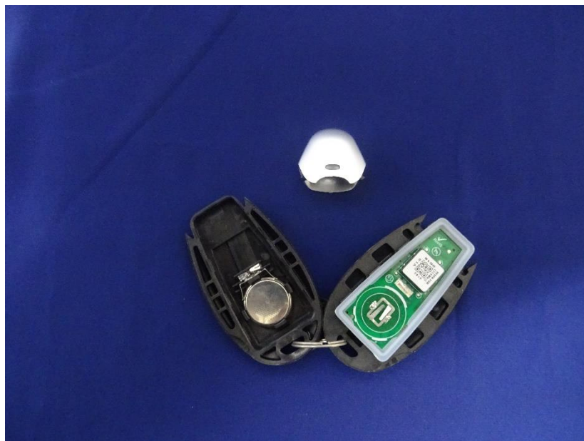
PCB With Encloser
