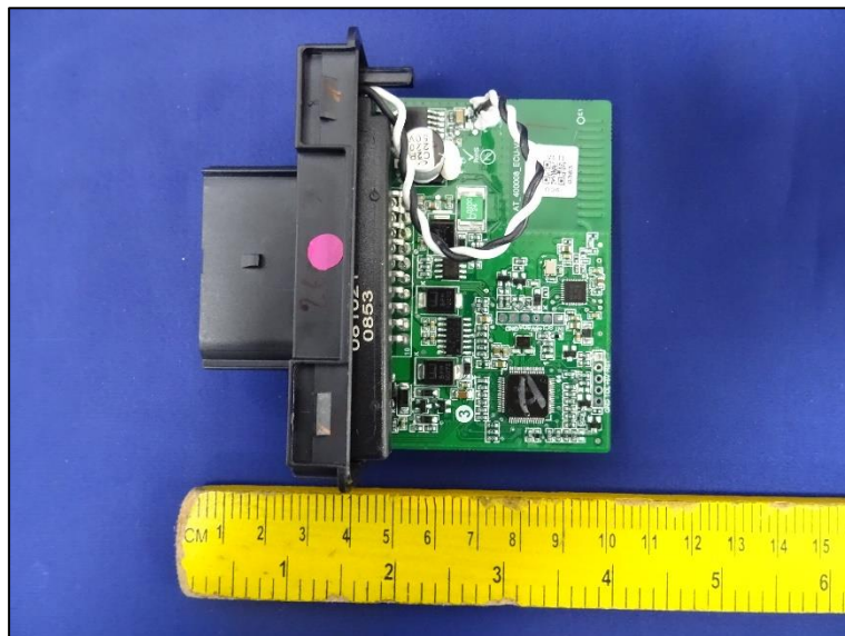
PCB Dimensional View
