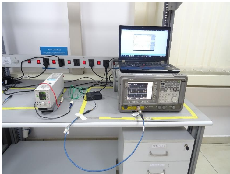
Conducted Test Setup Photo
