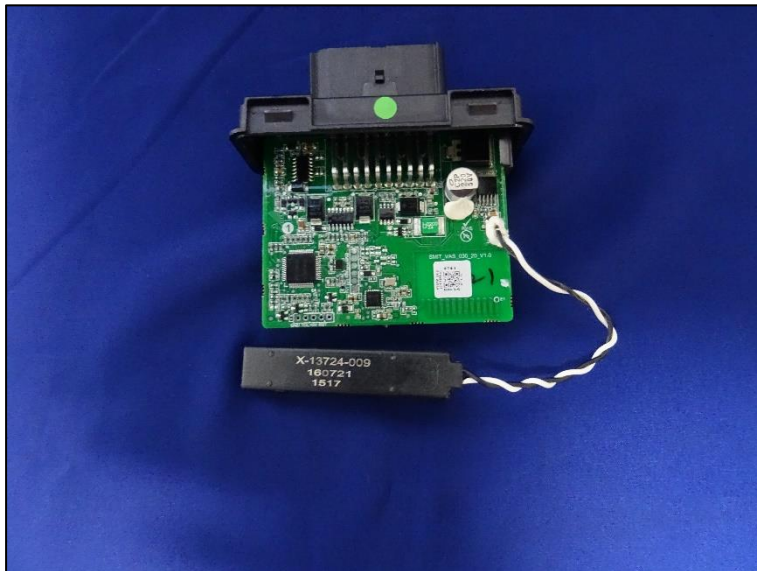
PCB With Antenna
