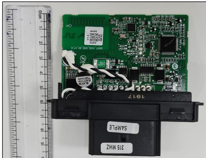
PCB Dimensional View
